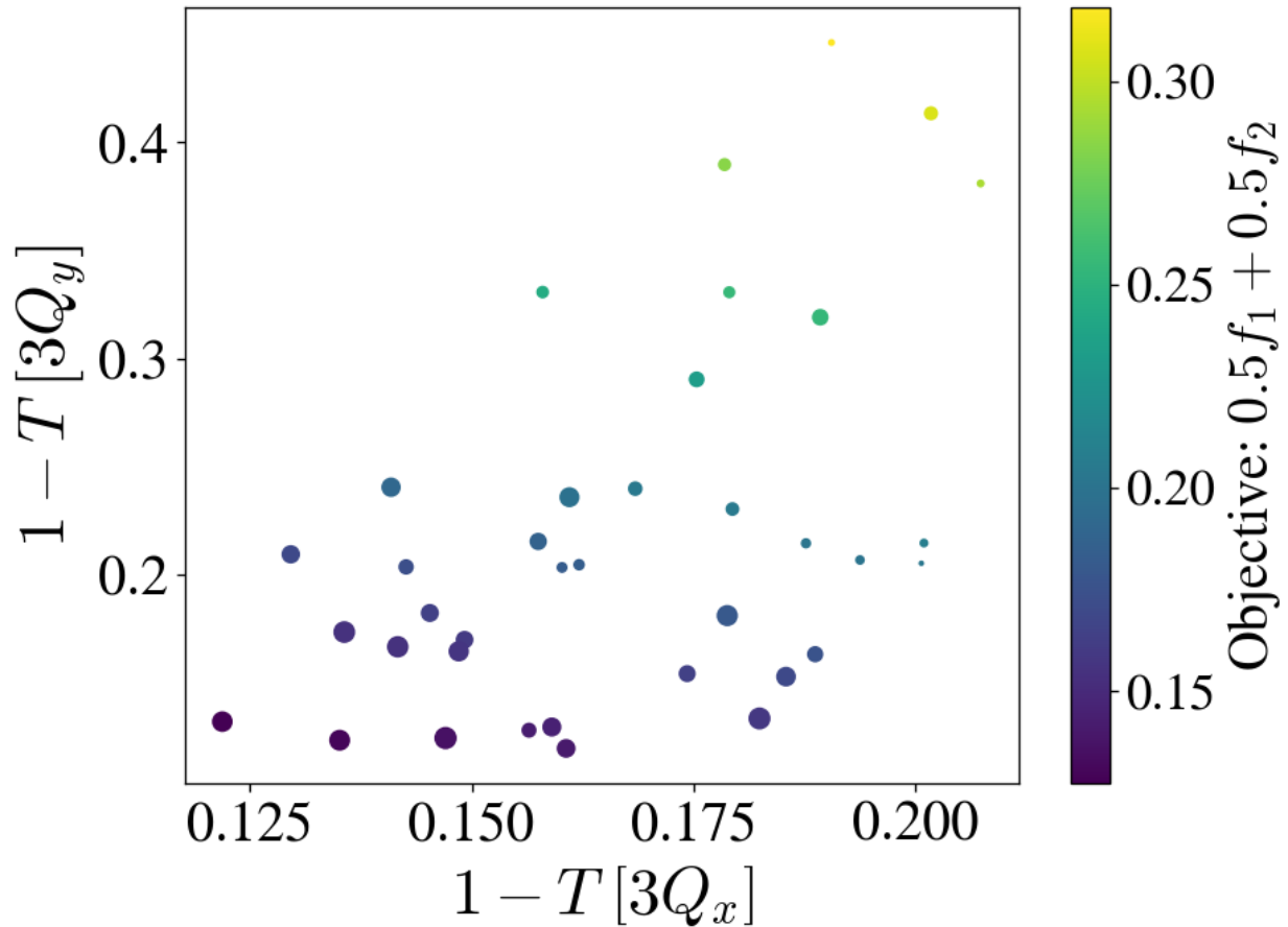
Figure 4.19 Multiobjective Nelder-Mead optimization of the transmission through 3Q_x and 3Q_y . The objective function to be minimized was defined as an equally-weighted sum of both one minus transmissions—corresponding to the fractional losses through the resonance lines.
