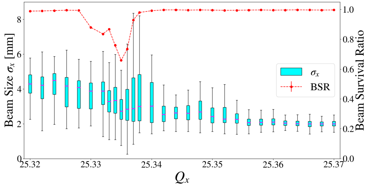
Figure 6.12 Static tune scan with beam survival ratio and IPM data box plots with 3Q_x compensation, transverse dampers ON and 2 Booster Turns of equivalent intensity or approximately 0.5 \times 10^{10} ppb.
