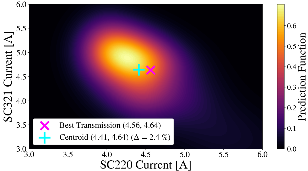
Figure 4.17 Prediction function built from the best R-squared statistics BPMs, in order to predict the best global currents for h_{3000} compensation.
