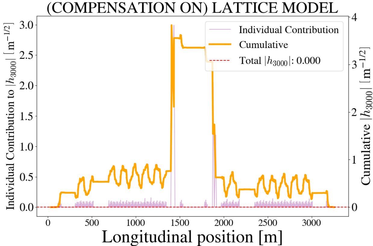
Figure 4.12 Distribution of the h_{3000} term around the ring with individual contributions from each relevant element and the cumulative sum from an arbitrary starting point. This is with existing sextupoles powered at the correct currents to cancel out h_{3000} and h_{1020} simultaneously.
