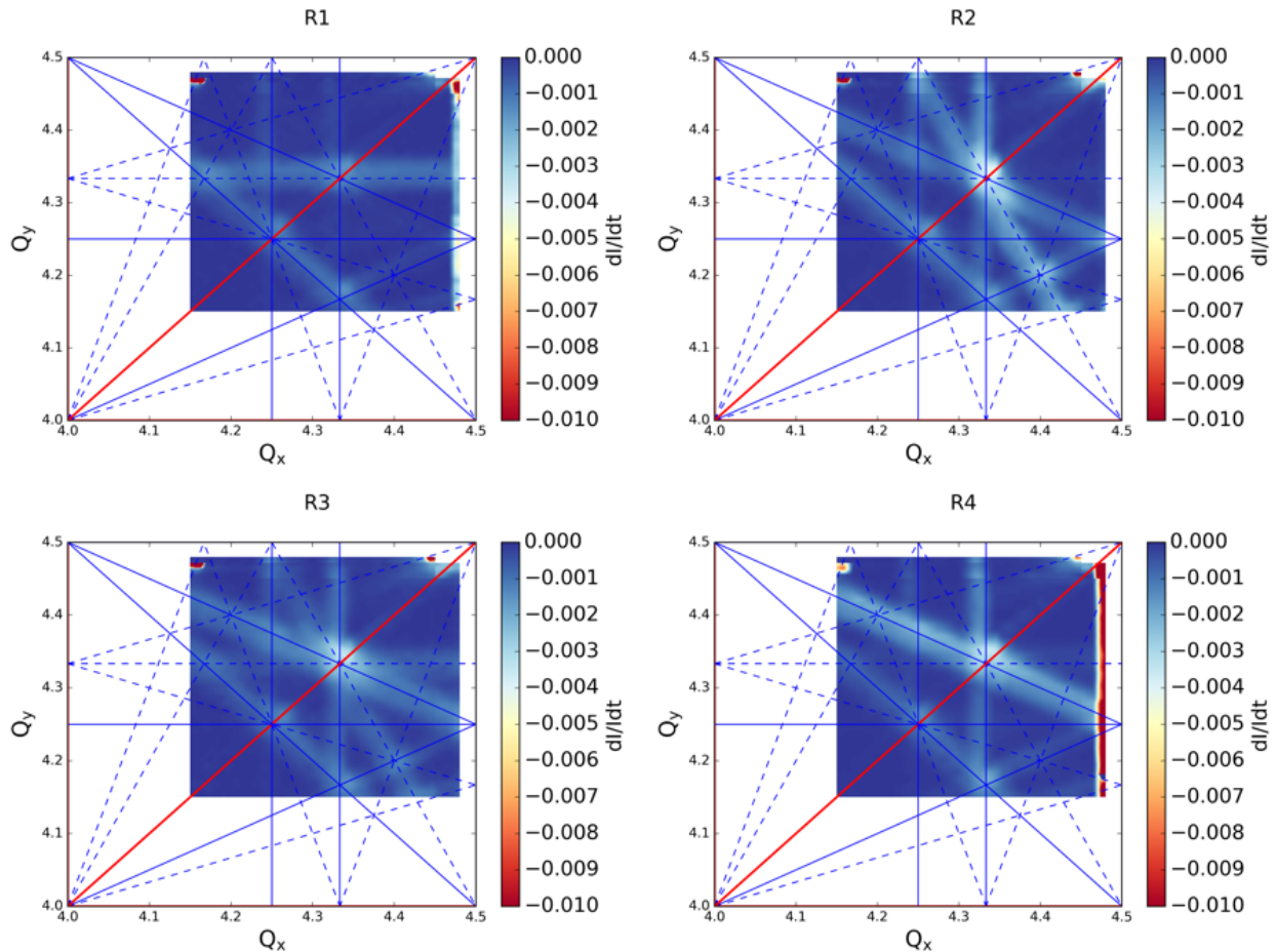
Figure 5.4 Dynamic loss maps for the bare machine of the 4 rings (R1, R2, R3 and R4) in the PS Booster. The plots are an average of scanning in 4 directions. Plot provided by F. Asvesta.
