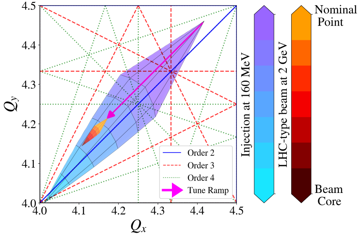
Figure 5.2 Operational tune footprint for PSB beam at injection (cool color map) and footprint after beam has been accelerated to 2 GeV (warm color map). During acceleration, there is a tune ramp illustrated with the fuchsia arrow.
