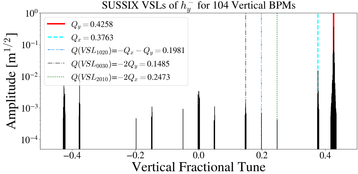
Figure 4.7 Spectral lines of h_y^- calculated with SUSSIX [43]. The h_y^- signal was reconstructed for the 104 Vertical BPMs. The spectrum for all BPMs is superimposed in this plot.
