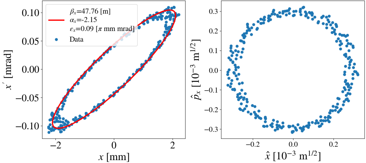
Figure 4.5 Reconstructed phase space data with the best ellipse fit (left plot). The right plot shows the reconstructed normalized phase space from using Eq. 2.13 with the Twiss parameters, as estimated from the ellipse fit. This data corresponds to the horizontal data shown in Fig. 4.4 for the R:HP620 BPM.
