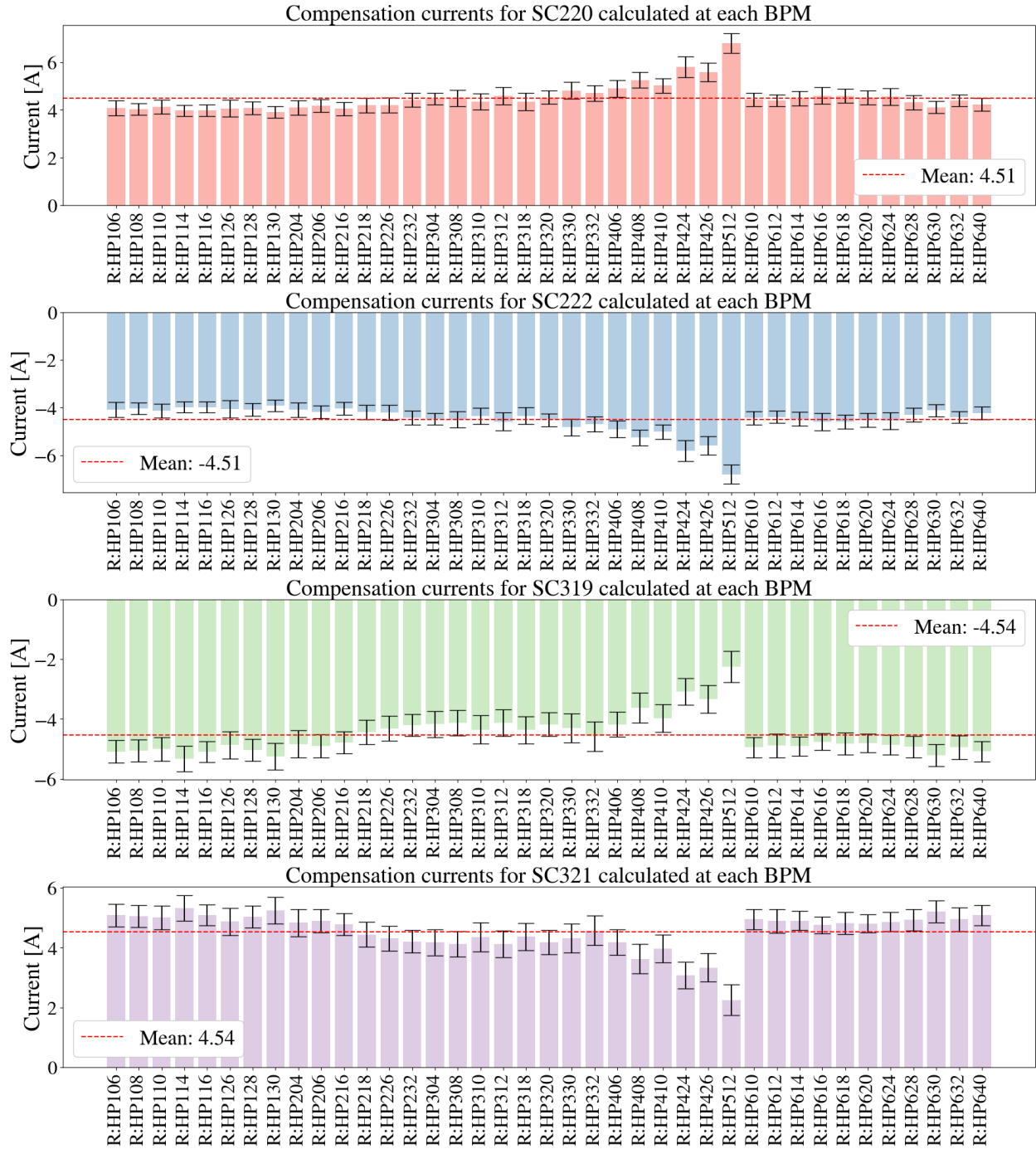
Figure 4.16 Compensation currents calculated from BPMs that showed the best R-square statistic from performing the RDT scans.
