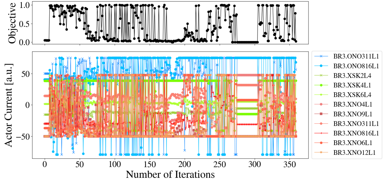
Figure 5.10 Summary for the second instance of Bayesian optimization of resonance compensation applied to Ring 3 in the CERN PSB. This second instance of optimization was trained with the data from the first instance.
