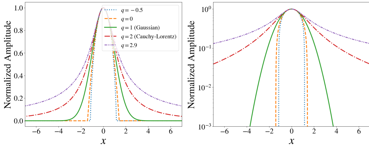
Figure 6.1 Several q -Gaussian distributions for different q parameters normalized to unit amplitude and with a scale parameter of \sigma = 1 .
