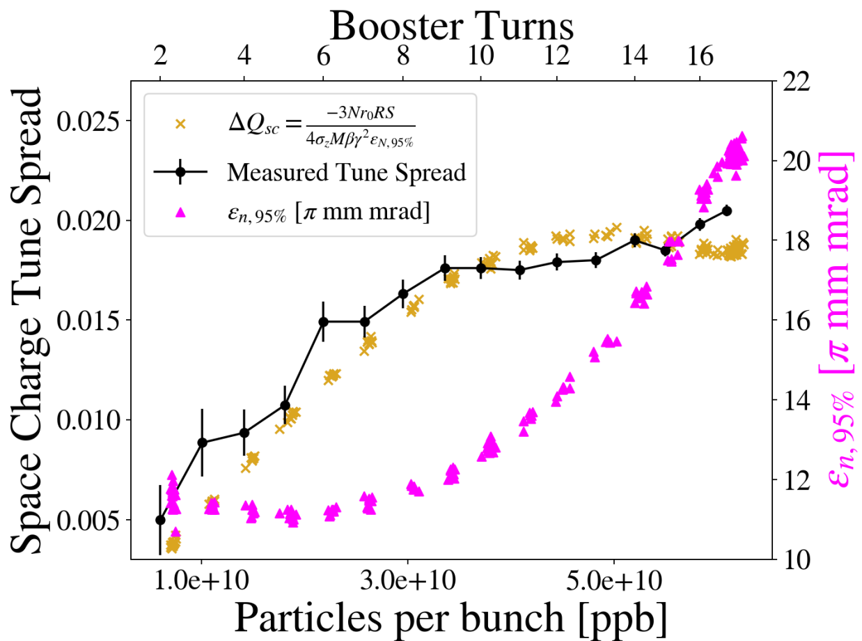
Figure 6.3 Tune spread measurements compared to tune spread calculations from horizontal emittances measured with multiwire data.
