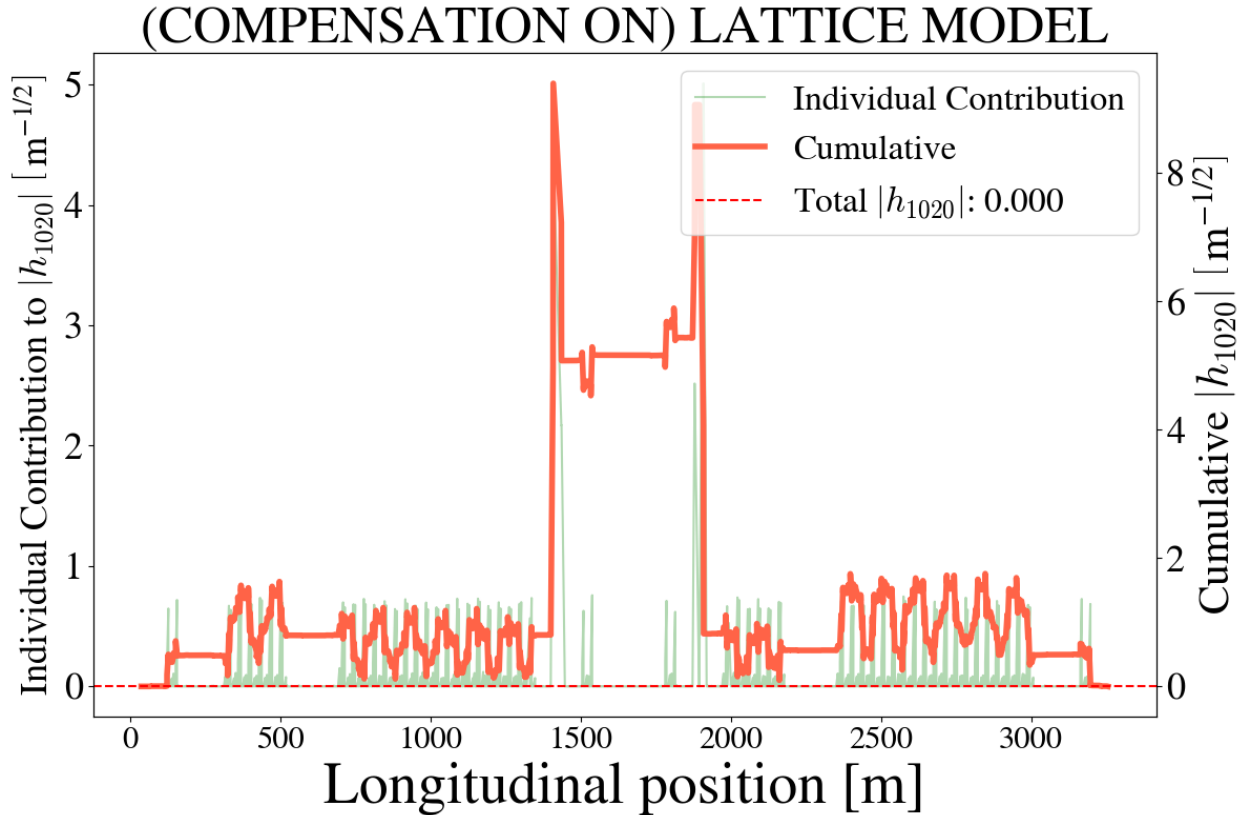
Figure 4.13 Distribution of the h_{1020} term around the ring with individual contributions from each relevant element and the cumulative sum from an arbitrary starting point. This is with existing sextupoles powered at the correct currents to cancel out h_{3000} and h_{1020} simultaneously.
