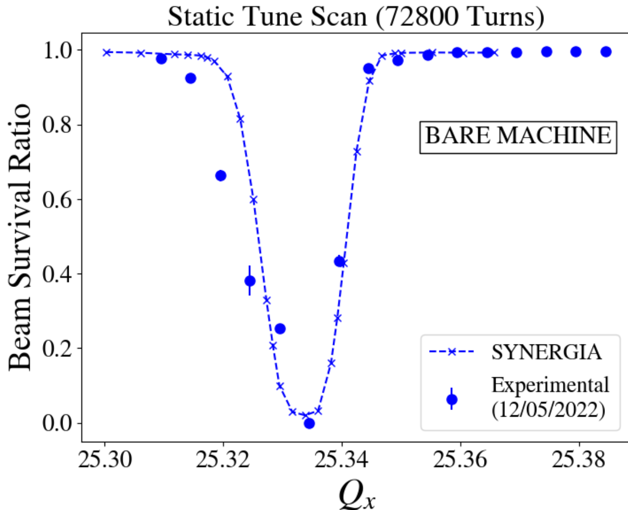
Figure 4.24 Static tune scan for bare machine with comparisons between experimental data and SYNERGIA simulations at a low intensity of 0.5e10 particles per bunch (2 Booster Turns of equivalent intensity).
