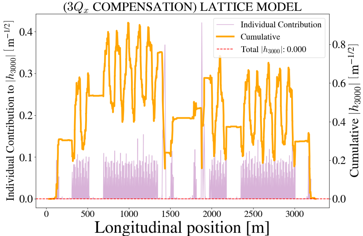
Figure 4.10 Distribution of the h_{3000} term around the ring with individual contributions from each relevant element and the cumulative sum from an arbitrary starting point when correction elements are set to compensate 3Q_x = 76 , i.e., h_{3000} = 0 .
