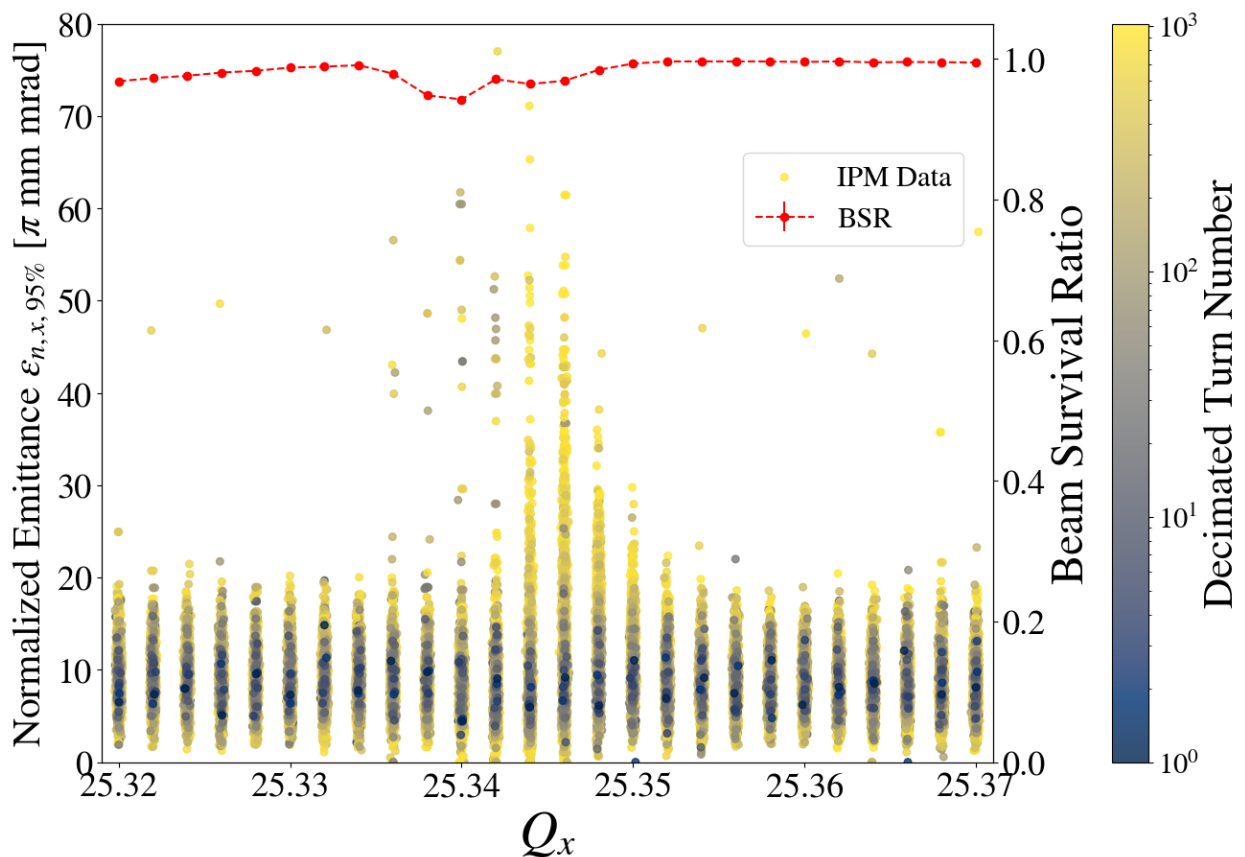
Figure 4.28 Static tune scan with beam survival ratio and emittance data calculated from IPM data for machine with 3Q_x compensation at 2 Booster Turns of equivalent intensity.
