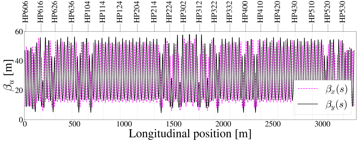
Figure 3.5 Beta functions for the Recycler Ring lattice tuned to Q_x = 25.44 and Q_y = 24.39 . Lattice functions calculated from lattice file using SYNERGIA.
