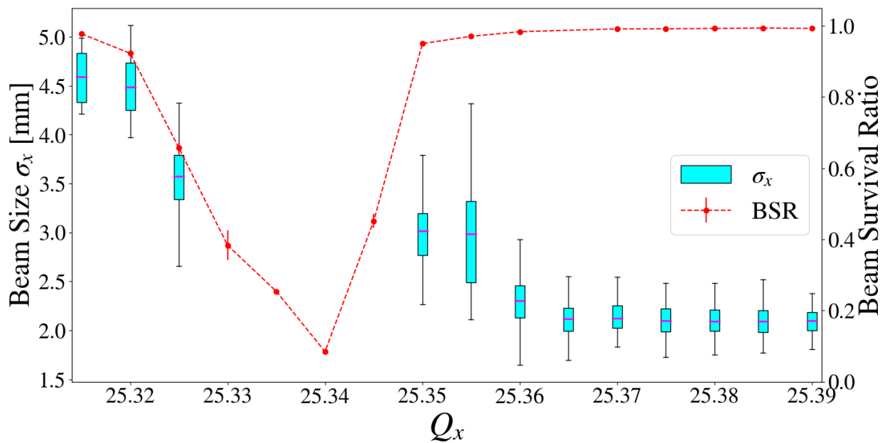
Figure 4.26 Static tune scan with beam survival ratio and IPM data box plots for bare machine at 2 Booster Turns of equivalent intensity.
