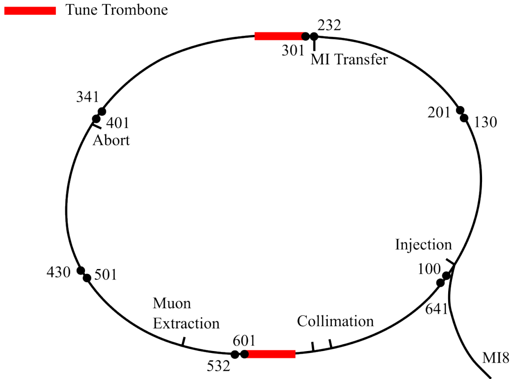
Figure 3.4 Schematic layout of the Recycler Ring and its corresponding sections. Original plot provided by R. Ainsworth, first published on Ref. [14].
