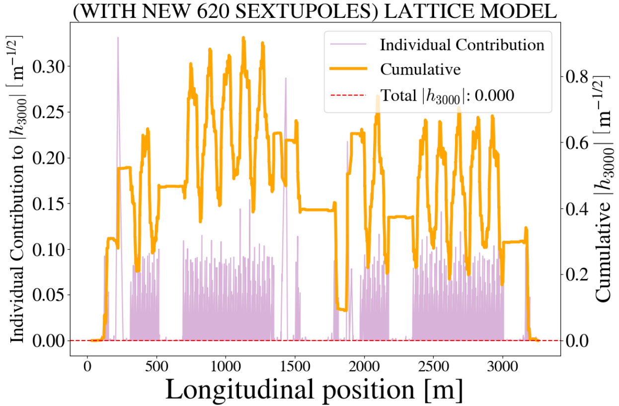
Figure 4.32 Distribution of the h_{3000} term around the ring with individual contributions from each relevant element and the cumulative sum from an arbitrary starting point. This is with the new 620 sextupoles powered at the correct currents to cancel out h_{3000} and h_{1020} simultaneously.
