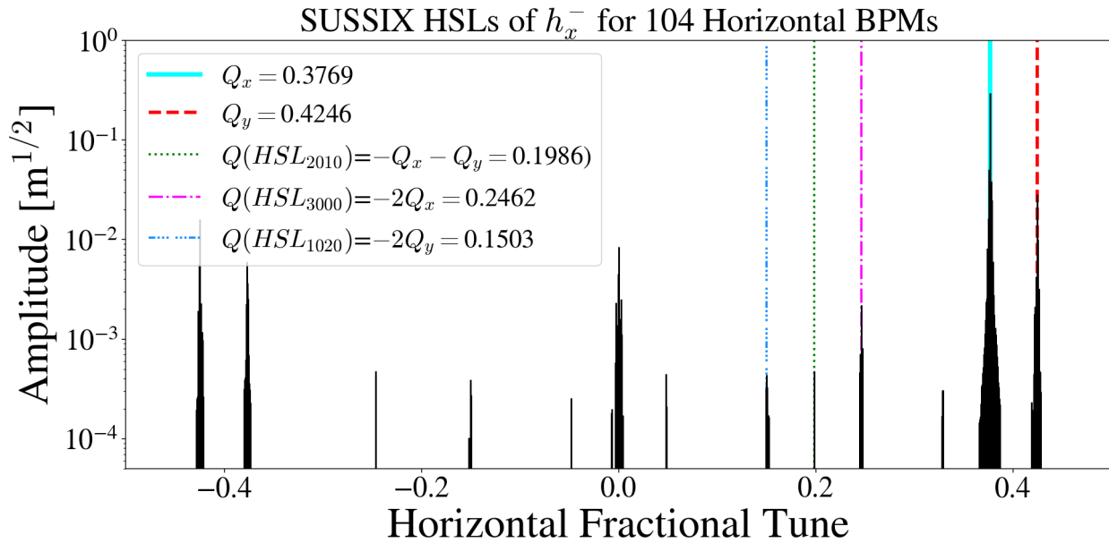
Figure 4.6 Spectral lines of h_x^- calculated with SUSSIX [43]. The h_x^- signal was reconstructed for the 104 Horizontal BPMs. The spectrum for all BPMs is superimposed in this plot.
