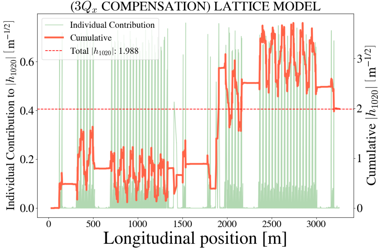
Figure 4.11 Distribution of the h_{1020} term around the ring with individual contributions from each relevant element and the cumulative sum from an arbitrary starting point when correction elements are set to compensate 3Q_x = 76 , i.e., h_{3000} = 0 .
