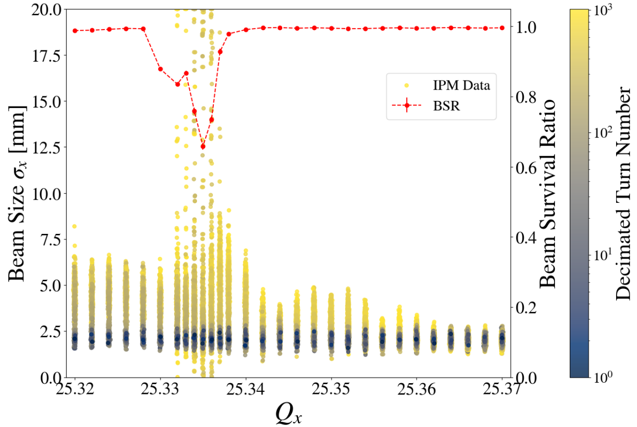
Figure 6.14 Static tune scan with beam survival ratio and IPM data scatter plots with 3Q_x compensation, transverse dampers ON and 2 Booster Turns of equivalent intensity or approximately 0.5 \times 10^{10} ppb.
