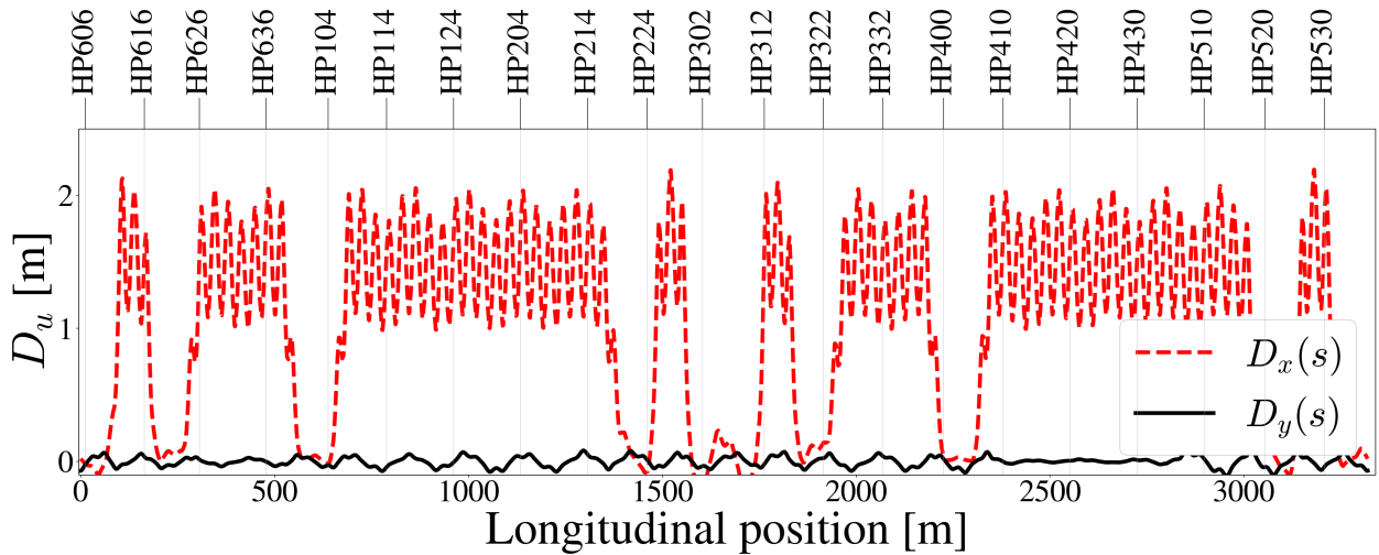
Figure 3.6 Dispersion functions for the Recycler Ring lattice tuned to Q_x = 25.44 and Q_y = 24.39 . Lattice functions calculated from lattice file using SYNERGIA.
