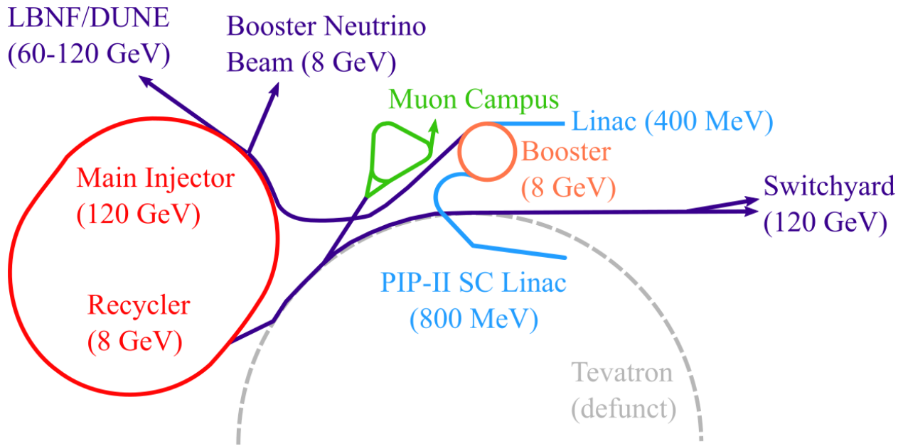
Figure 3.2 Future layout of the Fermilab Accelerator Complex for the Proton Improvement Plan II (PIP-II). Original plot provided by R. Ainsworth, first published on Ref. [14], but modified for this document.
