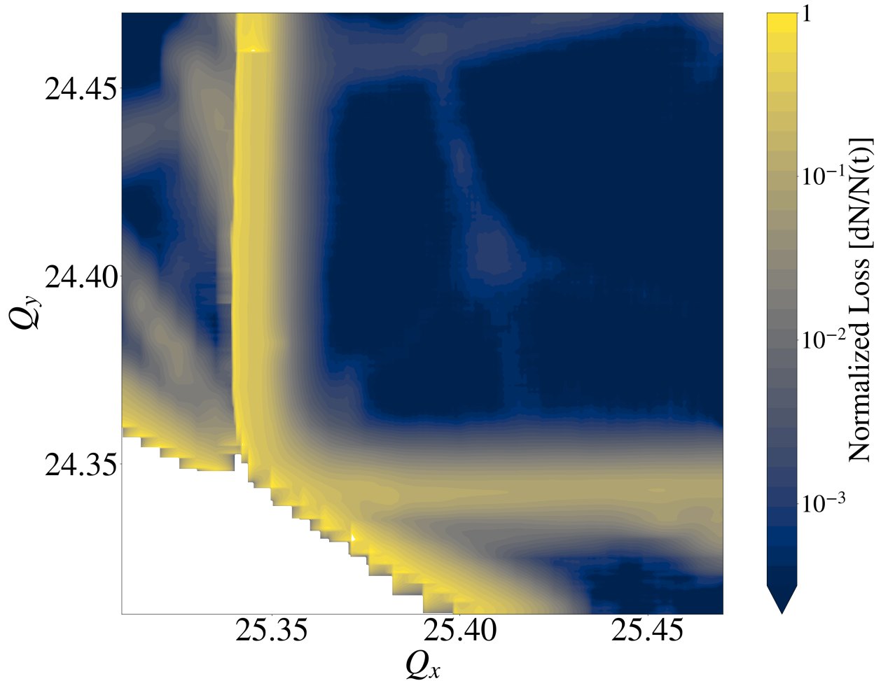
Figure 4.21 Dynamic loss map from ramping the tunes with an interval of \Delta Q_u = 0.005 in both directions. The directions of scan are from left to right and top to bottom. The results are superimposed in this plot.
