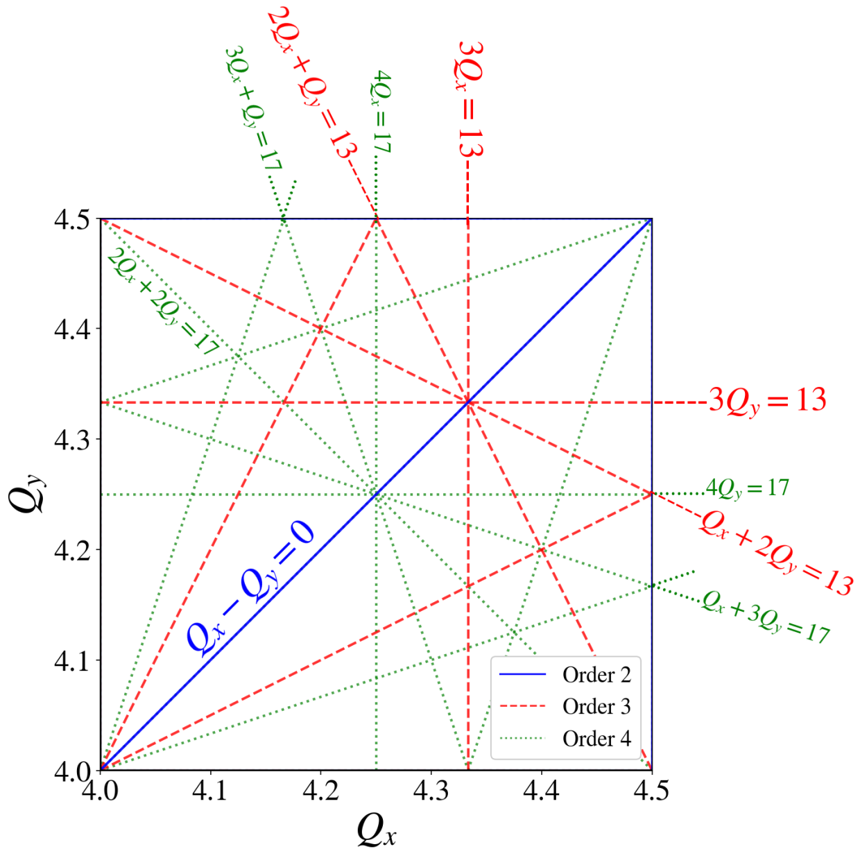
Figure 5.3 Portion of the tune diagram enclosing the operational tunes of the PS Booster with relevant resonance lines labelled.
