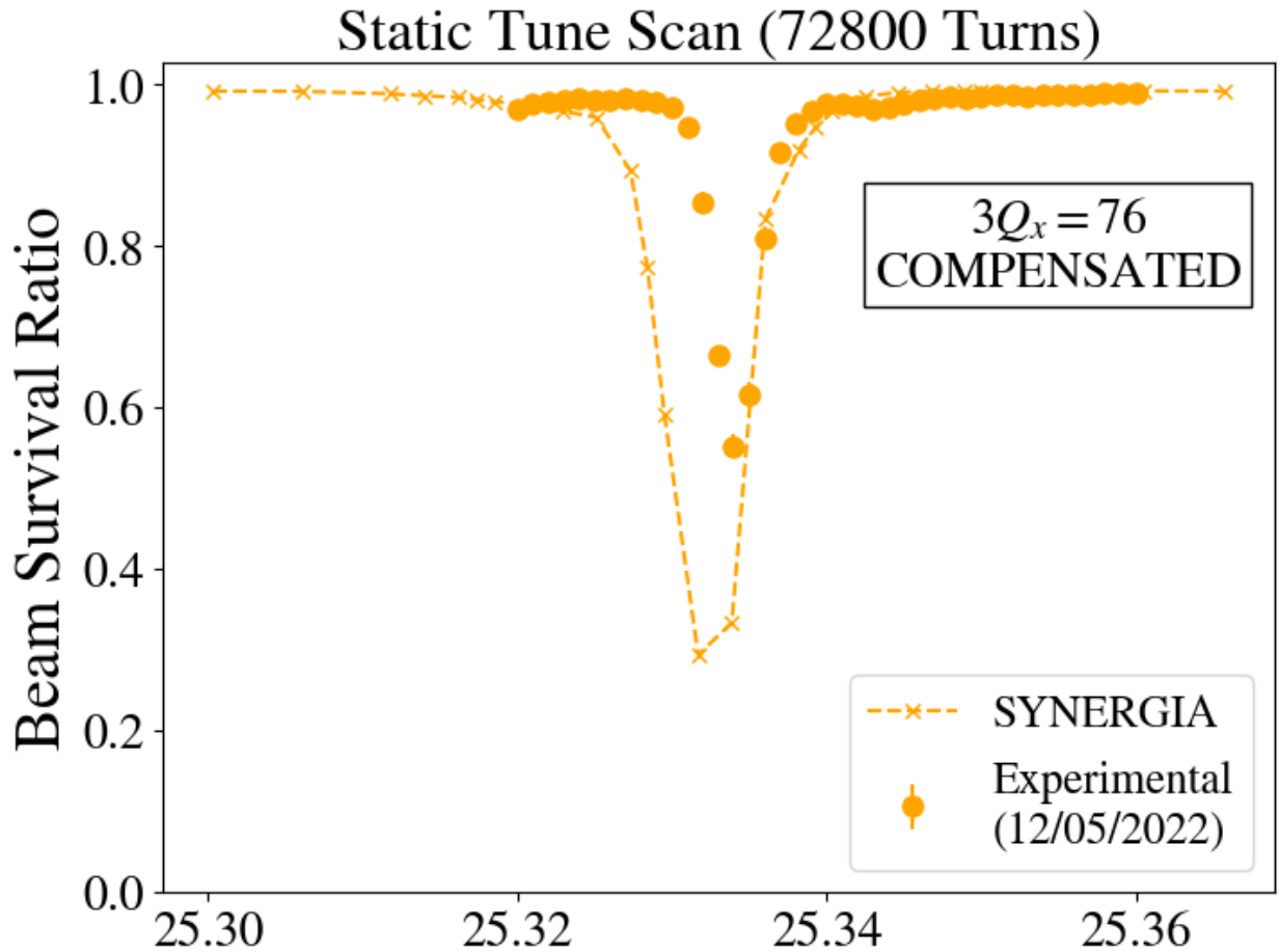
Figure 4.25 Plot for static tune scan for machine with 3Q_x compensation including comparison between experimental data and SYNERGIA simulations.
