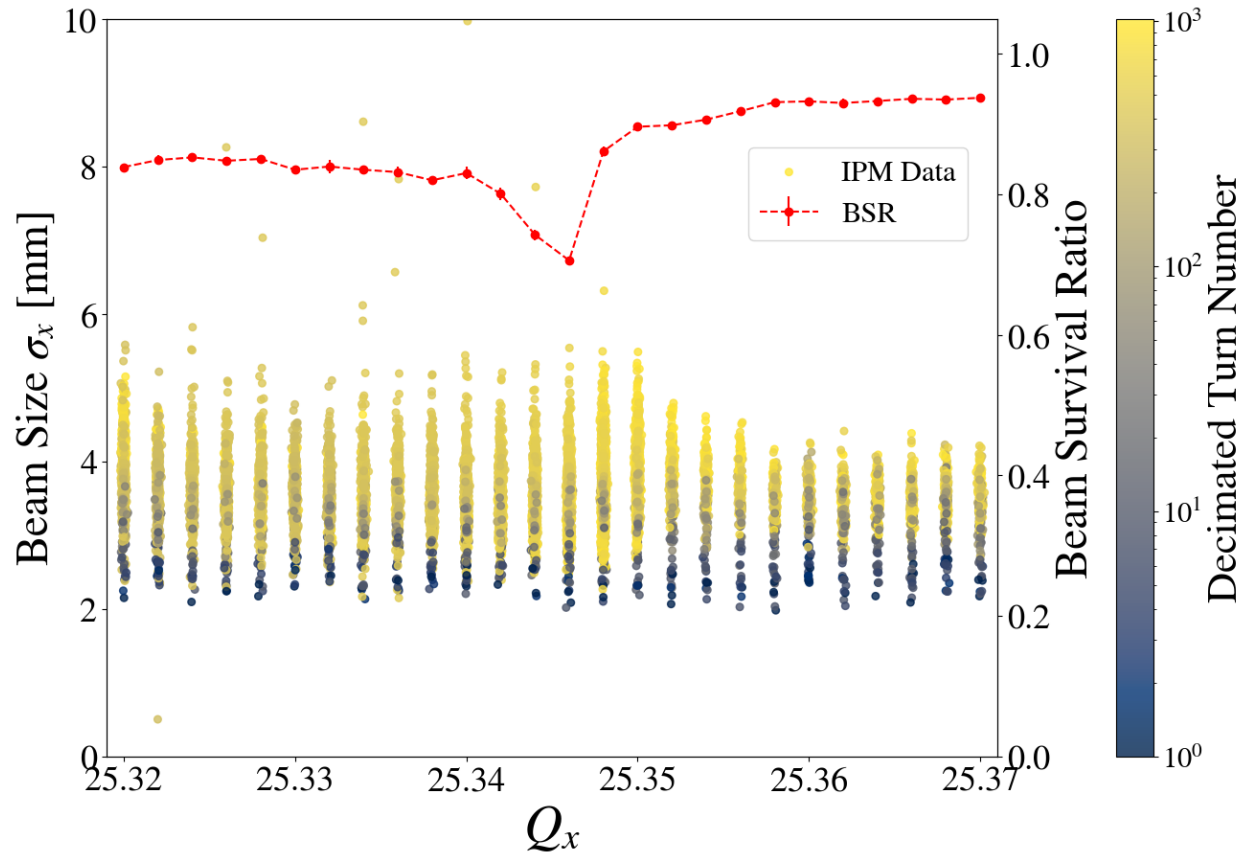
Figure 6.6 Static tune scan at an equivalent intensity of 8 Booster turns or approximately 3 \times 10^{10} ppb.
