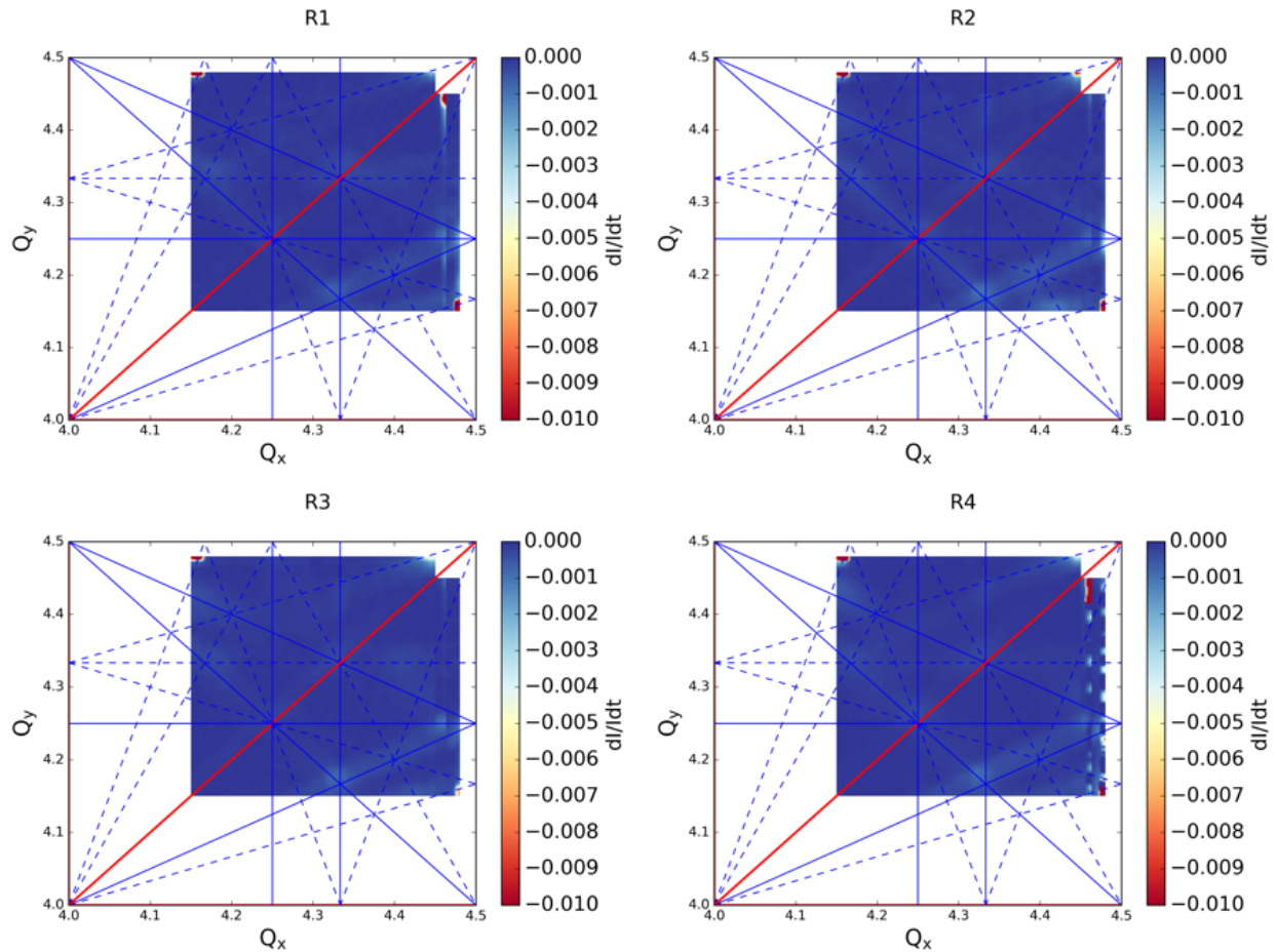
Figure 5.13 Dynamic loss maps for the 4 rings in the PS Booster with the best configuration from the Bayesian optimization of the resonance compensation. The plots are an average of scanning in 4 directions. Plot provided by F. Asvesta.
