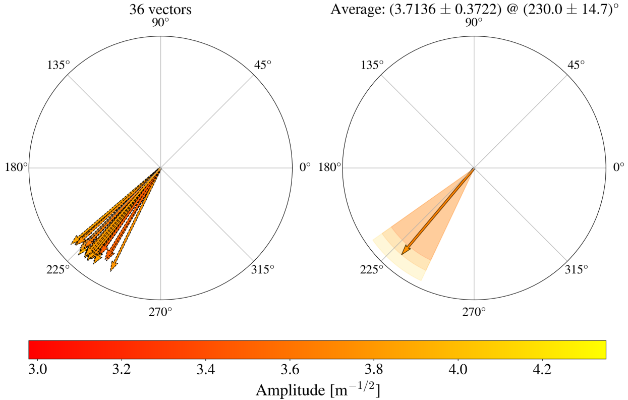
Figure 4.8 Polar plot for the measurement of h_{3000} for 36 measurements at horizontal BPM R:HP620.
