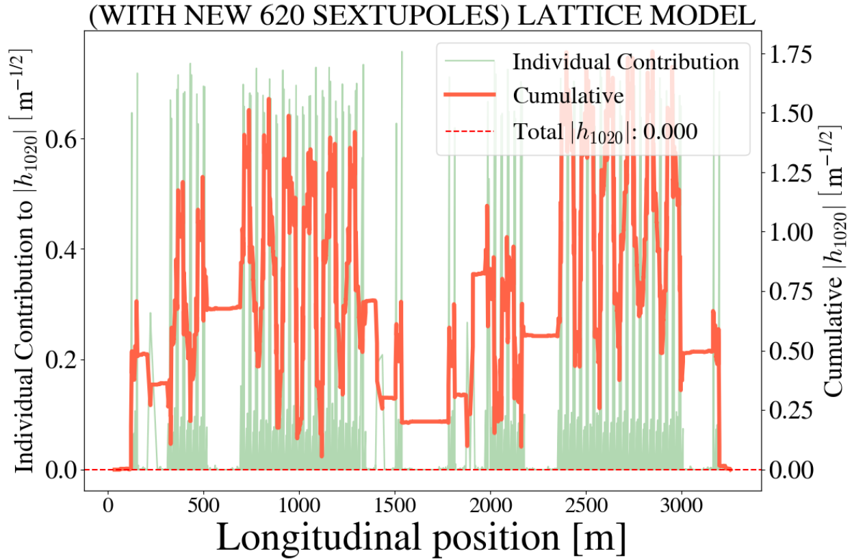
Figure 4.33 Distribution of the h_{1020} term around the ring with individual contributions from each relevant element and the cumulative sum from an arbitrary starting point. This is with the new 620 sextupoles powered at the correct currents to cancel out h_{3000} and h_{1020} simultaneously.
