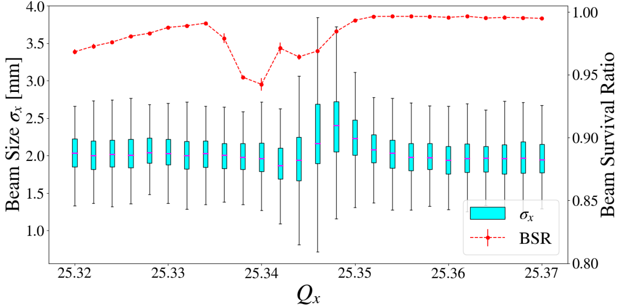
Figure 4.27 Static tune scan with beam survival ratio and IPM data box plots for machine with 3Q_x compensation at 2 Booster Turns of equivalent intensity.
