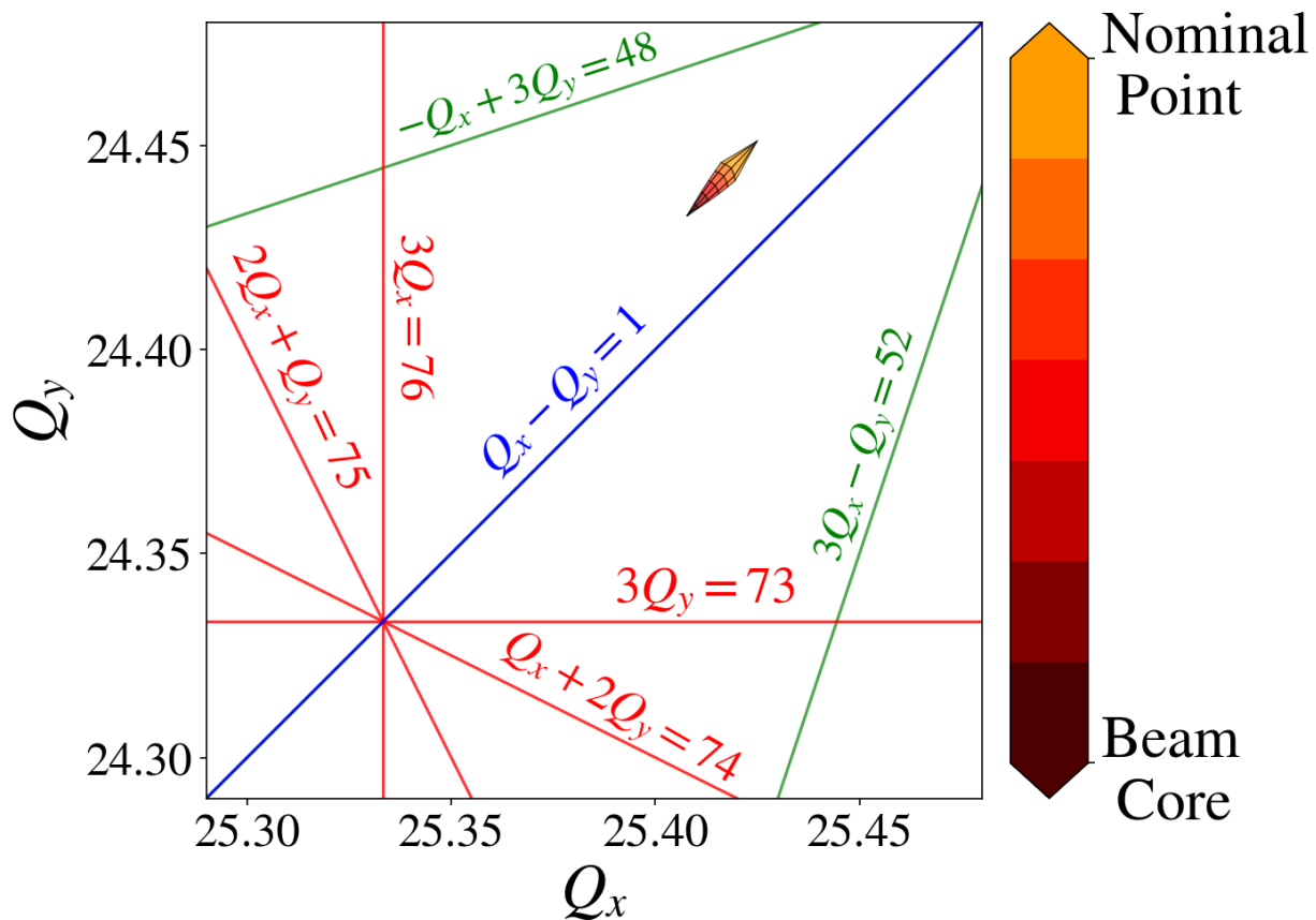
Figure 2.4 Approximate operational tune footprint at low intensities calculated with PySCRDT [24], i.e., 1e10 particles per bunch.
