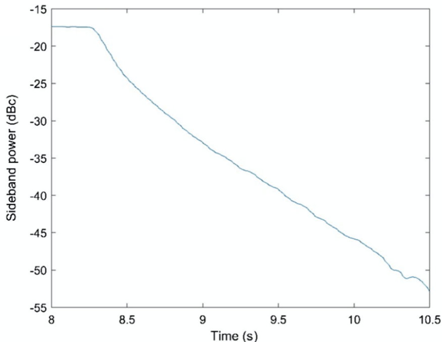
Figure 4.8: The decay curve measured at 95 Hz. The decay rate of the mechanical mode energy is -14 dB=s. [77]
