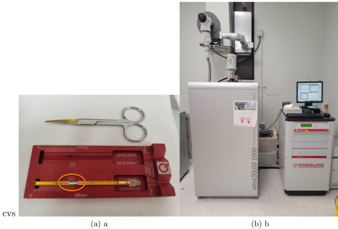
Figure 6.5: (a) PPMS insert device with niobium sample mounted (circle). (b) PPMS instrument used at FNAL.
