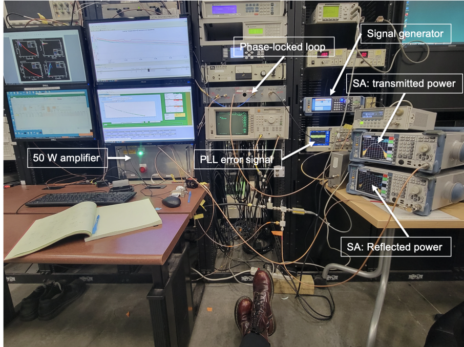
Figure 2.5: Vertical testing RF instrumentation at MSU/FRIB
