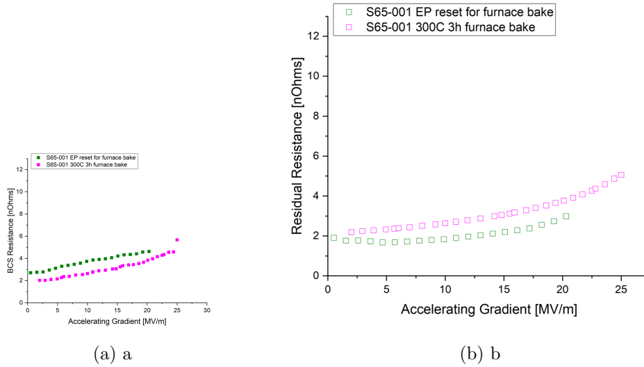
Figure 5.11: Deconvolution of R_0 and R_{BCS} for the furnace-baking EP baseline trial (green) and the 3 h, 300°C furnace baking trial (magenta). While no major gains in Q_0 performance were seen, the different becomes apparent here: furnace baking decreased R_{BCS} and increased R_0 compared to the EP baseline. Fractionally, this tradeoff was quite balanced, so the furnace baking effect was masked in the Q_0 v E_{acc} representation.
