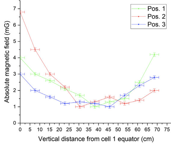
Figure 4.17: Background magnetic field in the vertical test dewar. The fields were measured by lowering fluxgate magnetostatic sensors in increments to create a vertical scan at three different azimuthal locations, spaced evenly 120^\circ around the edge of the dewar. The sensor locations were offset from the center axis by the same distance as the cavity equator. These were measured with the cavity installed in the dewar together with the dewar lid; however, this measurement could only be conducted at room temperature, not at 2K.
