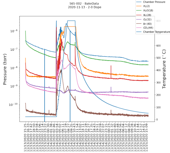
Figure 5.2: Time series gas pressure and temperature profile of the first 2/0 N-doping procedure conducted on S65-002 at FNAL. If the dataset can be recovered from the furnace, this will be updated.
