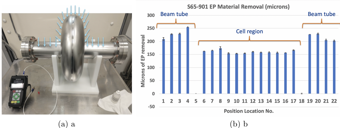
Figure 4.11: (a) Image of the prototype FRIB 644 MHz \beta opt = 0.65 single cell cavity, with blue arrows indicating the 20 used ultrasonic thickness measurement locations across the cavity surface. (b) Microns ( \mu\text{m} ) of removal, with measurement error, showing an average removal in the cell region of 160 m with a standard deviation of approximately 6 \mu\text{m} . No significant deviation exists between the material removal from the near-vertical sidewalls (positions 6-10, 13-17) and the cavity equator (position 11-12). Positions 5 and 18 encroached upon the high-curvature region near the cavity iris and the ultrasonic thickness measurement tool could not produce accurate readings.
