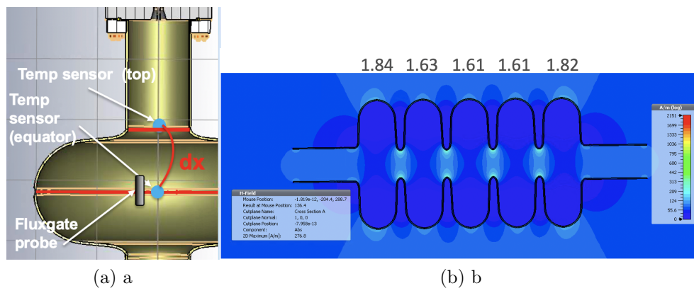
Figure 6.2: (a) Diagram of the experimental setup with the positions of the fluxgate magnetic probe, and two Cernox temperature sensors highlighted. (b) CST Microwave Studio simulation of idealized flux expulsion in a 5-cell FRIB400. cavity.
