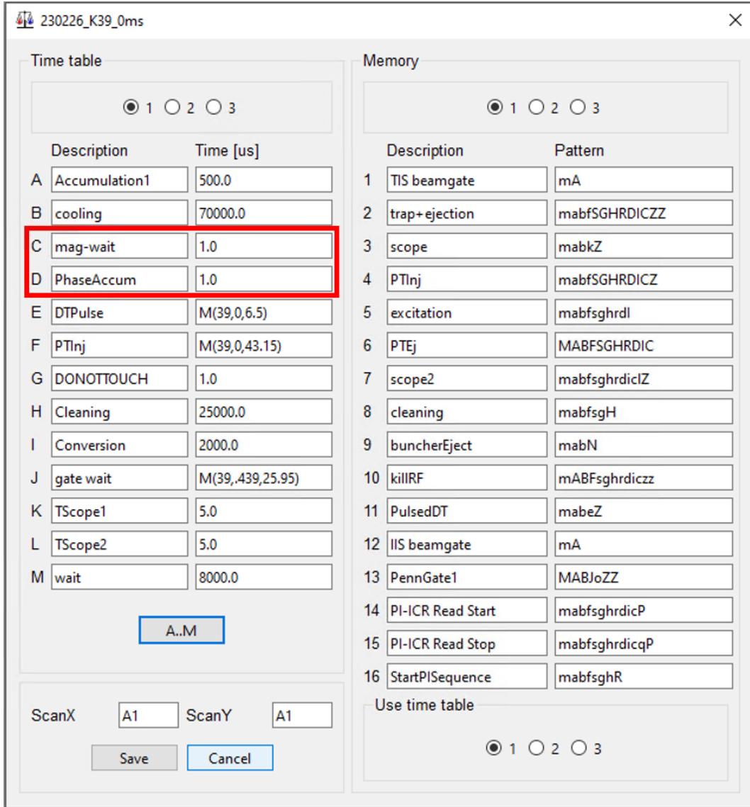
Figure B.3: The Timing panel. Red box added to this figure to show the two values which must regularly be manually changed. Mag-wait is t_{acc-} and PhaseAccum is t_{acc+} , as referenced in Figures 2.9 and 2.10 respectively.
