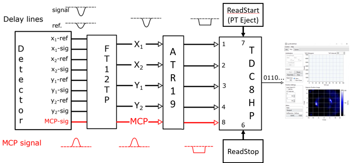
Figure A.1: Diagram showing the flow of signals from detector to computer. Adapted from [43]
