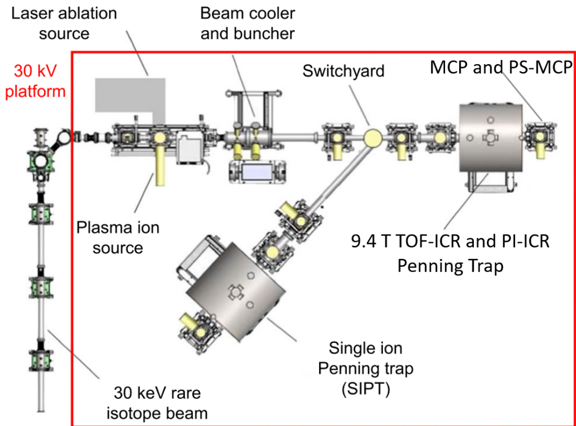
Figure 3.1: Layout of the Low Energy Beam and Ion Trapping (LEBIT) facility. Adapted from [25]
