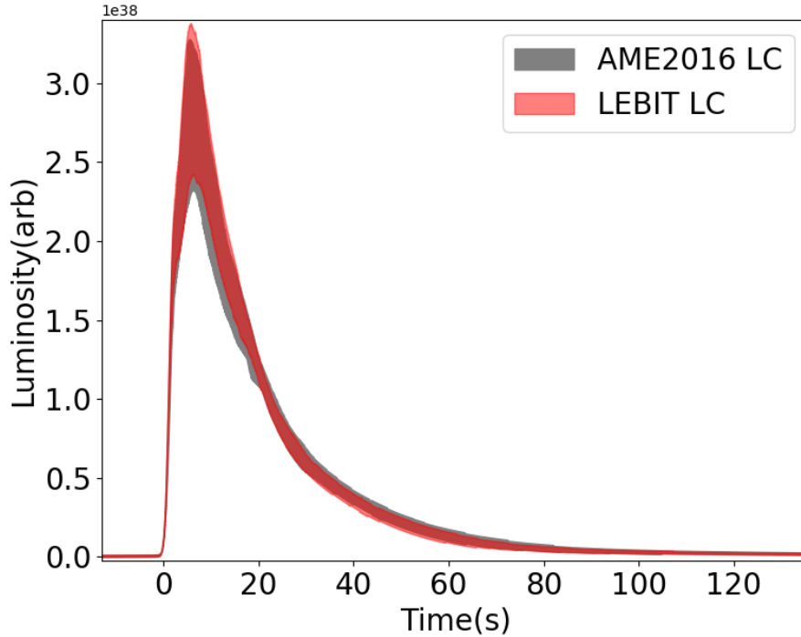
Figure 4.7: MESA multizone XRB light curve generated using the mass of ^{27}\text{P} from LEBIT (red) and AME2016, each varied \pm 3\sigma . The burster is "GS 1826-24"-like, with accretion rate decreased from 2.98 \times 10^{-9} to 1.23 \times 10^{-9} msol/yr in order to enhance ^{27}\text{P} 's impact.
