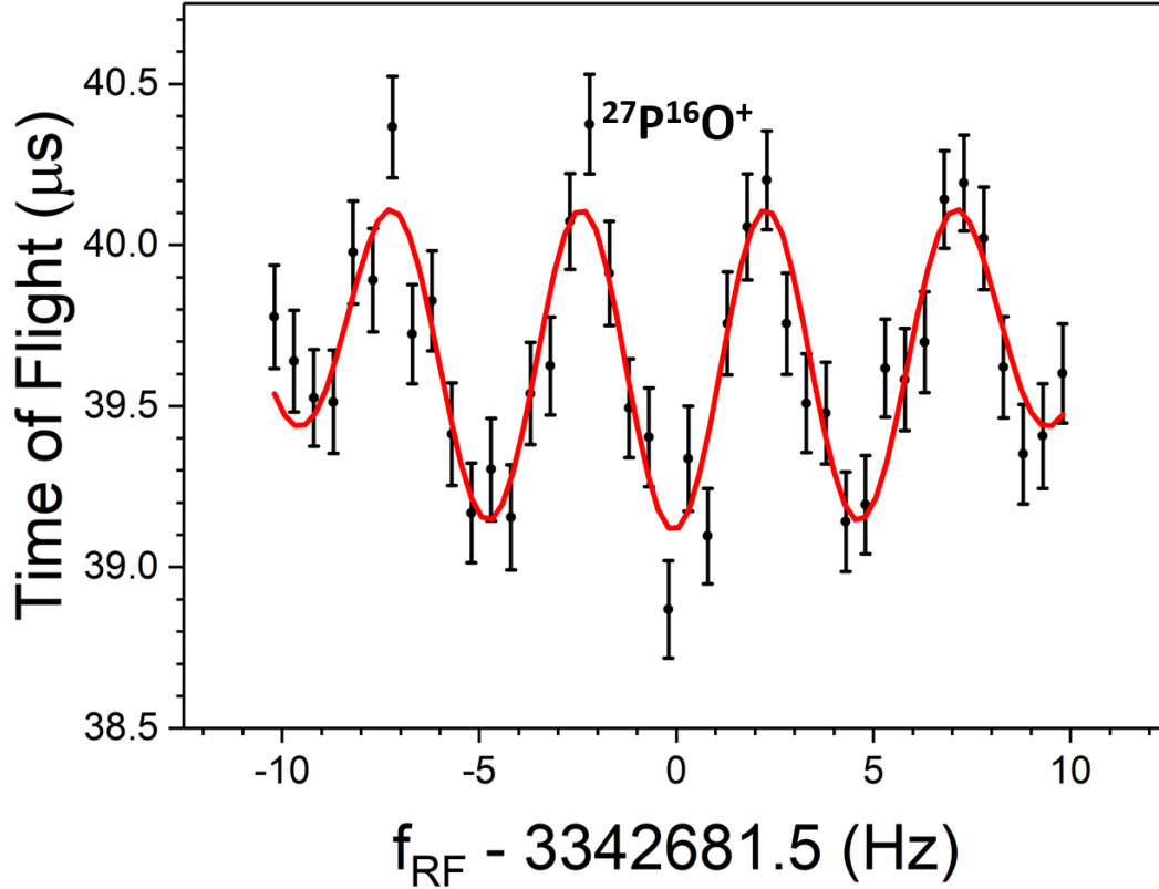
Figure 4.2: A sample ^{27}\text{P}^{16}\text{O}^+ time-of-flight ion cyclotron Ramsey resonance measurement. The central dip in the interference pattern corresponds to the resonant cyclotron frequency. The red curve is a fit to the theoretical profile [29].
