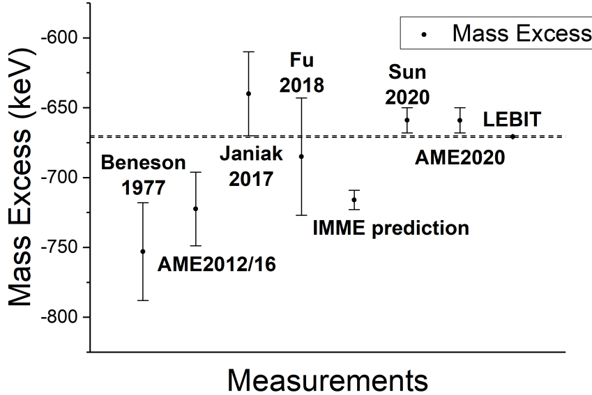
Figure 4.4: Past measurements and predictions of ^{27}\text{P} 's mass compared to the LEBIT result (dotted line). [65]
