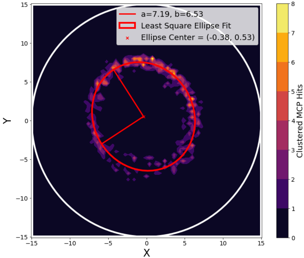
Figure 2.7: Elliptical projection of the circular path ions in the Penning trap follow. An ellipse is fit to the position data using the techniques in [44], and the center of this fit—in this case (-0.38, 0.53) —is used as the origin which all phases in PI-ICR calculations are taken with respect to. "a" and "b" are the radii of the major and minor axes, respectively.
