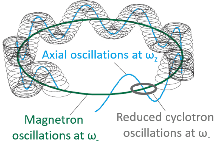
Figure 2.2: Ion motion in a Penning trap split into its three component motions
