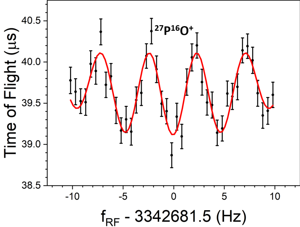
Figure 2.5: Sample 250 ms Ramsey resonance of ^{27}\text{P}^{16}\text{O}^+ . Instead of a continuous 250 ms excitation, an excitation scheme of 50 ms RF, 150 ms free evolution, 50 ms RF was applied to generate the above interference pattern. The above theoretical fit (red), and fits for other complex schemes are described in [29]. The central ToF minimum corresponds to the cyclotron frequency f_c .
