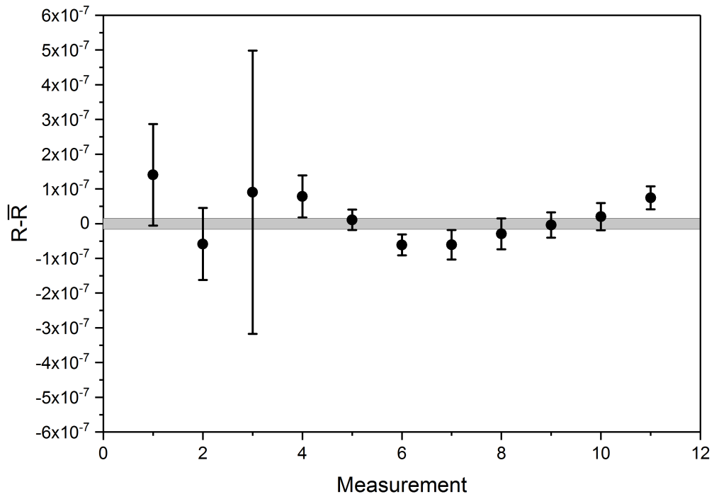
Figure 4.3: Measured cyclotron frequency ratios R = \frac{f_{ref}^{int}(HCNO^+)}{f_c(^{27}P^{16}O^+)} relative to the average value \bar{R} = 1.000270250(16) . The gray bar represents \pm 1\sigma uncertainty in \bar{R} and has been scaled by the Birge Ratio of 1.23 [5].
