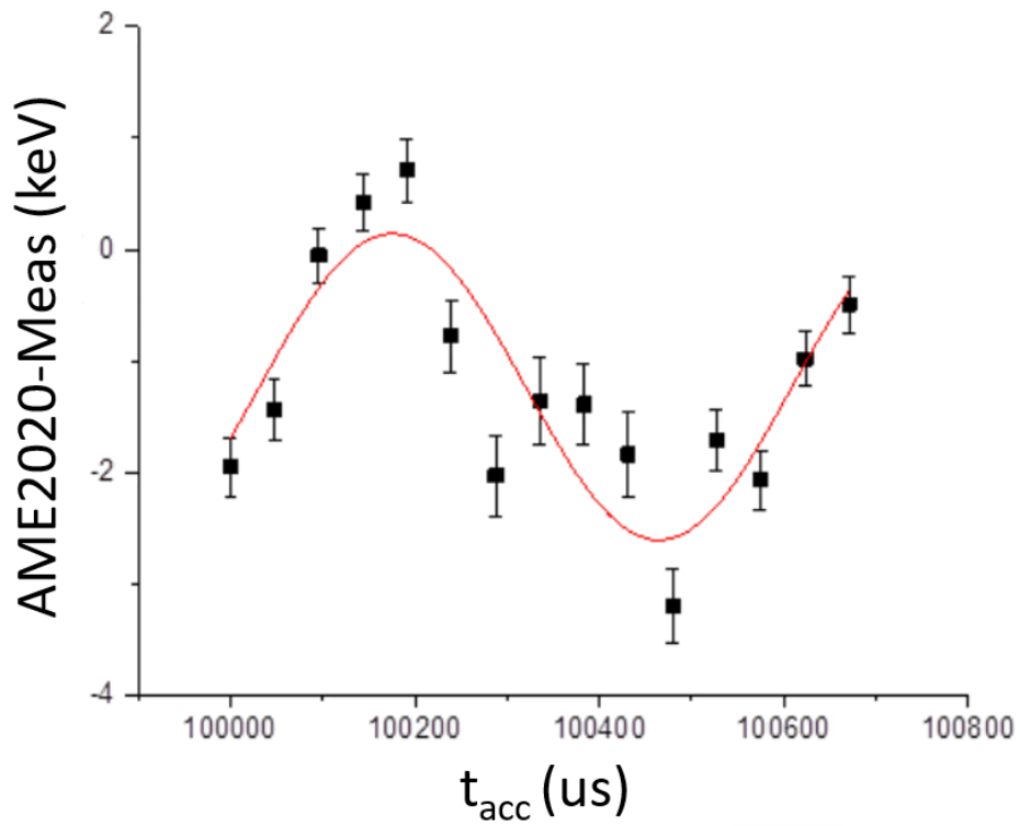
Figure 5.9: Mass measurements made with intentional off-center injection into the penning trap. Measurements were made over a series of 15 accumulation times spanning 700 us, just over one reduced cyclotron period T_- = 535 us.
