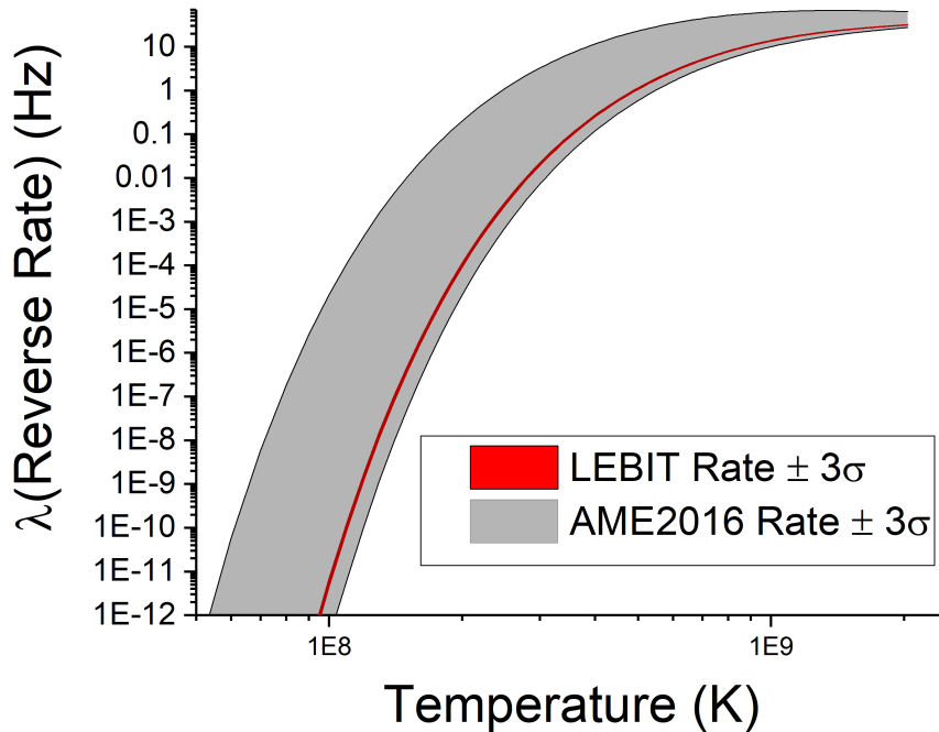
Figure 4.6: Reverse proton capture rate of ^{26}\text{Si} varied by uncertainty in the mass of ^{27}\text{P} . AME2016 is used for comparison in order to more readily compare to Schatz and Ong’s sensitivity study [57]
