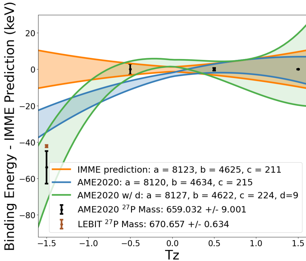
Figure 4.5: Isobaric Multiplet Mass Equation prediction of the binding energy of the A = 27 , T = 3/2 quartet. IMME's form is BE = a + bT_z + cT_z^2(+dT_z^3) . A d-coefficient is required for a good fit (green).
