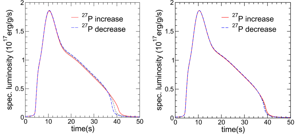
Figure 4.1: Single-zone 1-D type-I XRB light curve model using AME2016’s mass (left) vs the IMME predicted mass (right) for ^{27}\text{P} . The XRB simulation has been re-run with the only changes being the mass of ^{27}\text{P} increased by 3\sigma (red), or decreased by 3\sigma (blue). 3\sigma = 21 keV (left), 79 keV (right)
