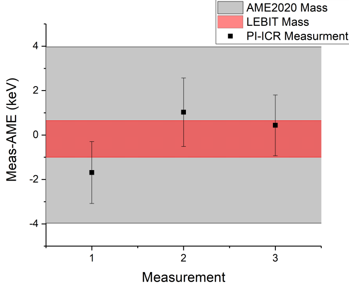
Figure 5.10: The difference between the AME2020 and LEBIT measured mass excess of ^{105}\text{Sn} . LEBIT value -73338.144 \pm 0.825 in red, AME2020 value -73338.001 \pm 3.971 in grey. The error bars of the LEBIT data have been inflated by the Birge ratio [5] value of 1.221 to account for a greater than statistically expected fluctuation in measurements.
