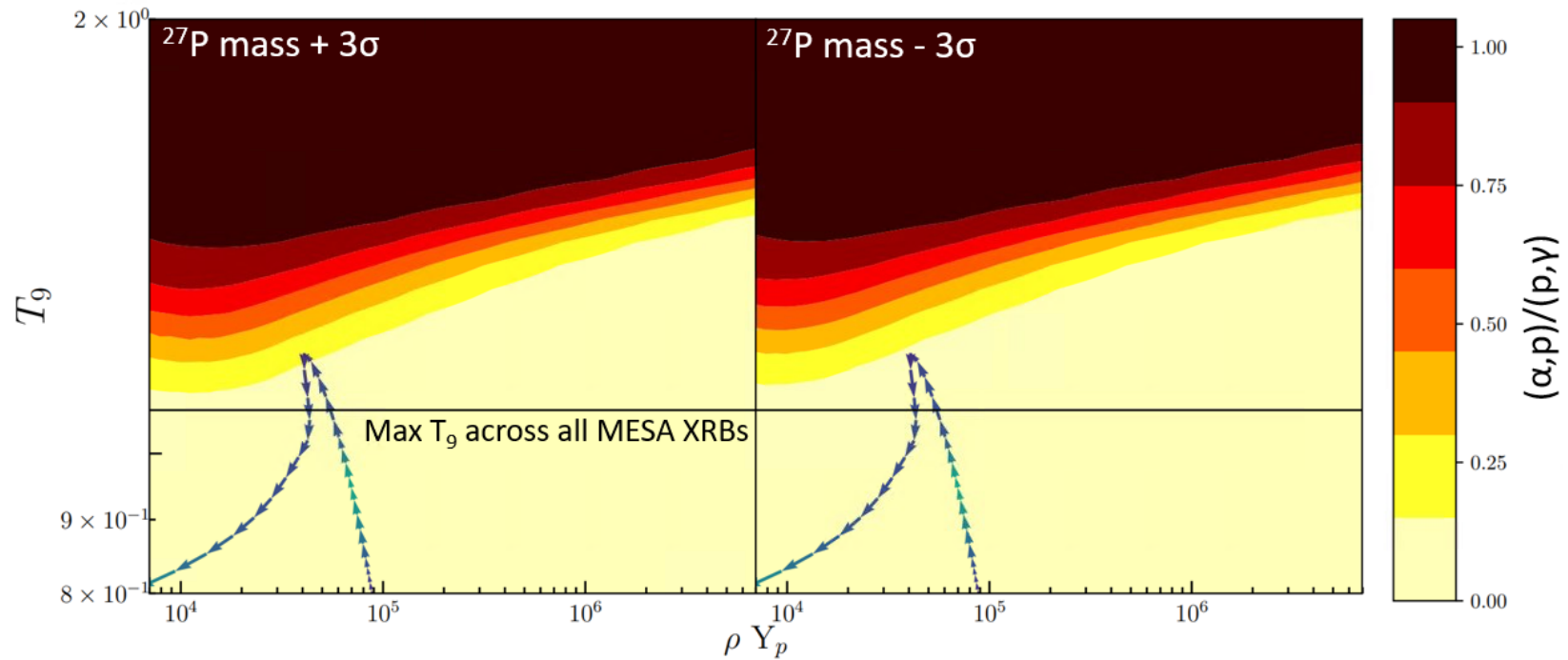
Figure 4.8: Contour plots of the ratio of paths— (\alpha, p)/(p, \gamma) —taken out of the ^{26}\text{Si} waiting point during a type-I XRB. Contours generated using a ^{27}\text{P} mass value of \text{AME2016} \pm 3\sigma (left: +3\sigma , right : -3\sigma ). AME2016 used to demonstrate why sensitivity study [57] predicted the mass of ^{27}\text{P} to impact the rp process path.
