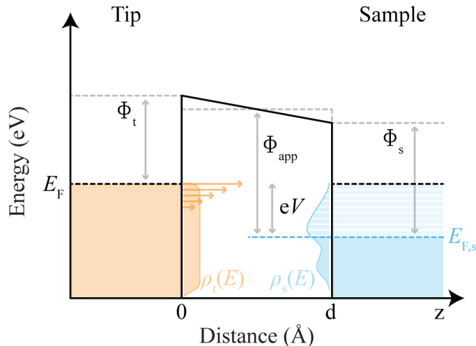
Figure 2.10: Energy level diagram of an STM junction with positive bias applied to the sample. Bias changes alter the Fermi level alignment between the tip ( E_{F,t} ) and sample ( E_{F,s} ), promoting tunneling between the two reservoirs. Tunneling is limited to exchanges between occupied states of \rho_t(E) , and empty states of the sample in \rho_s(E) . Transmission through the barrier is further emphasized near the top of the Fermi level where the apparent barrier height, \Phi_{app} = \Phi_{avg} + eV/2 - E , is the lowest.
