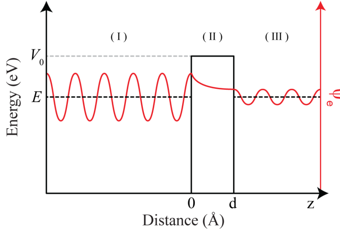
Figure 2.2: Quantum tunneling through a one-dimensional potential barrier with height V_0 and width d . An electron wavefunction, \psi_e , is represented by a complex plane wave in region (I), where V(z) = 0 , and experiences a real-valued decay within region (II), where V(z) > E . The electron is shown to have tunneling through the barrier into region (III), where it forms another complex plane wave with smaller amplitude.
