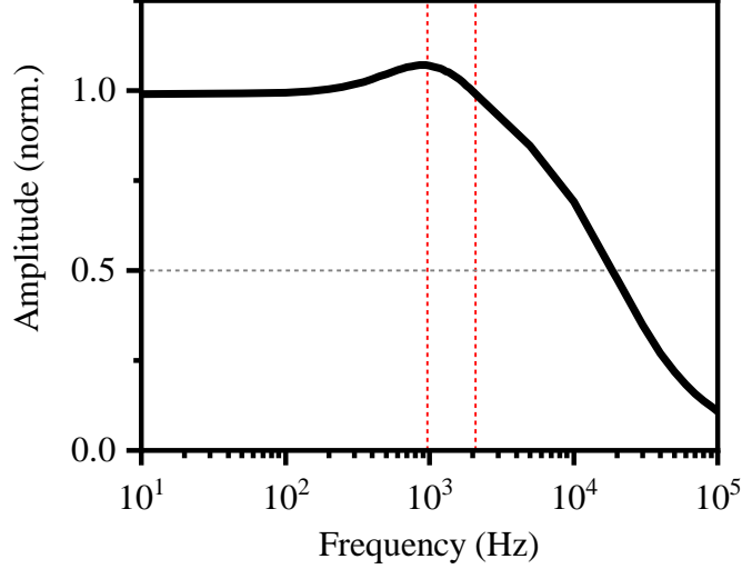
Figure 2.12: Frequency dependent transfer function for our FEMTO low-noise pre-amplifier operating at maximum gain of 10^9 V/A. The response curve is normalized to the modulation amplitude used during the measurement, 100 mV. Red dashed lines indicate commonly used modulation frequencies for THz-STM (963 Hz) and STS (2083 Hz).
