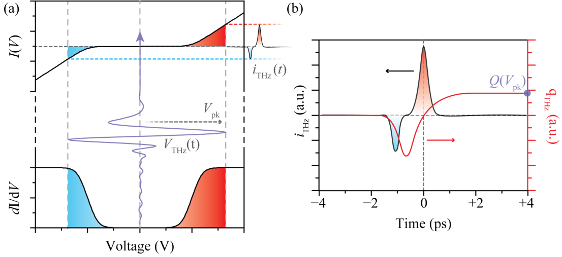
Figure 4.4: Rectification of THz-induced current pulses. (a) An ultrafast voltage transient, V_{\text{THz}}(t) , is applied to an I(V) curve. The nonlinearities of the I(V) produce an asymmetry in the current pulse, i_{\text{THz}}(t) . (b) The instantaneous rectified charge, q_{\text{THz}}(t) , is the running integral of the current pulse and its final value is the net rectified charge, Q_{\text{THz}}(V_{\text{pk}}) . Changing the size of the voltage waveform by adjusting V_{\text{pk}} samples different regions of I(V) to produce different values of Q_{\text{THz}}(V_{\text{pk}}) .
