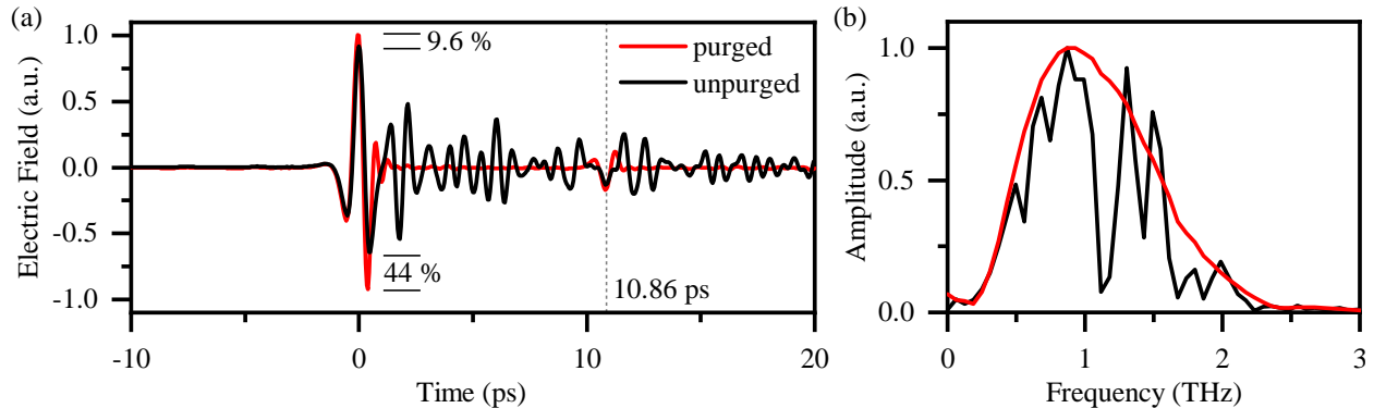
Figure 3.8: Long-time EOS measurements of our THz pulses with and without a dry air purge. (a) A pristine EOS trace acquired at < 0.05 % humidity is shown (red) to contrast against a waveform measurement performed under ambient conditions (black). Significant ringing is present as a result of THz absorption by \text{H}_2\text{O} in the atmosphere. (b) FFTs of the waveforms in (a) in the range -8 to 8 ps. The time window is narrowed to avoid reflections like the one indicated in (a) (a THz reflection from the 0.5 -mm-thick Si beamsplitter) that would introduce Fabry-Perot resonances in the FFT. The waveforms in (a) are normalized to the maximum of the purged signal, the resulting changes in field strength are indicated in percent. The amplitude spectra in (b) are normalized to the maximum of the individual data.
