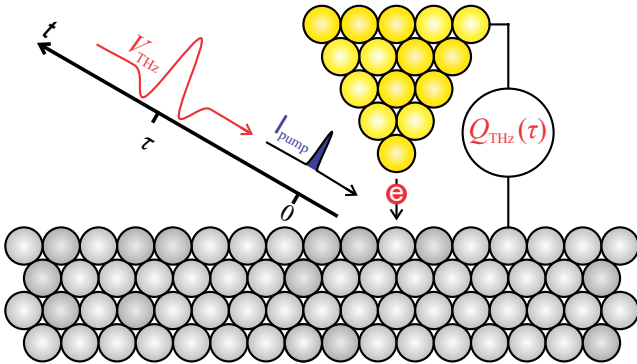
Figure 4.9: Schematic depicting an optical-pump/THz-STM-probe measurement of a transient I(V) . The pump pulse is absorbed by the sample at t = 0 , triggering a modification of the I(V) within the pump intensity envelope ( I_{\text{pump}} ). The evolution of the junction is read out via the rectified current ( Q_{\text{THz}}(\tau) ) generated by a time-delayed THz voltage probe ( V_{\text{THz}} ).
