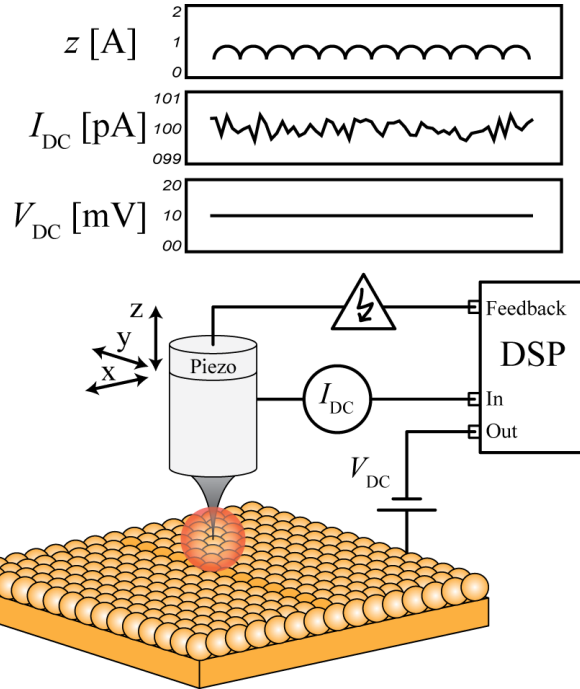
Figure 2.4: Illustration of the basic operational principles of the scanning tunneling microscope.
