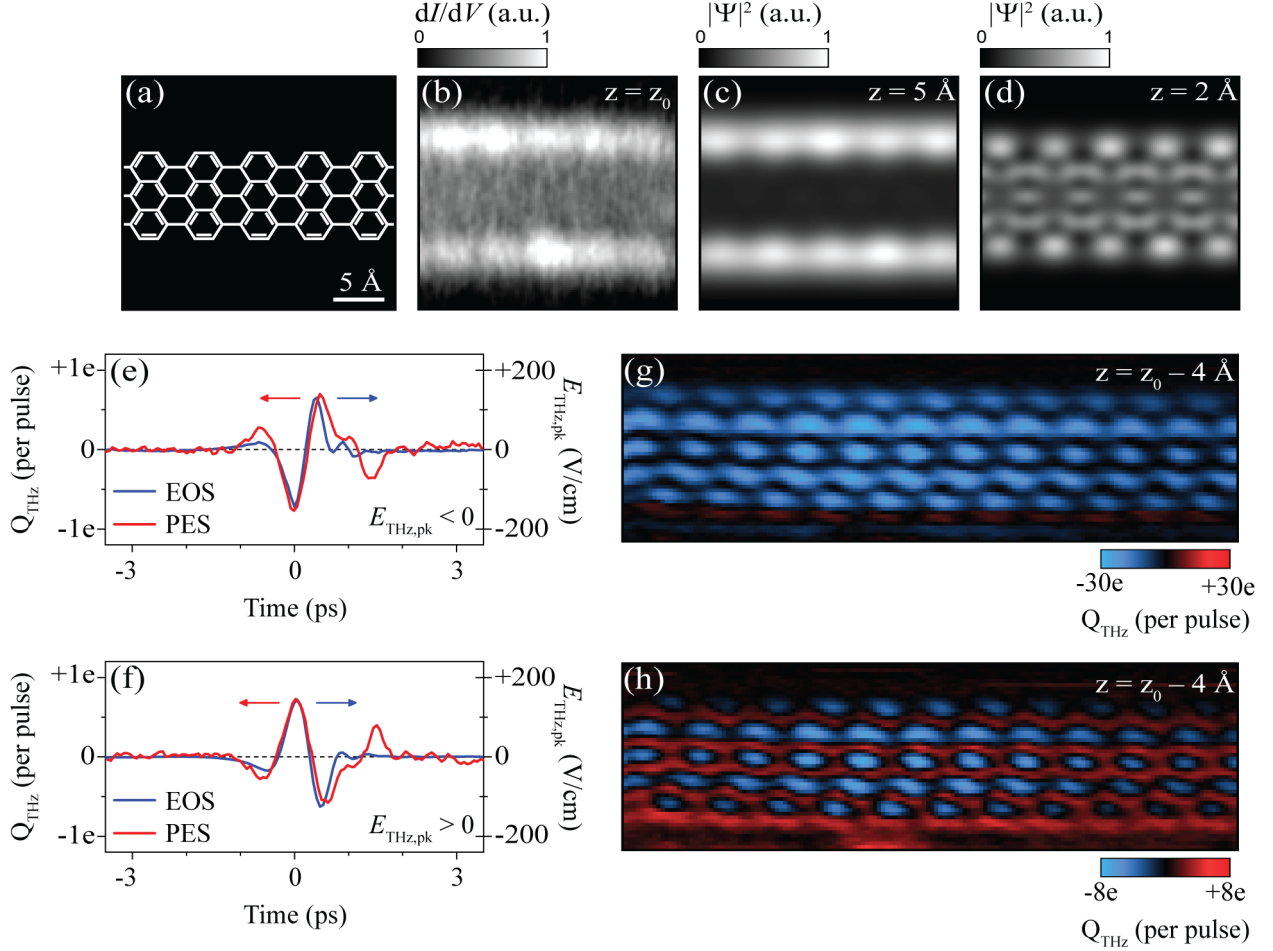
Figure 6.2: THz-STM of seven-atom-wide graphene nanoribbons on Au(111). (a) The chemical sketch of a 7-AGNR segment. The scalebar applies to all images in the figure. (b) Measured steady-state STM constant-height dI/dV acquired at V_{DC} = -1 V. The initial tip height, z_0 , was set with the tip located at the center of the nanoribbon at V_{DC} = -1 V and I_{DC} = -50 pA. (c),(d) Electron probability density, |\Psi|^2 , at V = -0.9 V calculated using DFT at a tip height of (c) 5 Å and (d) 2 Å. (e),(f) THz-pulse waveforms measured via free-space electro-optic sampling (EOS, blue curves) and photoemission sampling at the tip apex (PES, red curves). The carrier-envelope-phase shift between (e) and (f) is 180°. (g),(h) THz-STM constant-height rectified charge maps, Q_{THz}(x, y) , acquired at E_{THz,pk} = -180 V/cm (g) and E_{THz,pk} = +180 V/cm (h), with V_{DC} = 0 V and z = z_0 - 4 Å for both images.
