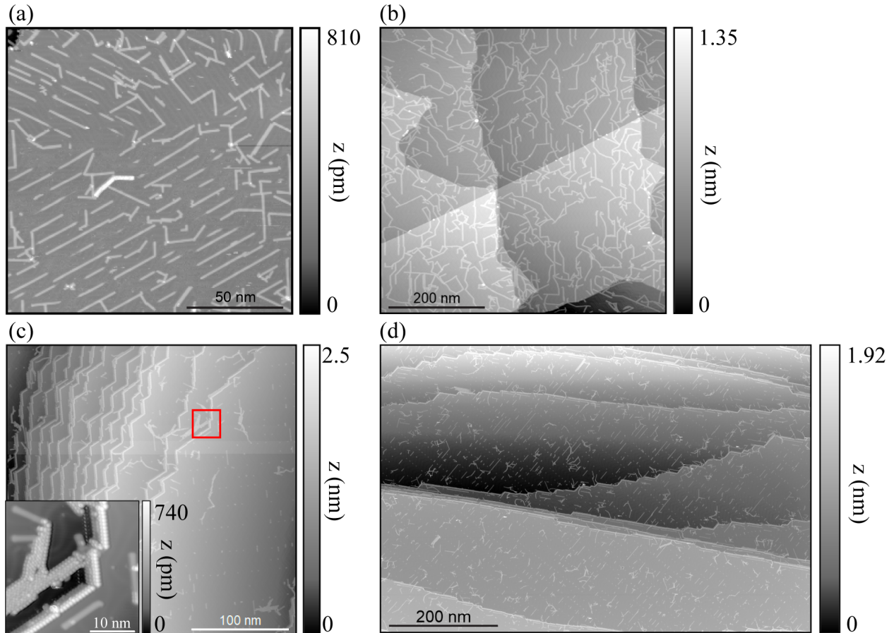
Figure 5.3: GNR samples produced under different growth conditions and procedures. (a) and (b), Results from using a slow annealing rate to transition between temperature setpoints where the temperature was held constant for several minutes. Results in (a) were deemed successful with long disconnected ribbons while the result in (b) are considered a failure due to the formation of large ribbon networks. (c) and (d), Results from a fast anneal rate from room temperature to final temperature setpoints (c, 370 K and d, 440 K). The sample in (c) showed significant clustering at the substrate step-edges and only produced polymers (inset). Results in (d) are considered successful with the formation of long disconnected ribbons spread across the sample surface. All images acquired in constant-current mode with parameters (a):, V_{DC} = -1 V and I_{DC} = -50 pA; (b): V_{DC} = -2 V and I_{DC} = -50 pA; (c): and inset, V_{DC} = 1.5 V and I_{DC} = 100 pA; (d): V_{DC} = 1.5 V and I_{DC} = 100 pA.
