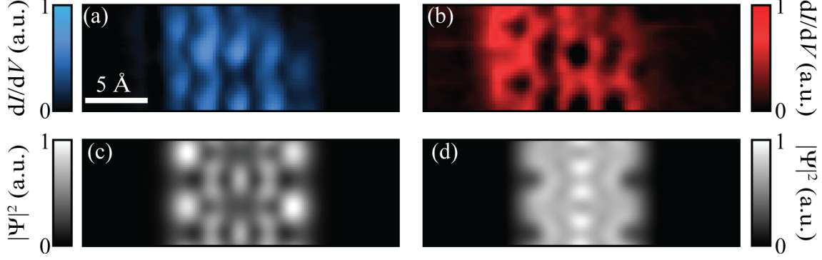
Figure 6.5: Atomically resolved dI/dV maps extracted from THz-STs. (a),(b) Model dI/dV maps at negative (a) and positive (b) bias extracted pixel-by-pixel from field-dependent Q_{\text{THz}}(x, y) images in Figure 6.4. (c),(d) Electron probability density at z = 2 \text{ \AA} and V = -0.9 \text{ V} (c) and V = +1.3 \text{ V} (d) calculated by DFT. The scalebar in (a) applies to (a) – (d).
