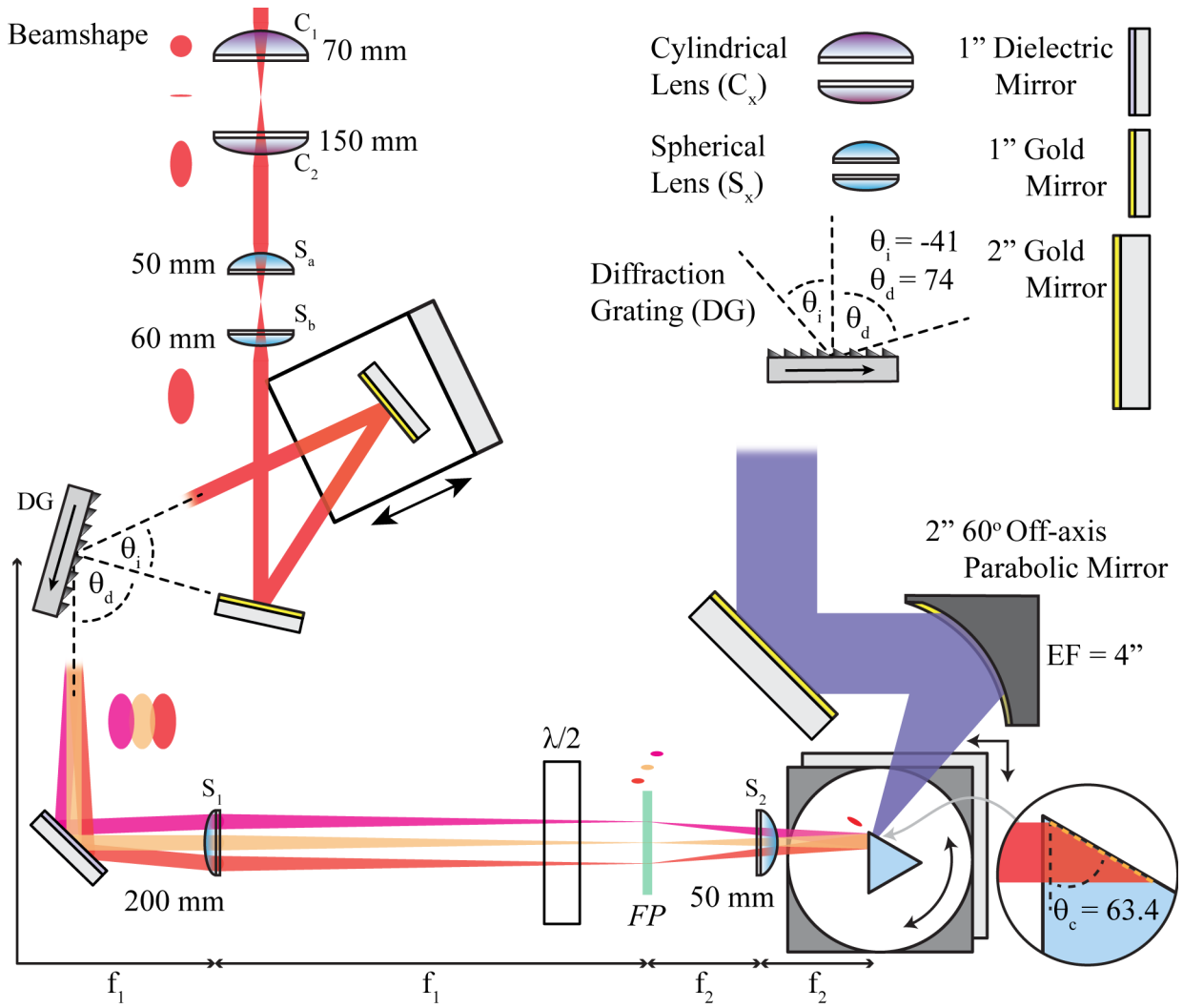
Figure 3.4: A schematic for our 4f tilted-pulse-front setup to generate THz pulses in LiNbO 3 . The beam shape is indicated by colored ellipses aside the optics along the beam path. A pair of cylindrical lenses ( C_1 and C_2 ) create a vertical ellipticity in our NIR laser beam (red, \lambda = 1030 nm). The spherical lens pair ( S_a and S_b ) expand the beam by a factor of 1.2 to decrease the power density on our Thorlabs 300 lines/mm diffraction grating. A stage is used to align the NIR beam into the grating at \theta_i = -41 deg. The ‘blaze arrow’ indicates the direction of the beam diffracted through the m = -1 order at \theta_d = 74 deg, leading to diverging colors (multicolored ellipses). The 4f setup is defined by spherical lenses S_1 and S_2 with focal lengths f_1 = 200 mm and f_2 = 50 mm. S_1 collimates the diverging colors and focuses each beam to a spot in the Fourier plane (FP). At the Fourier plane, the colors are focused at different positions. A half waveplate ( \lambda/2 ) rotates the polarization to vertical, aligning it with the crystal’s electro-optic axis. S_2 recombines the colors at a color focus while simultaneously creating the desired pulse front tilt. Due to the choice of magnification from the 4f telescope and grating density, the NIR pulse front tilt matches the Cherenkov angle, \theta_C = 64 deg, inside the LiNbO 3 crystal for optimized THz pulse generation.
