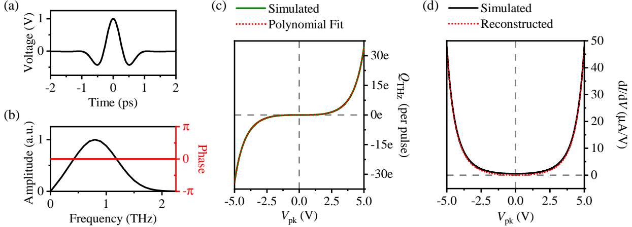
Figure 7.1: Reconstructing a Simmons model differential conductance. (a) Simulated THz voltage waveform, V_0(t) and (b) corresponding spectral amplitude (black curve) and phase (red curve). The amplitude is zero at 0 THz, i.e. the temporal integral of V_0(t) is zero. (c) Simulated rectified charge (green curve) for a Simmons model with \Phi_s = \Phi_t = 5 eV and polynomial fit of order N = 22 (dotted red curve). (d) Simmons model differential conductance (black curve) and reconstructed differential conductance (red curve) obtained from the steady-state inversion algorithm.
