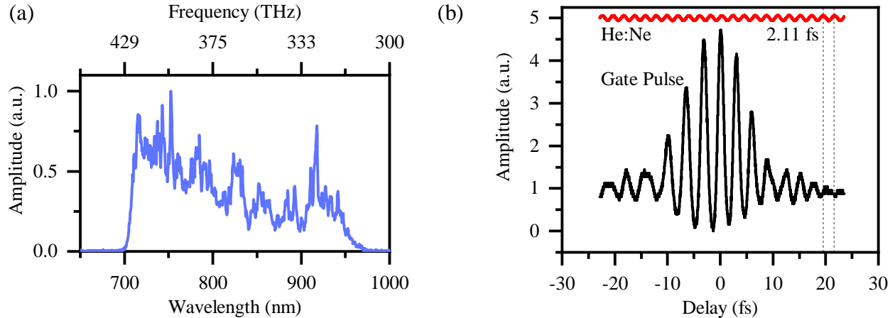
Figure 3.10: Verification of ultrashort gate pulse duration for EOS measurements. (a) Measurement of the 10-mW-average-power gate pulse using a Flame spectrometer from Ocean Optics. The spectrum spans 112 THz, from 700 nm to 950 nm. (b) Interferometric autocorrelation trace of the ultrashort gate pulse (black) produced from a white-light supercontinuum. The time axis is determined by the interference period (2.11 fs) of a CW He:Ne laser (red) with a wavelength of 633 nm.
