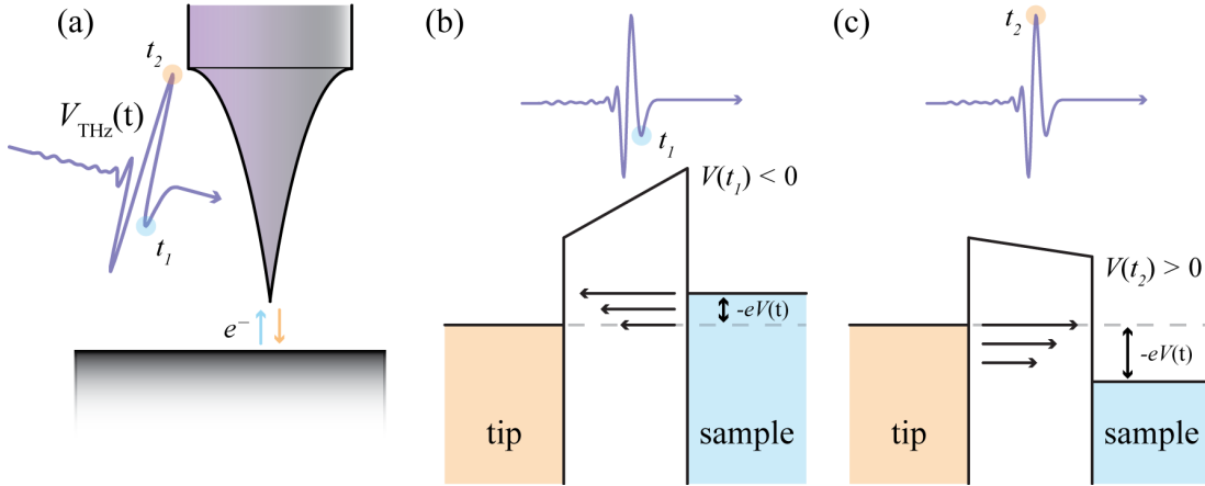
Figure 4.3: THz induced modification to the potential energy landscape of an STM tunnel junction. (a) A free-space THz pulse is coupled to tip of an STM, where it acts as a quasi-static bias voltage, V_{\text{THz}}(t) , and induces a current across the tunnel junction. As the voltage evolves it opens different tunnel pathways. (b) During negative half-cycles, tunneling is allowed from the sample into the tip, resulting in negative current. (d) During positive half-cycles, a positive current is induced, as electrons are able to tunnel into unoccupied states of the sample.
