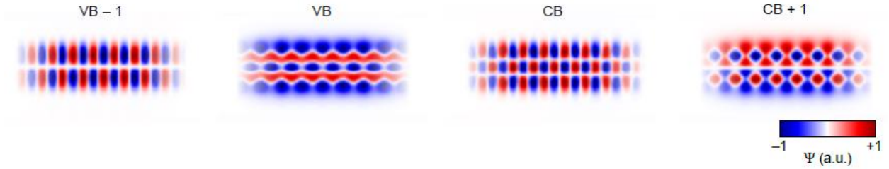
Figure 5.6: Simulated planar cross-sections of the electron wavefunction at several energy band resonances. Spatial distribution of the electron wavefunction, \Psi , for energies near the second valence band (VB-1), valence band (VB), conduction band (CB) and second conduction band (CB+1) calculated using density functional theory at a tip-sample distance of z = 2.0 \text{ \AA} . The calculation was performed with the 7-AGNR in the gas phase and the height is in reference to the atomic lattice of the 7-AGNR.
