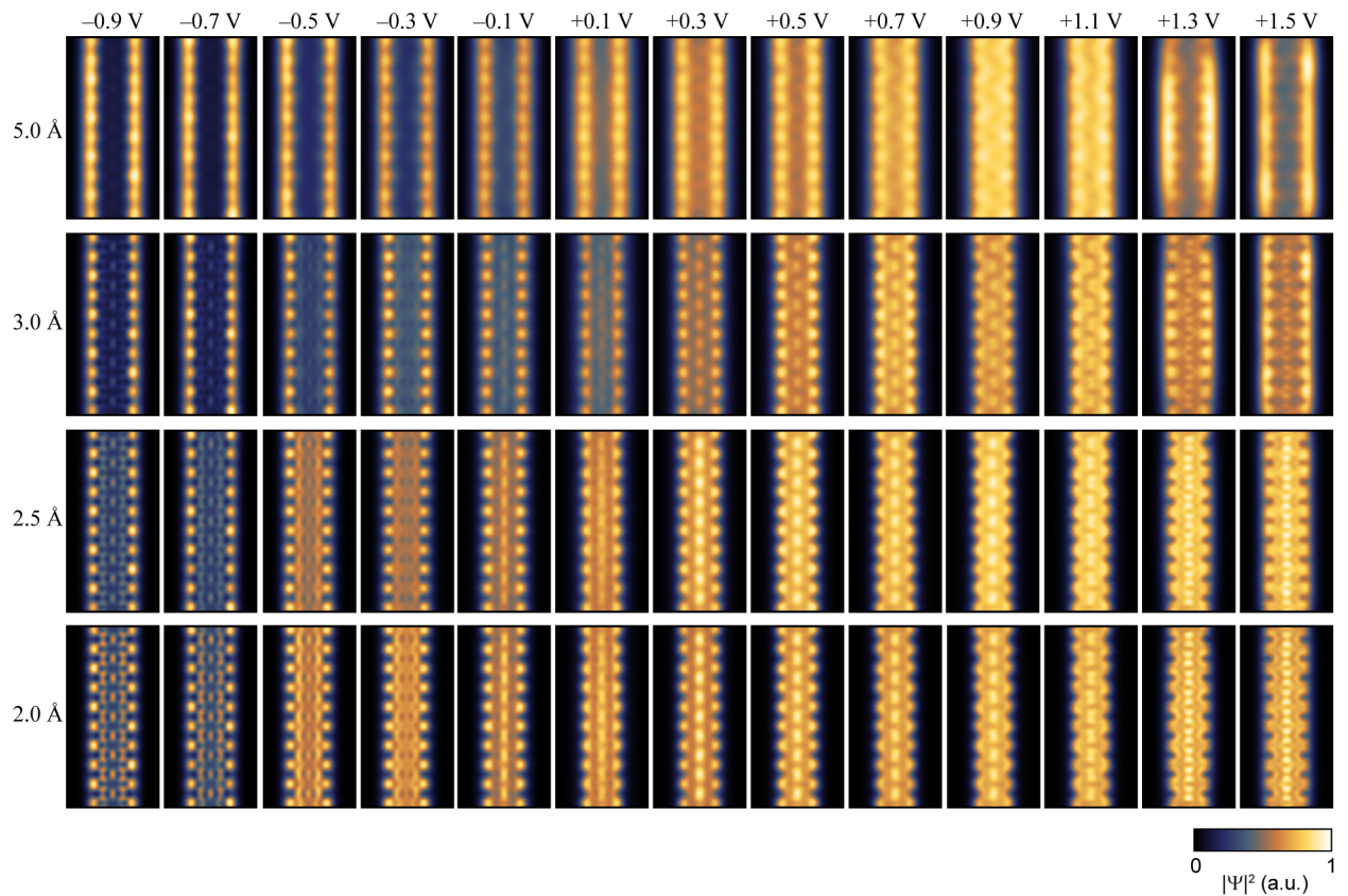
Figure 5.7: Simulated planar cross-sections of the probability density for a 7-AGNR as a function of distance and energy. Spatial distribution of the electron probability density, |\Psi|^2 , is calculated for energies ranging from 0.9 eV below to 1.5 eV above the Fermi level (see Reference [12] Methods). Image size 2 nm \times 4 nm. The height of the planar cross-section is referenced to the atomic lattice of the 7-AGNR. The colormap was set independently for each image. The calculation was performed with the 7-AGNR adsorbed on an Au(111) surface.
