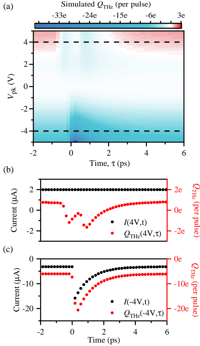
Figure 7.5: Simulated pump-probe THz-STs data. The simulation is performed using the THz voltage waveform in Figure 7.1(a) and the time-dependent differential conductance model described in the text, where the definition of the delay time \tau is shown in Figure 7.4(b). (a) Rectified charge map produced by the simulation. The algorithm was applied to a \tau window from -5 ps to 15 ps; a cropped region is presented to highlight detail on the subpicosecond timescale. Dashed lines are guides indicating the cross-sectional cuts shown in (b) and (c). (b) Cut through the rectified charge map at V_{\text{pk}} = 4 V (red circles) and simulated I(t) at V = 4 V for comparison (black circles). (c) Cut through the rectified charge map at V_{\text{pk}} = -4 V (red circles) and simulated I(t) at V = -4 V for comparison (black circles).
