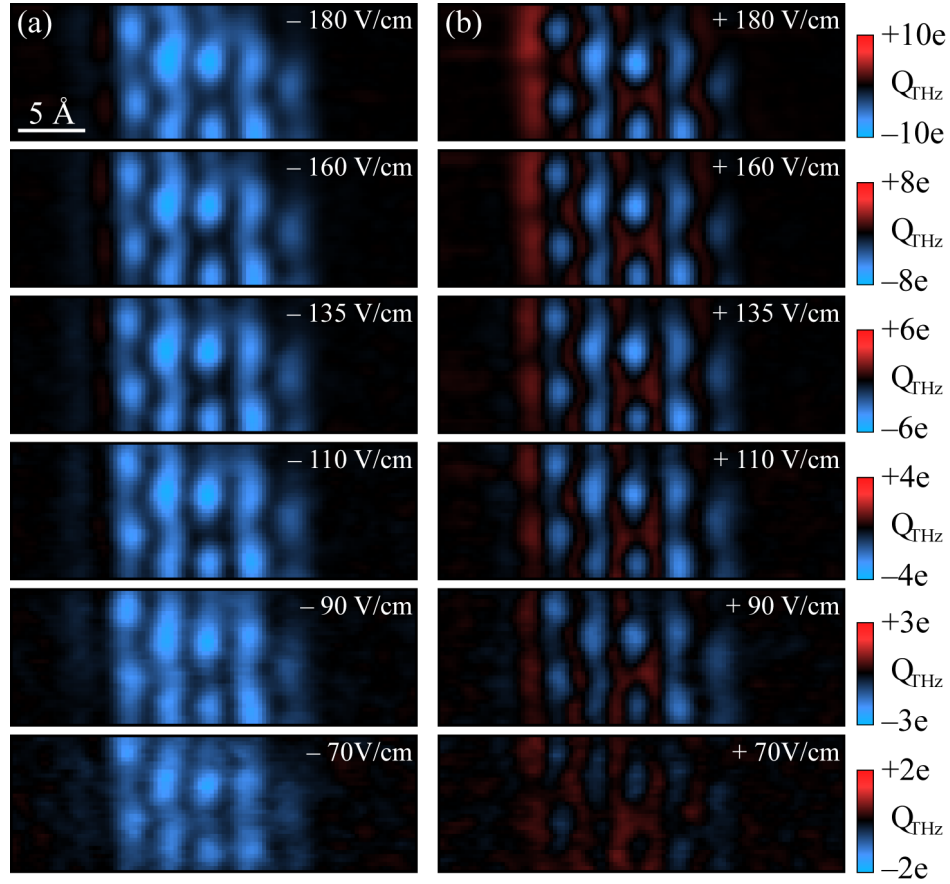
Figure 6.4: THz-STM field dependent imaging. (a),(b) THz-STM constant-height rectified charge maps acquired at several E_{\text{THz,pk}} using a negative-field-dominant THz pulse (a) and a positive-field-dominant THz pulse (b). The images were acquired with the tip at z = z_0 - 4 \text{ \AA} . A 5 \times 5 smoothing filter was applied to the dataset.
