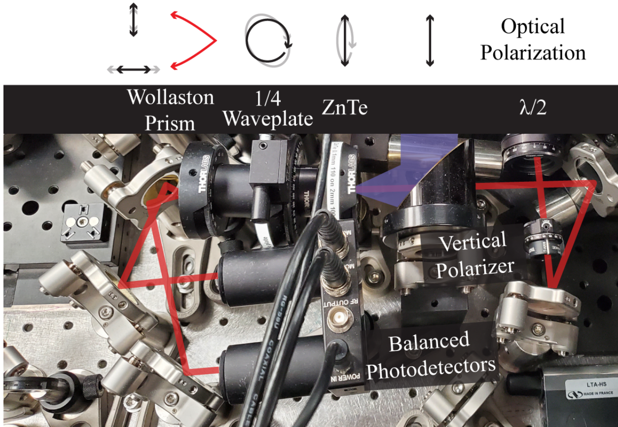
Figure 3.6: Electro-optic sampling setup used to perform time-domain measurements of the THz electric field transient. Optical gate pulses (red beamline, \lambda = 800 nm) pass through a waveplate ( \lambda/2 ) and vertical polarizer for attenuation and then through an aperture in the back of a 90^\circ off-axis parabolic mirror. THz pulses (purple beamline) enter along the collimated axis of the parabolic mirror before being focused into a 100 \mu\text{m} ZnTe(110) detection crystal mounted to a 2 mm ZnTe(100) crystal. The gate and THz pulses propagate co-linearly through the ZnTe crystal. The gate pulse ellipticity changes throughout the setup, as illustrated at the top. The ellipticity in the absence of a THz field (black arrows) is initially vertical and is converted to a circular polarization by a \lambda/4 waveplate. A Wollaston prism separates the gate pulses into horizontal and vertical polarization components before directing them into a balanced photodetector. In the presence of a THz field, THz-induced birefringence imparts a small ellipticity to the gate pulse, resulting in an imbalance between vertical and horizontal polarization after the \lambda/4 waveplate. The gate polarization in the presence of a THz field is illustrated at the top as grey arrows.
