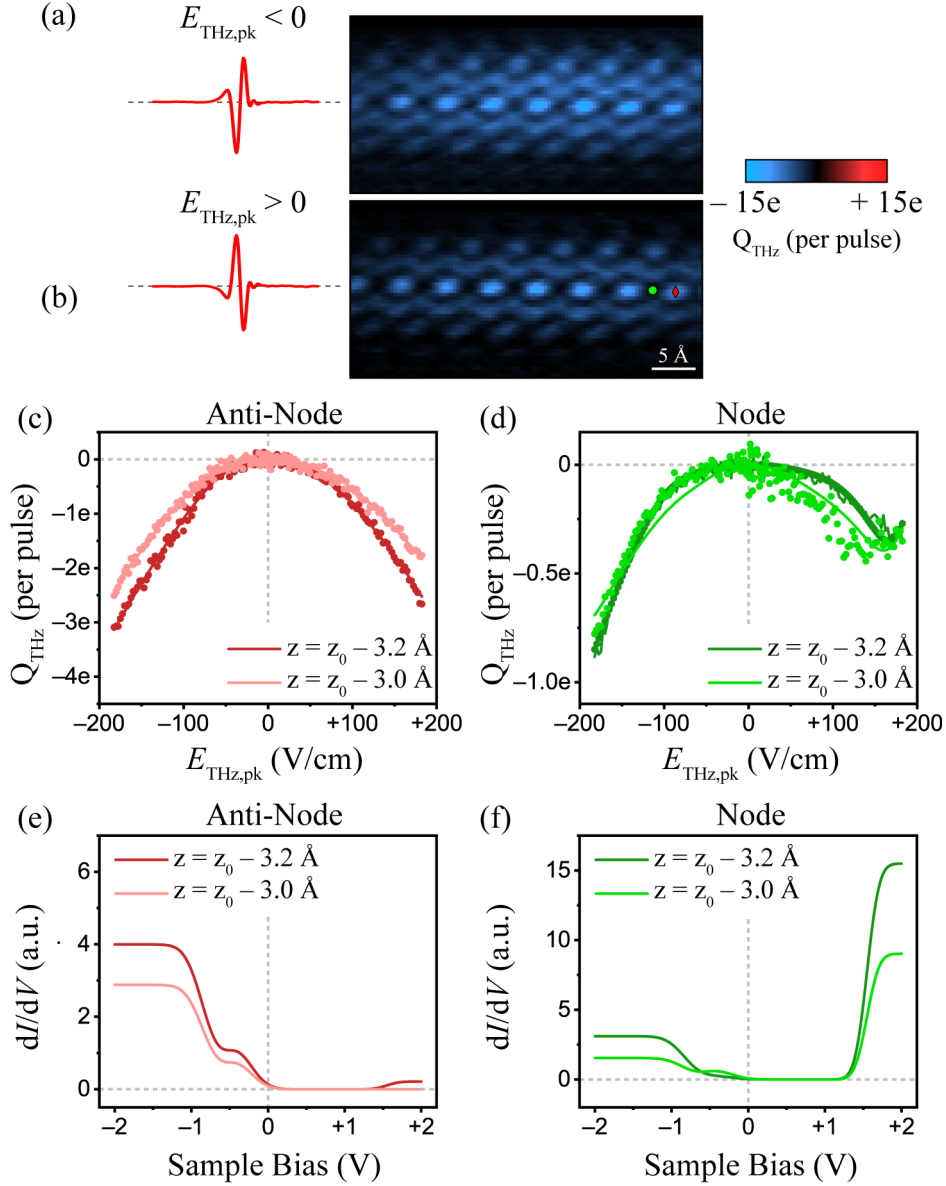
Figure 6.7: THz-STM imaging and spectroscopy of another 7-AGNR with a different tip apex. (a),(b) THz-STM constant-height rectified charge maps acquired at E_{\text{THz,pk}} = -135 \text{ V/cm} (a) and E_{\text{THz,pk}} = +135 \text{ V/cm} (b), with V_{\text{DC}} = 0 \text{ V} and z = z_0 - 3.0 \text{ \AA} for both images. The red triangle and green circle indicate the THz-STs locations for the anti-node and node, respectively. (c),(d) Measured (circles) and simulated (solid lines) Q_{\text{THz}}-E_{\text{THz,pk}} curves at z = z_0 - 3.2 \text{ \AA} (dark lines/symbols) and z = z_0 - 3.0 \text{ \AA} (light lines/symbols) with the tip positioned at the anti-node (c) and node (d) of the valence band LDOS ( V_{\text{DC}} = 0 \text{ V} ). (e),(f) Model dI/dV extracted from the fits in (c) and (d) for the anti-node (e) and node (f) tip positions, respectively.
