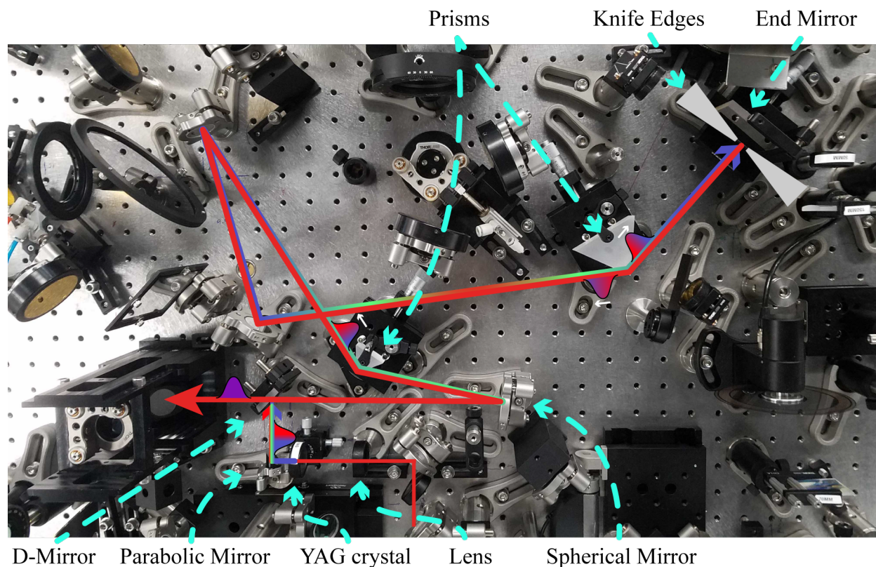
Figure 3.9: Supercontinuum white-light generation and prism compressor. An ultrafast NIR pulse ( \lambda = 1030 \text{ nm} ) with a pulse energy of \sim 500 \text{ nJ} is focused into a 4-mm-thick YAG crystal by a 2-inch focal length (50.8 mm) spherical lens. A 0.5-inch focal length (12.7 mm) silver 90^\circ off-axis parabolic is used to collimate the white-light and direct it toward a D-mirror. The white light is reflected into a 500-mm focal length spherical mirror that focuses through the prism compressor to a 2-inch diameter (50.8) mm square silver mirror. The mirror is on a stage to optimize its position at the Fourier plane generated by refraction through the prisms within the compressor and focusing optics. The white-light pulse propagates through a small prism (BK7) and large prism (BK7) whose separation distance, in combination with the focal length of the spherical mirror, dictate the dispersion compensation of the compressor. The multi-colored beampath indicates the white-light spectrum that enters the compressor and the red beampath indicates the spectrum that is selected by the knife edges at the Fourier plane. Gaussian distributions and white arrows indicate the relative orientation of the colors within the pulse. Positive dispersion is experienced during supercontinuum generation (red followed by blue at the YAG crystal). Refraction through the prisms provides negative dispersion that inverts the orientation of the colors (blue followed by red at the Fourier plane). At the output of the compressor the dispersion is minimized and the colors are evenly distributed throughout the pulse (blue and red are mixed to make purple after the D-mirror).
