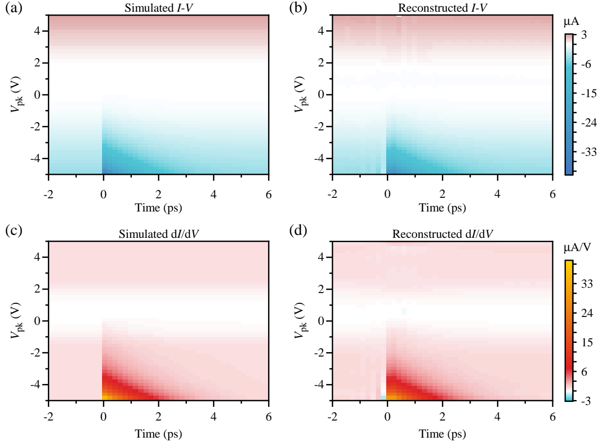
Figure 7.6: Reconstructing a transient I(V) curve and differential conductance with the time-dependent inversion algorithm. (a) Original I(V) used to simulate the THz-STs data shown in Figure 7.5(a). (b) Reconstructed I(V) obtained using the time-dependent inversion algorithm. (c) Differential conductance for the model tunnel junction in (a). (d) Reconstructed differential conductance determined alongside (b) using the inversion algorithm. Fitting of Q_{\text{THz}}(V_{\text{pk}}) in the algorithm was performed with a polynomial of order N = 21 . All plots are cropped along the time axis from the original bounds of -5 ps to 15 ps.
