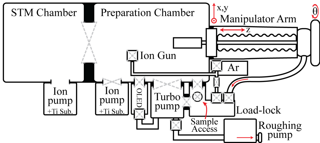
Figure 2.14: Schematic of the STM vacuum chamber. Valves are indicated by pairs of crossed grey dashed lines. Both the STM and preparation chambers are equipped with ion pumps capable of maintaining chamber pressures < 10^{-10} mBar. A turbo molecular pump is connected to the preparation and load-lock chambers and backed by a roughing pump. A leak valve connected to the ion gun is used to incorporate argon gas for ion bombardment. A circular access port is used to exchange tips and samples in/out of the vacuum system through the load-lock chamber. The manipulator arm maintains vacuum while moving in four degrees of motion and is pumped out through the load-lock chamber.
