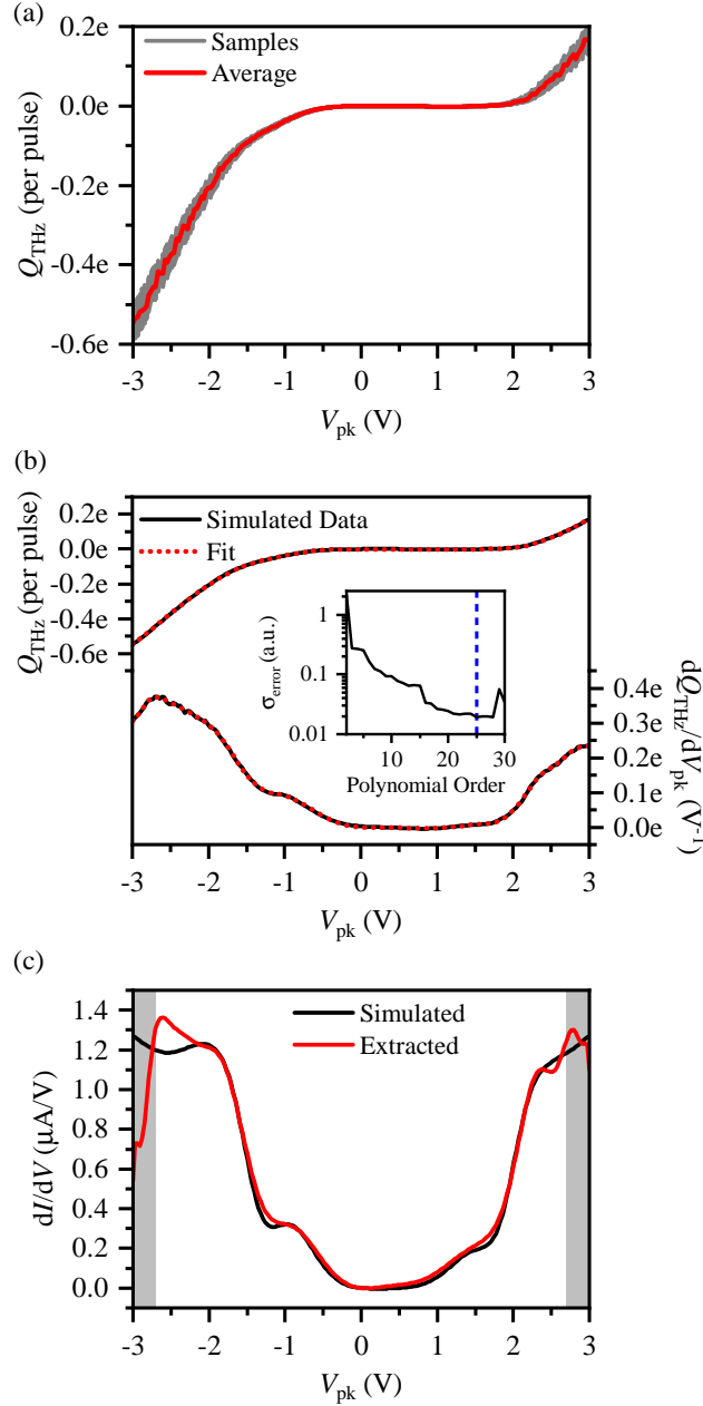
Figure 7.3: Reconstructing an arbitrary differential conductance in the presence of noise. (a) In a simulated THz-STs experiment, charge rectification is calculated for a voltage waveform with a randomly fluctuating field strength ( \epsilon_{\max} = 0.05 ; 10 calculations per V_{\text{pk}} ). The grey region shows the simulated experimental data and the red curve is the average.
