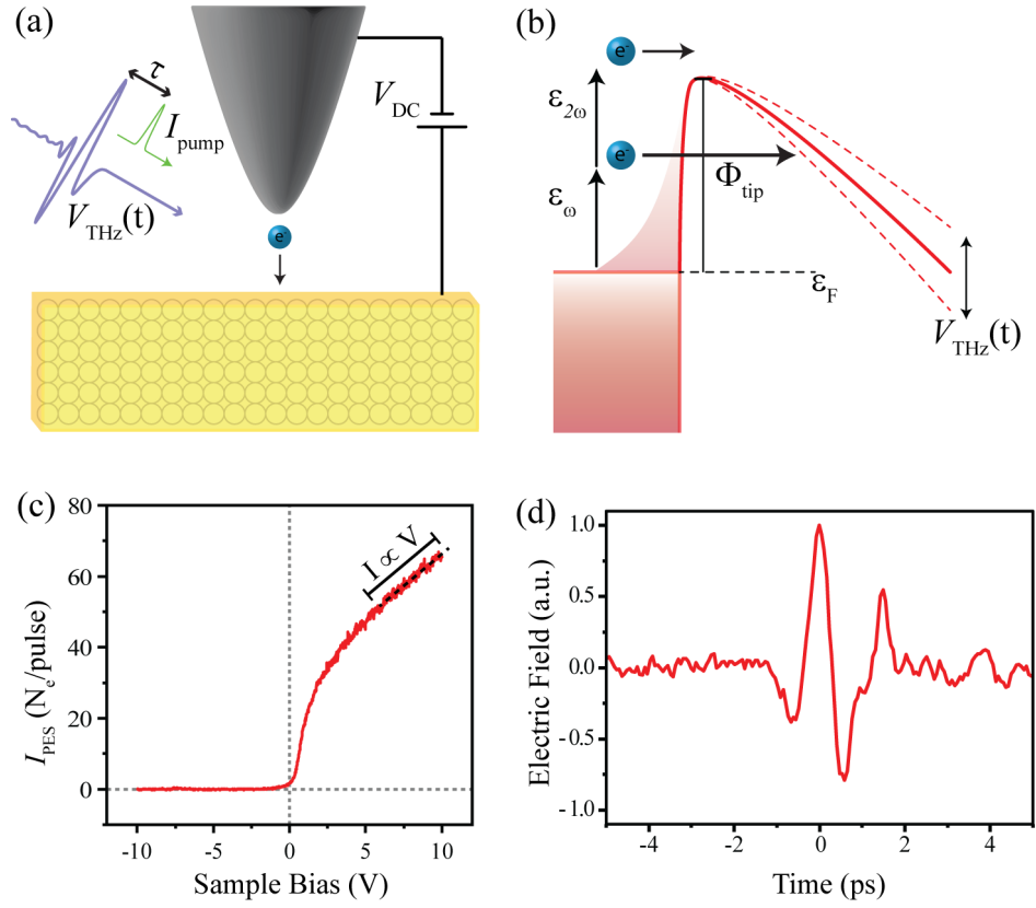
Figure 4.11: THz near-field waveform measurement by PES. (a) PES measurement geometry, an optical pulse ( I_{\text{pump}} , \lambda = 515 nm) photoexcites free-carriers in an STM tip held at positive bias, V_{\text{DC}} , producing an ultrafast photocurrent. A THz probe pulse follows at a time-delay, \tau , and couples to the STM tip. (b) Barrier schematic of the photoexcited junction. Multi-photon absorption promotes electrons from the Fermi level to higher energy levels of the tip, allowing for tunneling and photoemission. The THz probe pulse simultaneously applies a bias modulation that effects the total current generated during photoemission by changing the energy landscape proportional to V_{\text{THz}}(t) . (c) Average ultrafast PES current, I_{\text{PES}} , measured as a function of V_{\text{DC}} . A region of linear slope is identified near V_{\text{DC}} = 10 V. (d) THz near-field waveform measured with PES at V_{\text{DC}} = 10 V with an optical pulse energy of 30 nJ and a pulse duration of < 230 fs.
