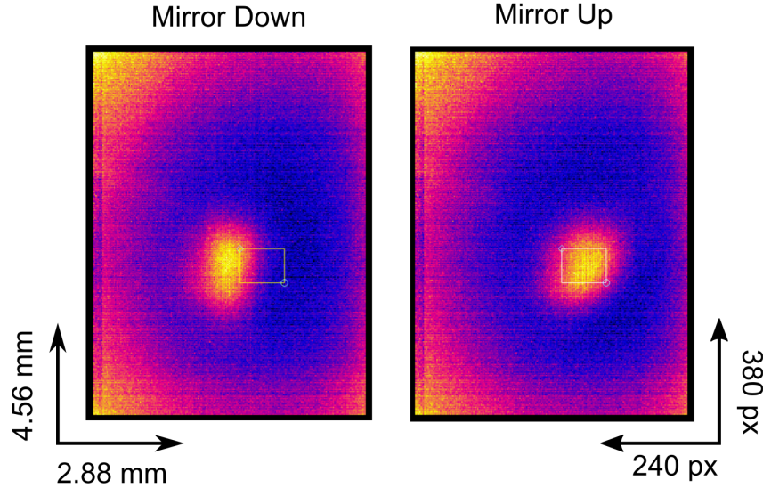
Figure 3.11: Images of the THz beam spot acquired by a SEEK Compact Pro thermal camera. The two images identify ‘mirror up’, which selects E_{\text{THz,pk}} > 0 , and ‘mirror down’ used for E_{\text{THz,pk}} < 0 . These images are used to optimize the pointing of our THz beam at various points throughout the setup. The contrast around the pulse comes from uneven exposure of the room temperature background.
