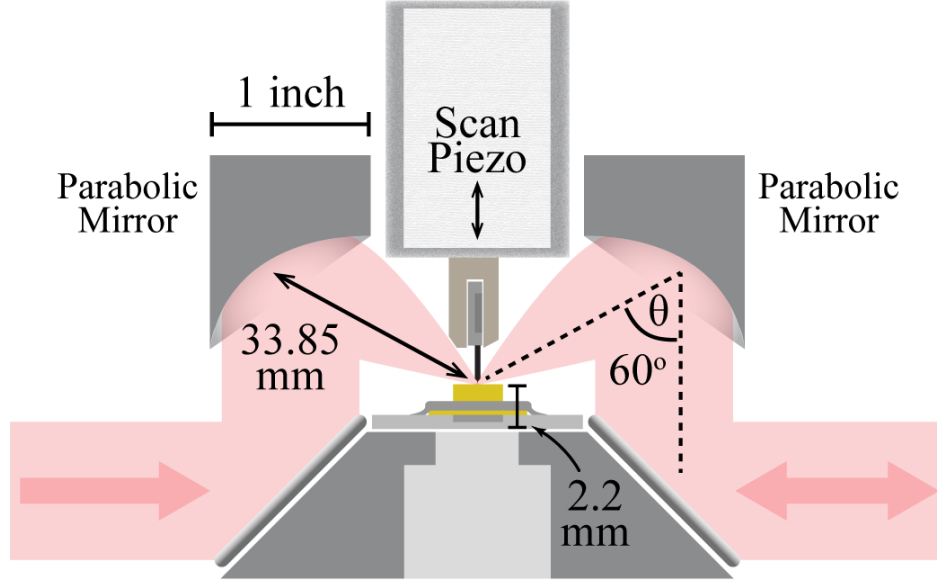
Figure 2.15: Schematic for the optical beam path on our custom Createc GmbH scan head. The scan head is equipped with a pair of 1 inch diameter, 60-degree off-axis parabolic mirrors with effective focal length of 33.8 mm. The scan piezo can be coarsely moved across the sample and vertically. To keep the tunnel junction within the optical focus, the sample + plate must be 2.2 mm in height and the parabolic mirrors are mechanically coupled to the scan piezo. The optical beam is incident from the left to reproduce our experimental setup and the right-side optical path may be used for illumination or collection of light coming from the focus.
