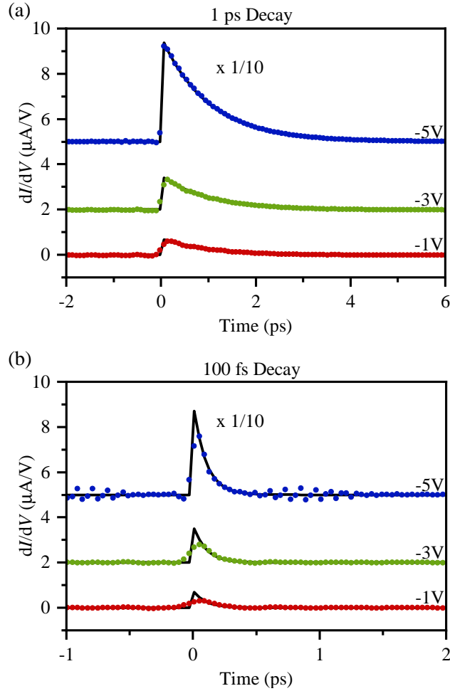
Figure 7.7: Resolving subcycle dynamics with the time-dependent inversion algorithm. The simulated I(V) is defined by a Simmons model that appears at t = 0 and subsequently decays away exponentially for t > 0 , as described in the text. For t < 0 , I = 0 and dI/dV = 0 . (a), (b) Simulated transient differential conductance at V = -5\text{ V} , V = -3\text{ V} , and V = -1\text{ V} (black curves, offset for clarity) for a decay time of (a) 1 ps and (b) 100 fs. The reconstructed transient differential conductance is shown for the same voltages ( V = -5\text{ V} : blue circles; V = -3\text{ V} : green circles; V = -1\text{ V} : red circles). Fitting Q_{\text{THz}}(V_{\text{pk}}) in the time-dependent algorithm was performed with a polynomial of order n = 21 for both 1 ps and 100 fs calculations. In both panels, the plots are cropped from the original time axis of -5\text{ ps} to 15\text{ ps} that was used in the time-dependent algorithm. Panel (b) was calculated using 500 points along the time axis compared to 250 points for panel (a) to facilitate analysis at higher frequencies.
