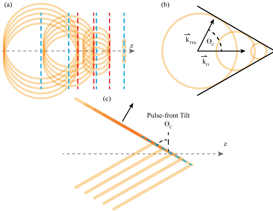
Figure 3.3: An illustration of the Cherenkov cone produced in \text{LiNbO}_3 . (a) An optical pulse with a pulse front perpendicular to the z axis (blue), propagating with wavevector, \mathbf{k}_O , generates Huygen's THz wavelets uniformly across the front (orange). Lack of phase matching with the the pulse front prevents the wavelets from different pulse front locations from constructively interfering. (b) Wavelets produced along the optical axis define a THz wavefront at the Cherenkov angle, \theta_C . (c) Tilting the optical pulse front at \theta_C = 64^\circ allows THz wavelets to constructively interfere along \mathbf{k}_{THz} , thereby increasing in amplitude to form a strong THz wave propagating along \mathbf{k}_{THz} (dark orange).
