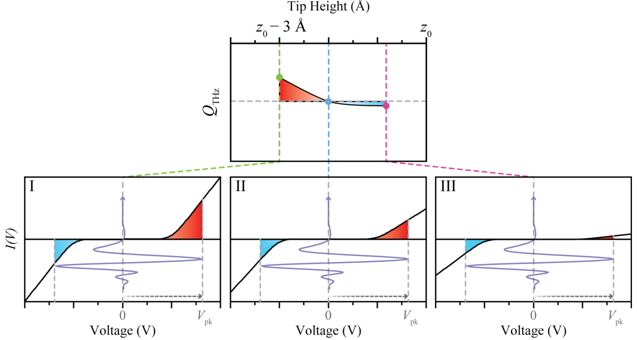
Figure 4.10: Illustration of a THz-STs vertical spectroscopy measurement. The experiment is initialized at a height z_0 - 3 \text{ \AA} , then Q_{\text{THz}} is recorded while the tip is retracted. In position (I), the positive THz-induced current contribution due to features at positive voltage in I(V) outweighs the negative equivalent, resulting in Q_{\text{THz}} > 0 . At position (II), the positive nonlinearity of I(V) has decayed more than the negative with increasing z , so the two THz-induced current contributions are equal in weight, producing Q_{\text{THz}} = 0 . The decay trend continues into position (III), where the positive side of I(V) is almost zero and Q_{\text{THz}} < 0 .
