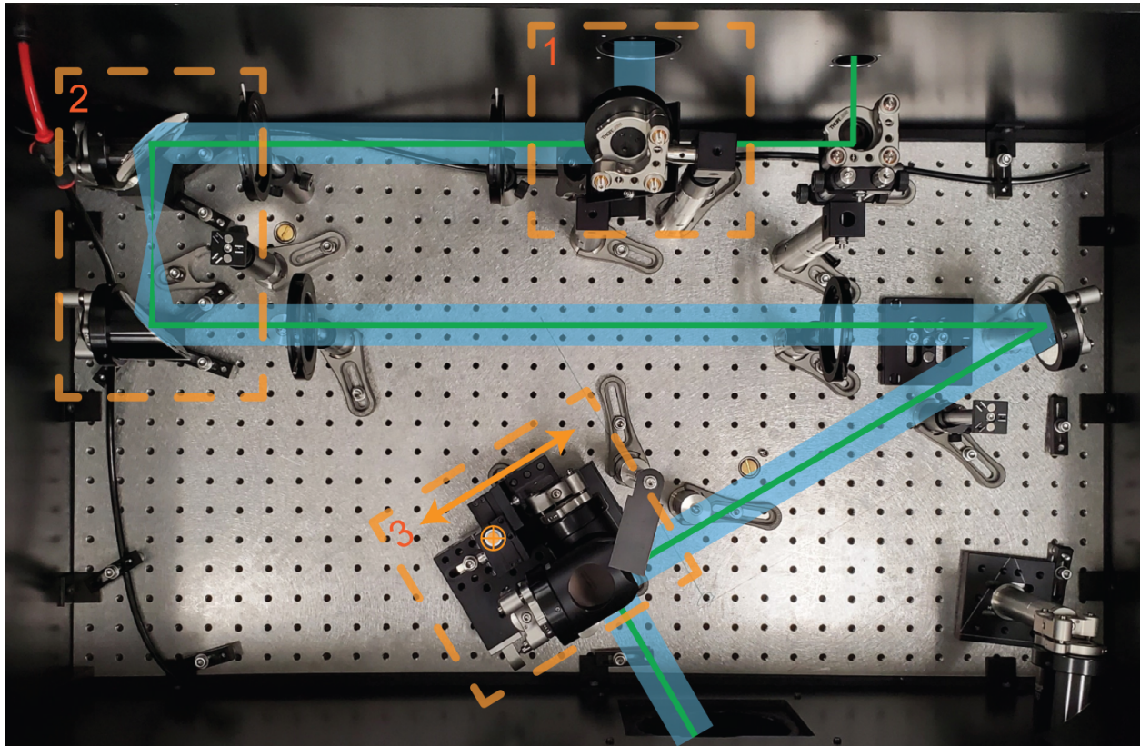
Figure 4.13: An overhead image of the THz-STM coupling setup. The THz beam path is indicated in blue and the optical beam path is shown in green. The setup is enclosed in a purge box with dry air supplied via the red inlet located at the left edge. Orange indicators show the final stage motion: an arrow for translation along the input beam direction and circles with a cross for vertical translation. The setup is constructed on a 24-inch by 48-inch optical breadboard (Newport PG-24-4-ML) and is removed during microscope bakeouts.
