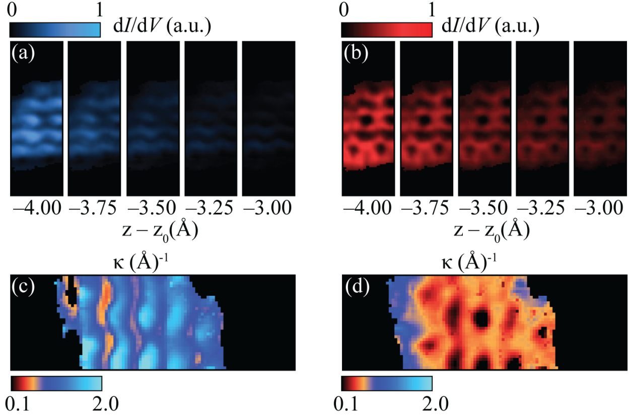
Figure 6.11: Tomographic dI/dV reconstruction from THz-STM tomography. (a),(b) Differential conductance for occupied (a) and unoccupied (b) states. (c),(d) Map of the inverse decay constant, \kappa , at negative (c) and positive (d) bias. Using the height-dependent Q_{\text{THz}}(x, y) data shown in Figures 6.10(a) and 6.10(b), we create a Q_{\text{THz}}(z) curve at each pixel. We fit the Q_{\text{THz}}(z) curves by incorporating an exponential decay into each term of Equation 6.1. Then, we use the field-dependent image data from Figure 6.4 to create a dI/dV map at z = z_0 - 4 \text{ \AA} used to initialize the model. The \kappa maps are spatially dependent decay coefficients for the dI/dV features at positive and negative bias. The regions within (c) and (d) that are represented by zero on the colormap (black) are artificially inserted because the local value for Q_{\text{THz}} and/or the dI/dV amplitude at the corresponding bias is negligible and \kappa cannot be determined.
