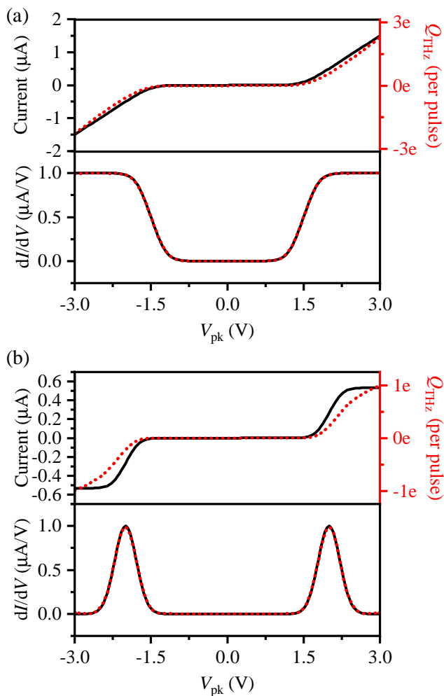
Figure 7.2: Reconstructing highly nonlinear differential conductances. (a) Top: I(V) for a simple model of a semiconducting sample with band onsets at -1.5 V and +1.5 V (black curve) and corresponding rectified charge (dotted red curve) produced by the THz voltage waveform in Figure 7.1(a). Bottom: differential conductance for the semiconductor model (black curve) and reconstructed differential conductance (dotted red curve). (b) Top: I(V) for a simple model of a molecule adsorbed on a salt film on a metal substrate with electronic orbitals centered at \pm 2 V (solid black curve) and corresponding rectified charge (dotted red curve) produced by the THz voltage waveform in Figure 7.1(a). Bottom: differential conductance for the molecular system (solid black curve) and reconstructed differential conductance (dotted red curve). Fitting of Q_{\text{THz}}(V_{\text{pk}}) in each system was performed with a polynomial of order N = 38 .
