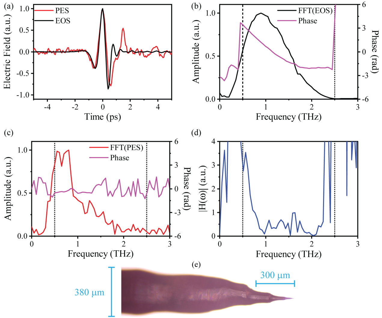
Figure 4.12: Comparison between THz electric far-field transient and near-field voltage transient. (a) A PES measurement of the THz near-field waveform (solid red curve) overlaid on the incident THz electric field measured by EOS. (b) EOS spectral amplitude (solid black curve) and phase (pink solid curve) calculated by FFT. (c) PES spectral amplitude (solid red curve) and phase (solid pink curve) calculated by FFT. (d) Absolute value of the transfer function, \tilde{H}(\omega) , between the EOS and PES waveforms for the STM tip shown in (e). (e) Optical image of the tungsten-wire STM tip used to record the THz-STM data presented here and in Chapter 6. The tip was \sim 3 mm long with a diameter of 384\mu\text{m} , and hosted a number of features on the scale of the THz wavelength. Dashed vertical lines in panels (b)-(d) indicate the boundaries to the region of most trustworthy data: 0.5 THz to 2.5 THz. Based on THz spectroscopy measurements using the same THz source. The THz spectroscopy measurements were performed by other members of the lab and are not within the scope of this thesis.
