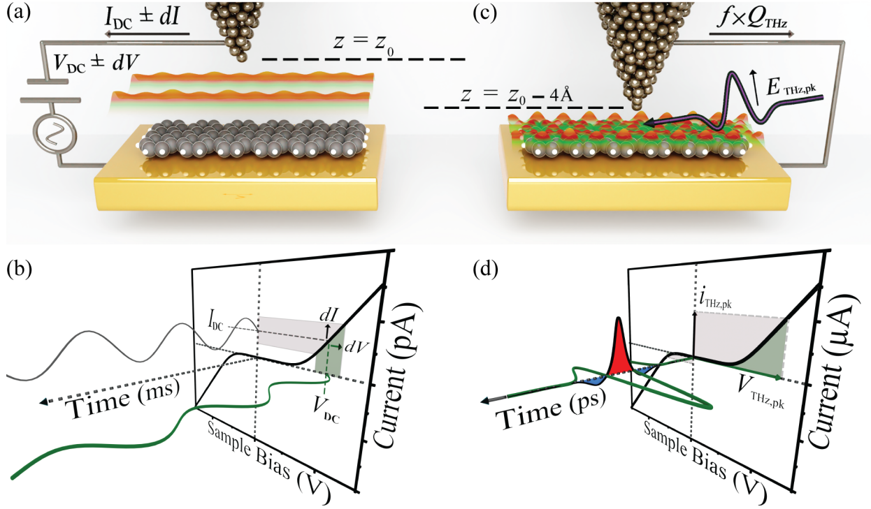
Figure 6.1: Comparing ultrafast terahertz scanning tunneling spectroscopy (THz-STs) to conventional STs. (a) Schematic diagram of the tunnel junction during scanning tunneling microscopy (STM) and STs of a seven-atom-wide armchair graphene nanoribbon (7-AGNR). The tip height, z_0 , is set by the tunnel current feedback conditions, e.g. with steady-state bias voltage V_{DC} = -1 V and steady-state tunnel current setpoint I_{DC} = -50 pA. (b) Schematic I(V) of a 7-AGNR (solid black line) with the time axis of the millisecond sine-wave modulation for conventional STs projected out-of-plane. In STs, the steady-state bias voltage is modulated by a sine-wave of amplitude dV (solid green curve), generating a tunnel current modulation of amplitude dI (solid grey curve). (c),(d) In THz-STM and THz-STs, a phase-stable single-cycle THz pulse with a peak electric field of E_{THz,pk} is coupled through free space to the STM tip apex, where it acts as an ultrafast transient bias with a peak voltage of V_{pk} . The tip height is reduced by approximately 4 Å to account for the reduced duty cycle of the bias compared to conventional STM. At this reduced tip height, the 7-AGNR LDOS features far richer spatial structure than at STM and STs tip heights (orange and green overlays in (a) and (c)). A THz voltage transient induces a sub-picosecond current pulse, i_{THz}(t) , defined by the I(V) , with peak current, i_{THz,pk} , reaching the \mu A scale, compensating for the low duty cycle of THz-STs. The average rectified component of the current pulses, Q_{THz} = eN_e = \int i_{THz}(t)dt , is measured as a steady-state current, I_{THz} = feN_e , where e is the elementary charge, f is the repetition rate of the laser and N_e is the average number of rectified elementary charges per THz pulse. The red and blue shadings underneath the sub-picosecond current transient in (d) emphasize the rectification process for a single pulse. The green and grey shaded regions in (b) and (d) highlight the range of the voltage modulation and resulting instantaneous tunnel current.
