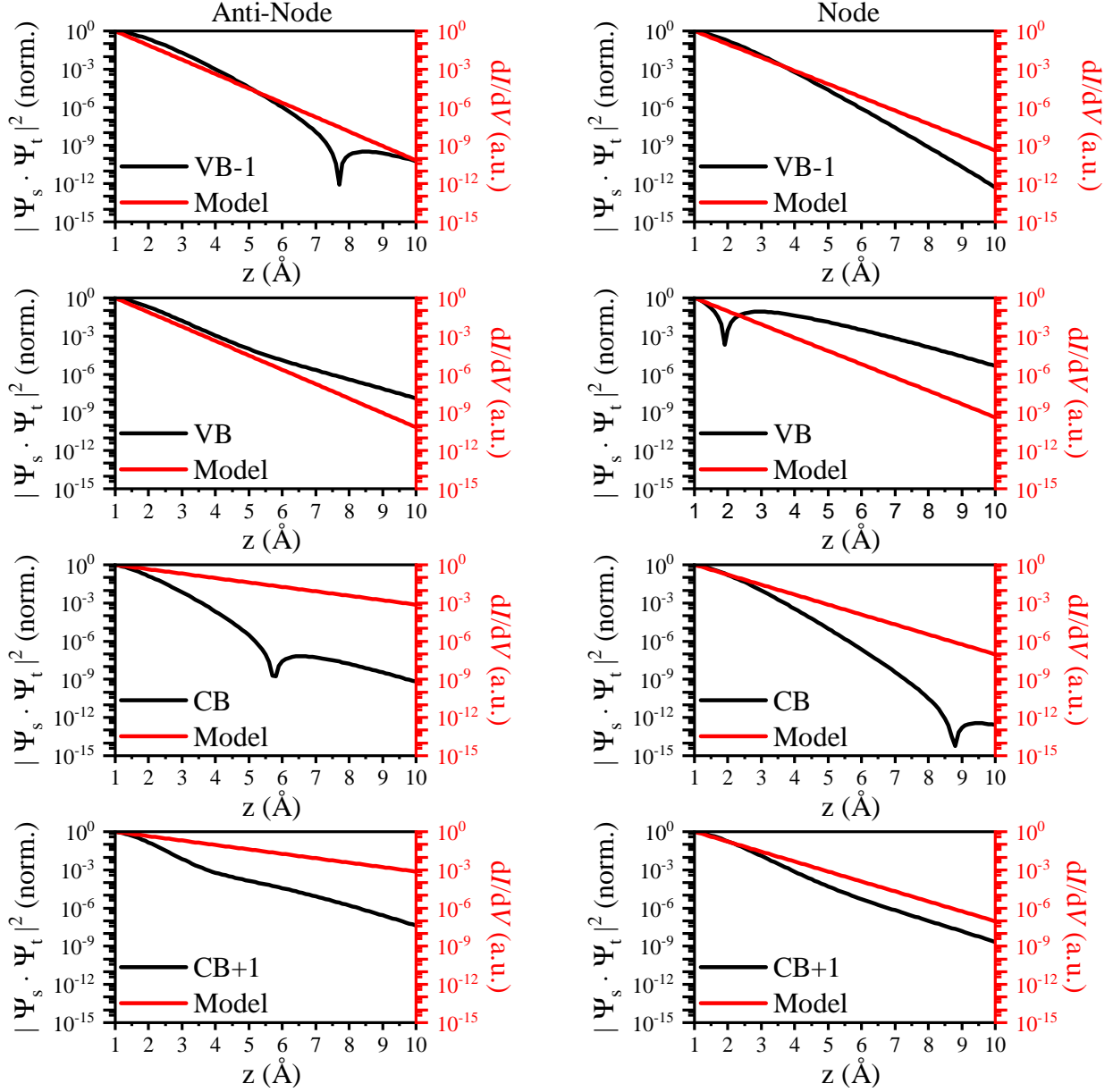
Figure 6.9: Comparison of the theoretical and experimental vertical decays at the anti-node and node positions. For each orbital and tip position, the theoretical vertical decay (solid black line) was calculated using a tight-binding model for the sample wavefunction ( \Psi_s ) that was convoluted with an s-wave tip ( \Psi_t ) following the Tersoff-Hamann approximation [82]. The theoretical decay is shown alongside a vertical cut through the extracted dI/dV of Figures 6.8(c) and 6.8(d) (solid red line) in each panel. The theoretical decays and extracted dI/dV decays are artificially normalized to the extracted dI/dV at z = 0 Å for easier comparison. The VB and VB-1 decays are compared to dI/dV at V = -0.9 V while the CB and CB+1 decays are compared to dI/dV at V = +1.3 V.
