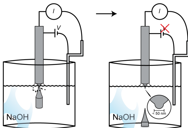
Figure 2.5: Electrochemical etching of a tungsten wire tip. A solid tungsten (W) wire is lowered into a solution of NaOH and adjusted to form a meniscus around the neck of the wire. Negative hydroxide ( \text{OH}^- ) ions react with W to form tungsten oxide ( \text{WO}_4 ). The wire surface is preferentially etched at the meniscus due to increased \text{OH}^- availability, giving rise to a taper in the lower shank. As the neck of the wire shank thins, the weight of the suspended material will cause the lower shank of wire to separate. This event causes a significant drop in the etch current (I) that will trigger a disconnect of the etch voltage (V). High current response rates produce a radius of curvature on the 10–100 nm scale.
