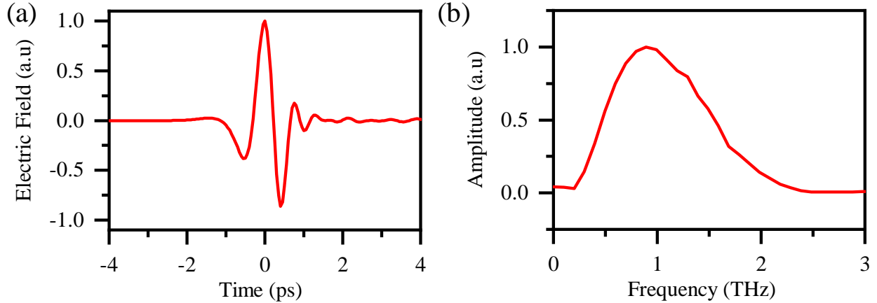
Figure 3.7: Time-domain measurement of a THz electric field transient acquire with EOS. (a) EOS waveform of a THz pulse generated by OR in our 4f setup with \text{LiNbO}_3 . (b) Fast-Fourier transform of the waveform in (a) with bandwidth of 1 THz.
