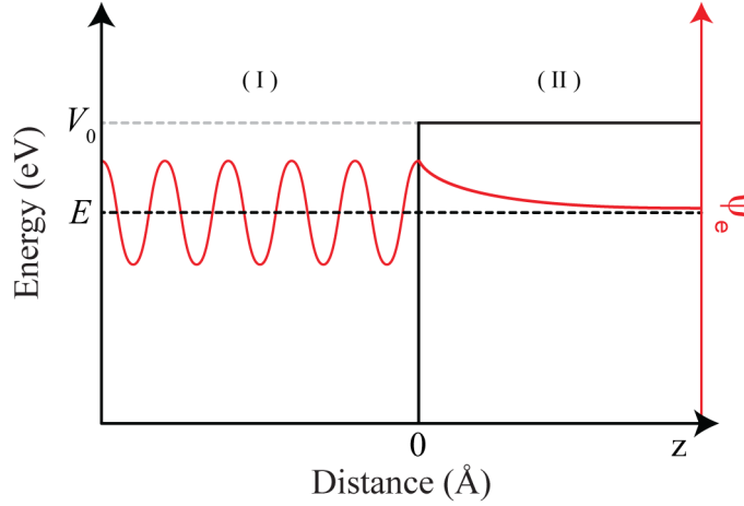
Figure 2.1: Quantum tunneling into a one-dimensional potential V(z) . An electron wavefunction, \psi_e , is represented by a complex plane wave in region (I), where V(z) = 0 , and experiences a real-valued decay within region (II) where V(0) = V_0 .
