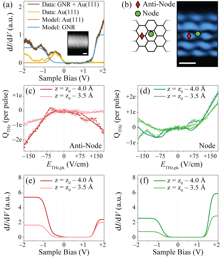
Figure 6.3: THz scanning tunneling spectroscopy of a 7-AGNR with ångström-scale resolution. (a) Conventional STS of a 7-AGNR adsorbed onto an Au(111) surface (solid brown line) and the Au(111) surface state (solid yellow line). The differential conductance of the gold surface state is modeled by a Gaussian centered at -0.4 V (solid orange line), while the differential conductance of the 7-AGNR is modeled as two error functions near the band edges (solid blue line). Inset: typical steady-state constant-height STM image showing the tip positions for tunneling spectroscopy. (b) Tip positions for THz-STs overlaid on a diagram of the physical structure of a 7-AGNR (left) and the Q_{\text{THz}} map from Figure 6.2(g) (right). Diamonds: anti-node position; circles: node position. (c),(d) Measured (circles) and simulated (solid lines) Q_{\text{THz}}-E_{\text{THz,pk}} curves at z = z_0 - 4 Å (dark lines and symbols) and z = z_0 - 3.5 Å (light lines and symbols) with the tip positioned at the anti-node (c) and node (d); V_{\text{DC}} = 0 V. (e),(f) dI/dV extracted from the fits in (c) and (d) for the anti-node (d) and node (f) tip positions, respectively. The dashed lines in (c) – (f) represent the origin. The scalebar in (b) and the inset of (a) are 5 Å.
