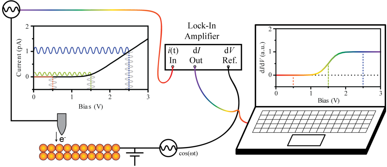
Figure 2.11: Extracting the differential conductance spectrum from the local slope of the I(V) . We trace out the local dI/dV as a function of applied bias ( V ) by recording changes in current, dI , for a bias modulation amplitude of dV . An AC current, i(t) , is induced by an AC bias modulation, V_{AC} = dV \cos(\omega t) , which can be measured using lock-in detection.
