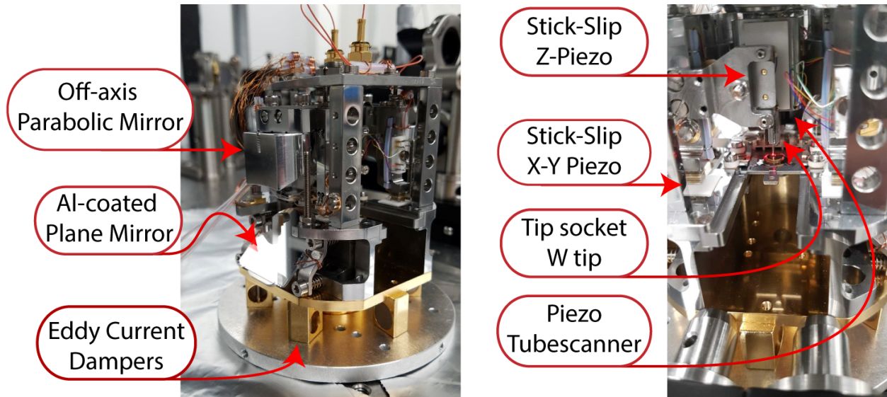
Figure 2.13: Image of the STM scan head with optical elements and pan-scan design.
