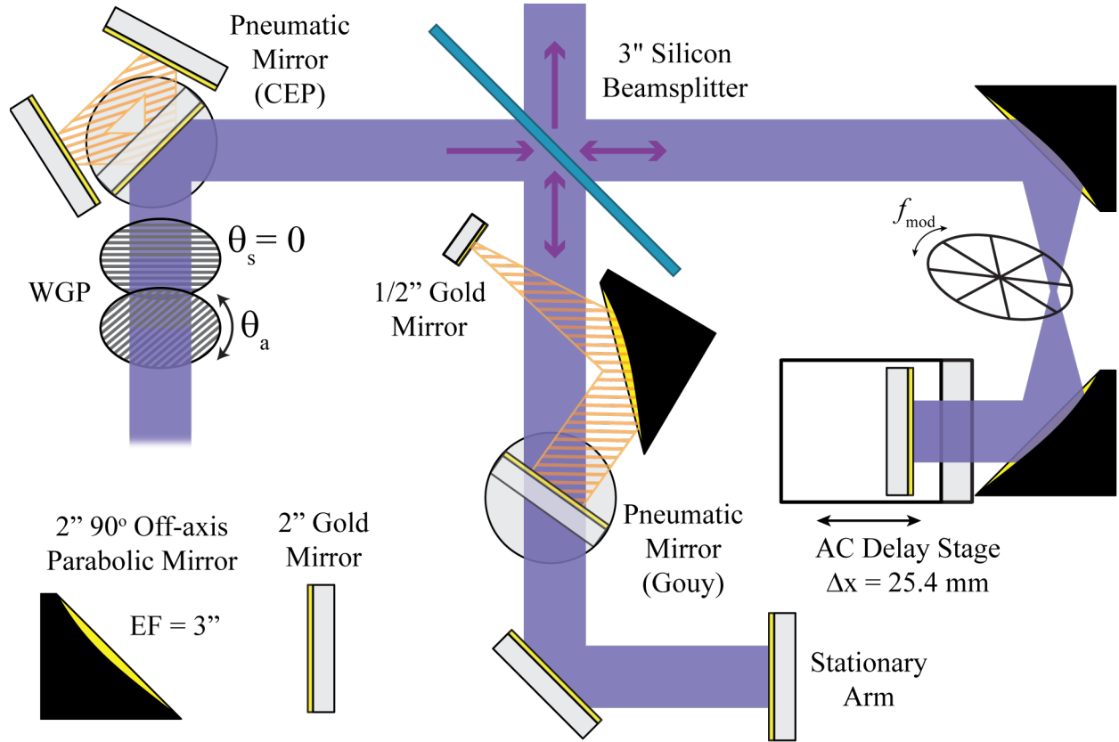
Figure 3.5: THz setup schematic. The THz beam ( E_{\text{THz}} , purple) enters the setup after generation through a pair of wire-grid polarizers (WGP) containing an array of 10\mu\text{m} wires spaced at 30\mu\text{m} . The first WGP controls the THz field strength, |E_{\text{THz}}| \propto \cos^2(\theta_a) with the second WGP statically held at \theta_s = 0^\circ to enforce vertical polarization. A pneumatic flip mirror (CEP) changes the number of reflections in the setup by 1 and alters the carrier-envelop-phase ( \phi_{\text{CEP}} ) by \pi , controlling the polarity of E_{\text{THz}} . A silicon beamsplitter is used to divide the pulse into equal portions and direct them into the two arms of a Michelson-interferometer. The stationary arm has a fixed path length and contains a second pneumatic flip mirror (Gouy) that allows us to change the stationary arm \phi_{\text{CEP}} by \pi using the reflection off of a 0.5-inch gold mirror at the focus of a 90^\circ off-axis parabolic mirror. The adjustable arm contains a delay stage (AC Delay) that controls the path length of the arm and the time-overlap of the two THz pulses. The adjustable arm beam path is equipped with a focus for power measurements or modulation with an optical chopper spinning at frequency f_{\text{mod}} .
