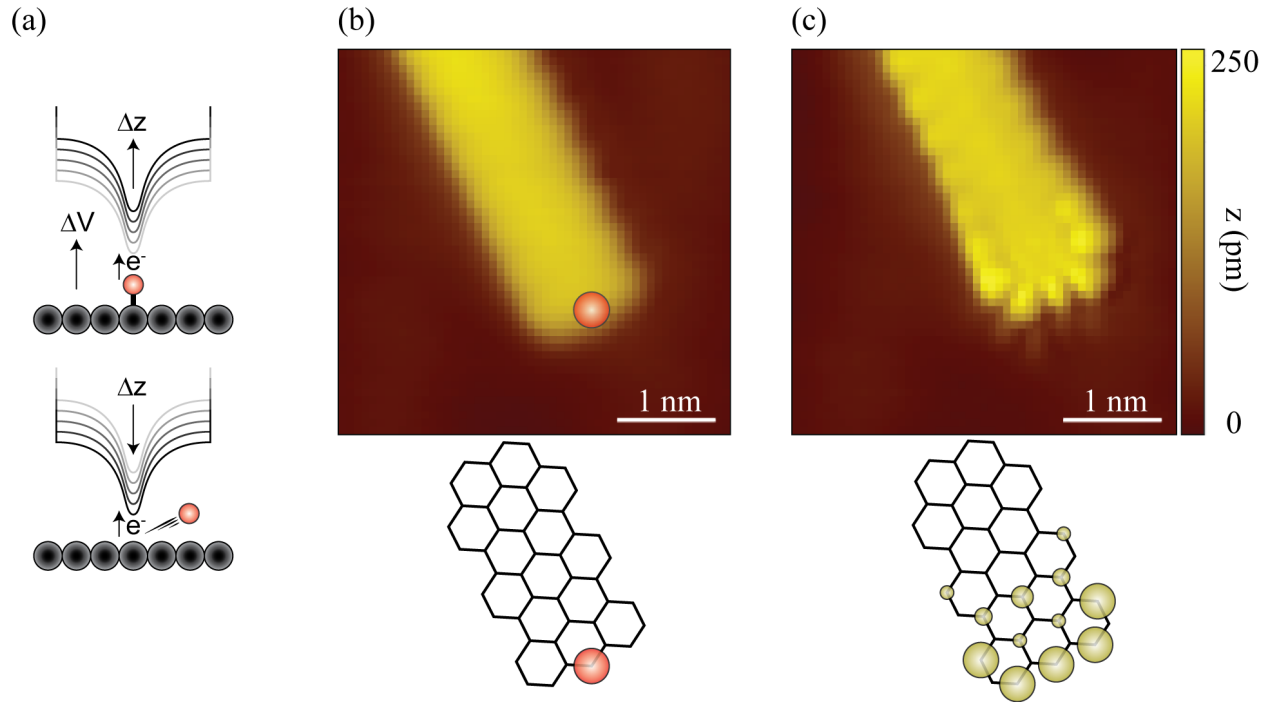
Figure 5.8: 7AGNR modification via dehydrogenation of the ribbon terminus with an STM tip. (a) Cartoon illustration of the tip-induced modification strategy. (b) (top) Topographic image of a 7AGNR exhibiting a featureless termination. (bottom) Carbon structure schematic. The red circle represents the location of the extra hydrogen, bonded to the structure as \text{CH}_2 . (c) (top) Topographic image of the same 7AGNR after tip-induced modification in constant-current operation. (bottom) Carbon structure schematic with yellow circles indicating the location and relative magnitude of the Tamm state exposed after tip-induced modification [224].
