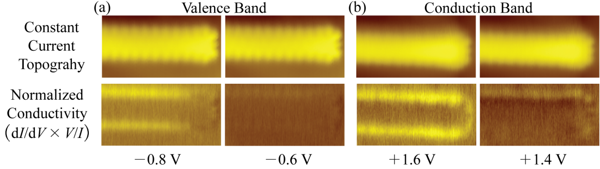
Figure 5.5: Constant-current topography and dI/dV imaging of 7-AGNR frontier bands. (a) Imaging with V_{DC} = -0.8 V, just above the valence band resonance and V_{DC} = -0.6 V, just below the onset. (b) Imaging with V_{DC} = +1.6 V, just above the conduction band resonance and V_{DC} = +1.4 V, just below the onset. dI/dV imaging performed with a bias modulation, V_{mod} = 50 mV measured peak-to-peak. Images acquired with I_{DC} = -50 pA.
