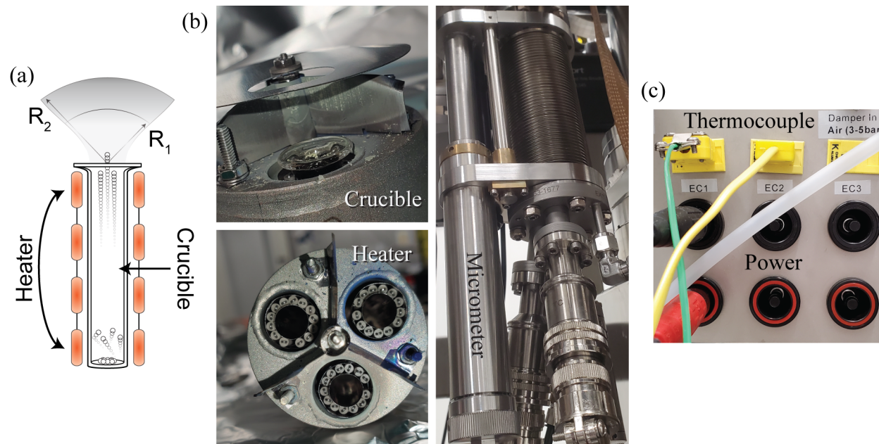
Figure 5.2: (a) Schematic for a Knudsen-type effusion cell, wherein a quartz crucible is heated to evaporate material with a well defined trajectory. (b) In our triple-OLED evaporator, each cell chamber has an individual heater, allowing for isolated evaporation of the material from each crucible. A bellows, equipped with a micrometer, is attached to give control over the radial position of the cell during sample production. (c) Media panel for connecting external power supply and K-type thermocouple. The power supply and thermocouple temperature monitor (green) must be manually moved to whichever cell going to be used.
