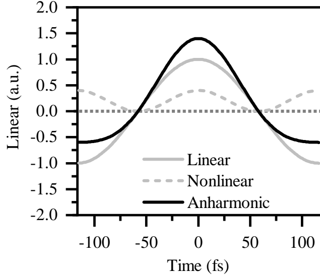
Figure 3.2: One period of an anharmonic oscillation demonstrating the preferential motion in one direction. The anharmonic curve (solid black line) is the sum of linear curve (solid grey line) and the nonlinear curve (dashed grey line).
