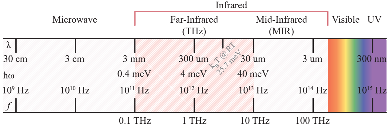
Figure 3.1: Electromagnetic spectrum spanning microwave to visible frequencies. The far-infrared (0.1 - 10 THz) frequency range has become a powerful tool for ultrafast materials science. With photon energies on the order of k_B T at room temperature or below, THz light is non-ionizing and suitable for investigating low-energy and collective excitations in the range of a few meV to several hundred meV.
