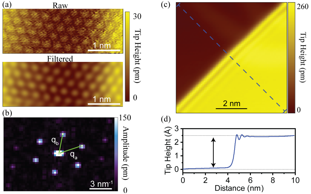
Figure 2.9: Atomic resolution images used to calibrate the STM scanning piezos. (a) Noisy topographic image of an Au(111) surface with atomic resolution (top) and filtered atomic resolution topographic image (bottom). (b) 2D Fast-Fourier transform (FFT) with lattice vectors r_a = 1/q_a = 2.86 \text{ \AA} and r_b = 1/q_b = 2.77 \text{ \AA} . (c) Topographic image of Au(111) terrace edge, including oscillations due to scattering of electrons in the surface state are visible at the step edge. (d) Line cut along the blue dashed line in (c) indicating a step height of 2.5 \text{\AA} . The filtered image in (a) is the result of isolating the Bragg peaks in the FFT of (b). Topographic images acquired in constant-current mode with setpoints (a) V_{\text{DC}} = -6 \text{ mV} and I_{\text{DC}} = -50 \text{ pA} at T_{\text{sample}} = 78\text{K} and (c) V_{\text{DC}} = -400 \text{ mV} and I_{\text{DC}} = -300 \text{ pA} at T_{\text{sample}} = 7\text{K}
