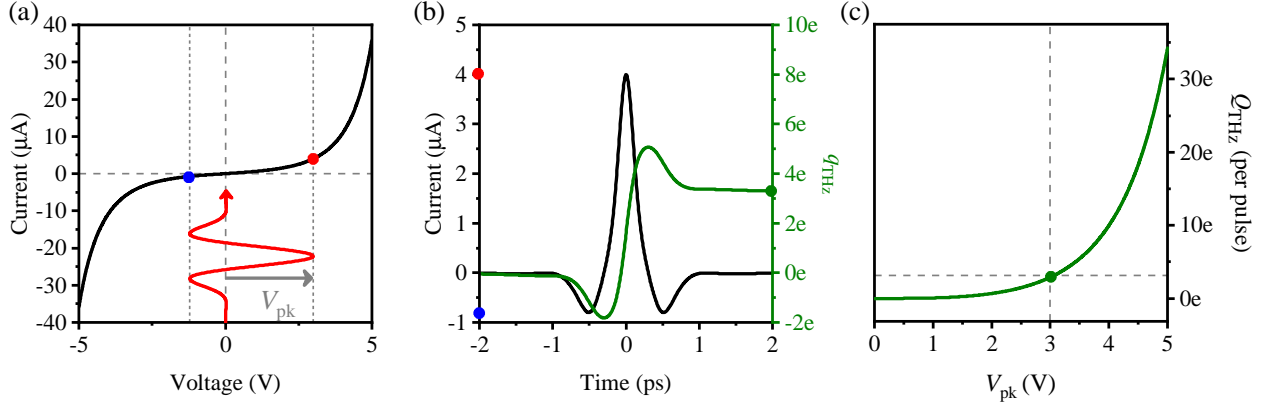
Figure 4.8: Terahertz-induced charge rectification across an STM tunnel junction. (a) Simmons model I(V) (black curve) for a typical THz-STM tip height of z = 4 \text{ \AA} . In THz-STM, a transient voltage pulse V_{\text{THz}}(t) (represented schematically by red curve) acts on the I(V) characteristic. Here, V_{\text{THz}}(t) is defined as a normalized oscillatory component multiplied by V_{\text{pk}} . The maximum and minimum voltages sampled by the voltage pulse are indicated by solid red and blue circles, respectively. (b) Ultrafast current pulse (black curve) generated by mapping the transient bias voltage onto the I-V characteristic in (a). Red and blue points indicate the extrema, as in (a). The green curve shows the running integral of the current transient, defined in the text as q_{\text{THz}} . The green point denotes the net rectified charge per pulse, defined in the text as Q_{\text{THz}} , which is detected in a THz-STM experiment. (c) The simplest spectroscopic measurement for THz-induced tunneling is to sweep V_{\text{pk}} and measure Q_{\text{THz}} .
