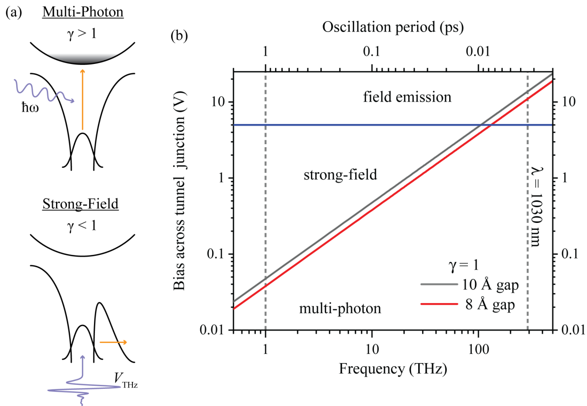
Figure 4.2: Illustration and calculation of the Keldysh parameter, \gamma , defining the separation between two regimes of nonlinear light-matter interaction, i.e., the multi-photon and strong-field regimes. (a) An illustration of the differences between multi-photon and strong-field regimes. In the multi-photon regime ( \gamma > 1 ) the system undergoes an electronic excitation by absorbing a photon with energy, \hbar\omega , resulting in a direct excitation into higher energy bands (top). In the strong-field regime ( \gamma < 1 ) the electric field of the light acts as a voltage, e.g., V_{\text{THz}} , and changes the potential of the system (bottom). Distortion of the energy landscape changes the height of the potential barriers and allows for quantum tunneling. (b) Calculation of applied voltage across an STM tunnel junction for typical gap distances. The region above the diagonal line corresponds to the strong-field regime, while the region below the line corresponds to the multi-photon regime. The blue horizontal line indicates the applied voltage at which field emission occurs for a static bias and \Phi = 5 \text{ eV} . A pair of vertical dashed grey lines are provided for reference, denoting the approximate center frequency of our THz pulses (left) and the fundamental frequency of our NIR laser system (right).
