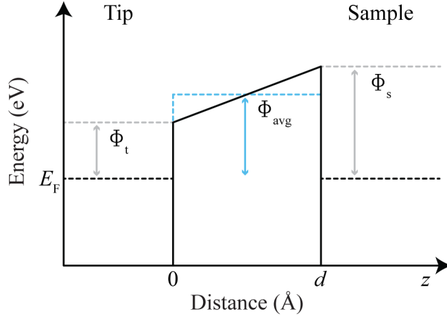
Figure 2.3: Trapezoidal potential barrier diagram. The tip material (left) is characterized by a work function, \Phi_t , which is the difference between the Fermi energy, E_F , and the top of the potential barrier at z = 0 . The sample material (right) is characterized by a work function \Phi_s . Notably, the difference between \Phi_t and \Phi_s produces a trapezoidal barrier that can be approximated by a rectangular barrier of height \Phi_{\text{avg}} = (\Phi_t + \Phi_s)/2 . The differences in height can arise from a combination of material and geometrical differences.
