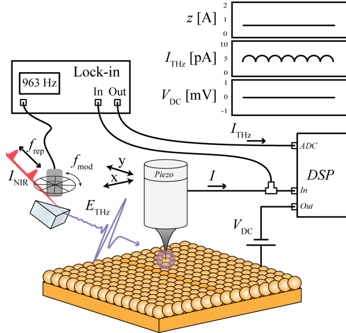
Figure 4.1: Schematic diagram of constant-height THz-STM operation. NIR pulses ( I_{\text{NIR}} ) generate single-cycle THz pulses ( E_{\text{THz}} ) that illuminates the tunnel junction of an STM and induces a tunnel current at a repetition rate, f_{\text{rep}} = 1 MHz. The STM tunnel current is fed into a lock-in amplifier that is referenced to an optical chopper, which modulates the NIR pulse train. This turns the THz generation on and off at a modulation rate, f_{\text{mod}} = 963 Hz. The lock-in signal is fed into the DSP, where the THz-induced current is recorded. Constant-height THz-STM operates without the feedback loop engaged and typically with V_{\text{DC}} = 0 V.
