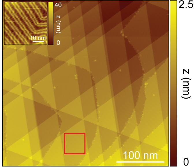
Figure 2.8: Constant-current topography image of a clean, atomically smooth, Au(111) surface. The herringbone surface reconstruction of the (111) crystal orientation is visible in the inset (red box). Preparation of the sample surface was done through cycles of sputtering with 1 keV Ar ions and annealing to 900 K. Imaging conditions: I_{\text{DC}} = -50 pA and V_{\text{DC}} = -2.0 V.
