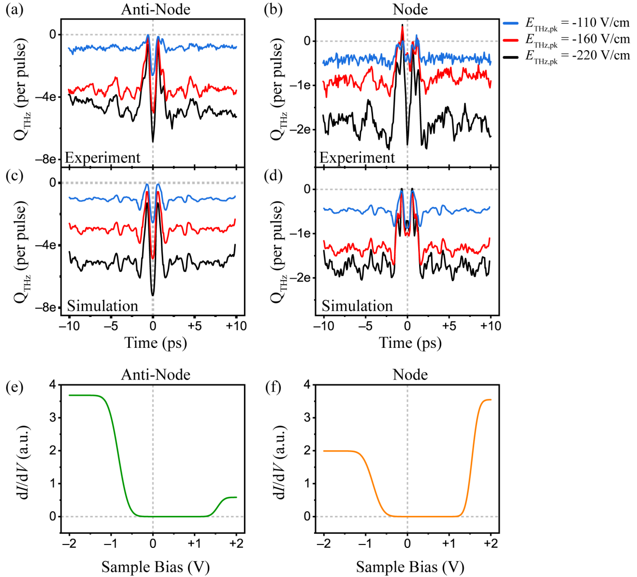
Figure 6.6: THz-STM autocorrelations of a 7-AGNR on Au(111). (a),(b) Experimental THz pulse autocorrelations acquired at zero DC bias ( V_{\text{DC}} = 0 V) and at constant height ( z = z_0 - 4 \text{ \AA} ) with the tip positioned at the anti-node (a) and node (b). (c),(d) Simulated THz pulse autocorrelations for the the anti-node (c) and node (d) tip positions using the PES waveform in Figure 6.2(e)/(f). The nonlinearity of the I(V) that rectifies the THz pulse within the model was determined from the t = 0 ps and t = 10 ps values of the experimental autocorrelations. (e),(f) Model dI/dV for the anti-node (e) and node (f) tip positions.
