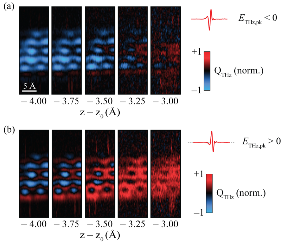
Figure 6.10: Variable-height THz-STM of a 7-AGNR on Au(111). (a),(b) THz-STM imaging tip-height dependence, Q_{\text{THz}}(x, y) vs. z , i.e., THz-driven scanning tunneling tomography, acquired at E_{\text{THz,pk}} = -180 V/cm (a) and E_{\text{THz,pk}} = +180 V/cm (b) with V_{\text{DC}} = 0 V. The scalebar in (a) applies to both (a) and (b).
