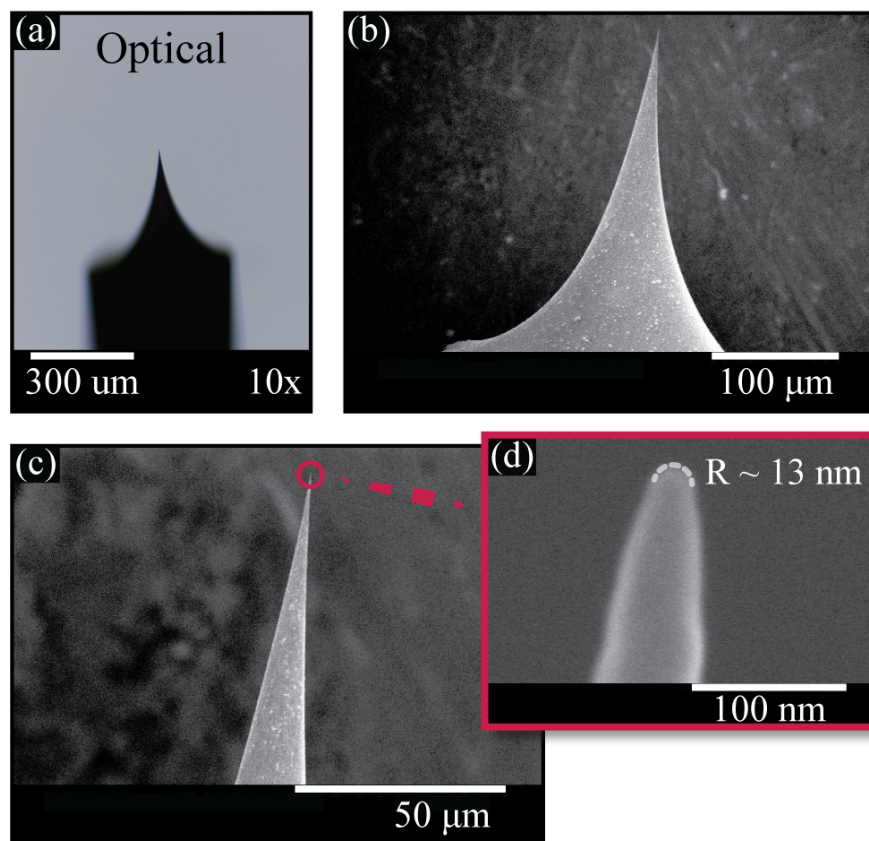
Figure 2.6: An example of a successful electrochemical etching of a tungsten wire tip. (a) Optical microscope image at 10x magnification. A single cusp feature formed by the ‘drop-off’ mechanism is present, providing a smooth taper on the scale of 300\ \mu\text{m} . (b), (c), and (d) Scanning electron microscope images of the same tungsten tip with increasing magnification. The SEM images indicate a radius of curvature of \sim 13\ \text{nm} .
