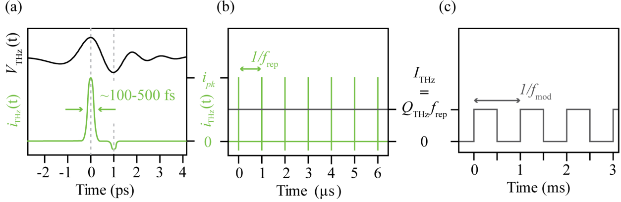
Figure 4.5: Measuring a THz-STM signal with lock-in detection. (a) An ultrafast voltage transient, V_{\text{THz}}(t) , induces a sub-picosecond current pulse, i_{\text{THz}}(t) . (b) A train of current pulses are generated at the laser repetition rate, f_{\text{rep}} , leading to a current detected by the STM that is proportional to the net charge rectified per pulse, Q_{\text{THz}} . (c) Using lock-in detection and modulating the THz pulse train at a rate, f_{\text{mod}} , the average THz-induced current, I_{\text{THz}} , is measured.
