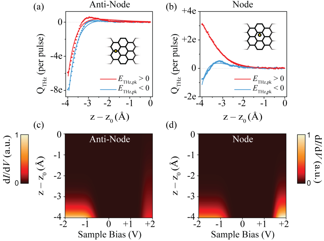
Figure 6.8: Tip-height-dependent THz-STM of a 7-AGNR on Au(111). (a),(b) Measured (circles) and simulated (solid lines) tip retraction scans at the anti-node (a) and node (b) positions (see inset) acquired at V_{DC} = 0 V, E_{THz,pk} = -180 V/cm (blue) and E_{THz,pk} = +180 V/cm (red). (c),(d) Differential conductance at the anti-node (c) and node (d) spatial positions for tip heights, z , ranging from z_0 to z_0 - 4 Å extracted from the fits in (a) and (b), respectively. The orbital decays are modeled using the expression \exp(-2\kappa z) . Negative bias fit parameters: \kappa = 1.3 Å -1 at the anti-node and \kappa = 1.2 Å -1 at the node. Positive bias fit parameters: \kappa = 0.4 Å -1 at the anti-node and \kappa = 0.9 Å -1 at the node.
