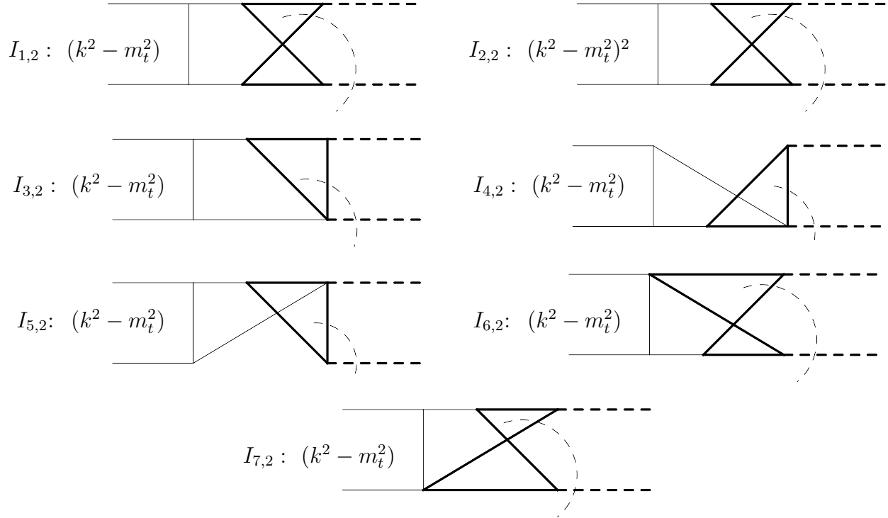
Figure 4.2.4: Integrals appearing in the linear combination in Eq. 4.2.21. I_{1,2} is the corner integral of the topology under consideration but with a numerator (k^2 - m_t^2) , identical to I_{2,1} from Eq. 4.2.20. I_{2,2} is I_{1,2} but with an extra numerator (k^2 - m_t^2) where k is equal to the difference of the momenta of the edges marked by the thin dashed lines. Integrals I_{3,2}, I_{4,2}, I_{5,2}, I_{6,2}, I_{7,2} are the same as I_{3,1}, I_{4,1}, I_{5,1}, I_{6,1}, I_{7,1} but with an extra numerator (k^2 - m_t^2) . All integrals are defined in d = 4 - 2\epsilon dimensions. Reproduced from [6].
