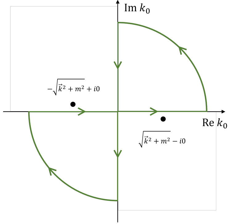
Figure B.1: The integration contour to perform Wick rotation. Note that the poles lie outside the contour.
