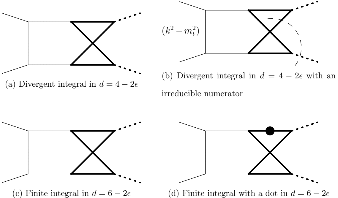
Figure 4.2.2: Examples of divergent and finite integrals in the limit \epsilon \rightarrow 0 for a non-planar topology. Thick solid lines represent the top-quark while thick dashed lines represent Z-bosons. Topology (b) contains an irreducible numerator, where k is the difference of the momenta of the edges marked by the thin dash lines. Reproduced from [6].
