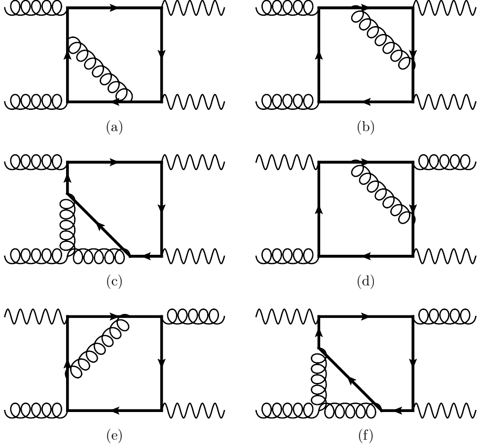
Figure 2.3.3: Representative Feynman diagrams in class A with reducible topologies.
