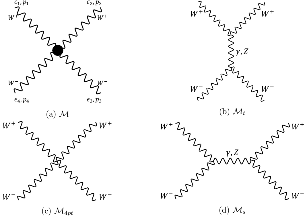
Figure 1.2.1: WW scattering with the 3 different subprocesses depicted.
