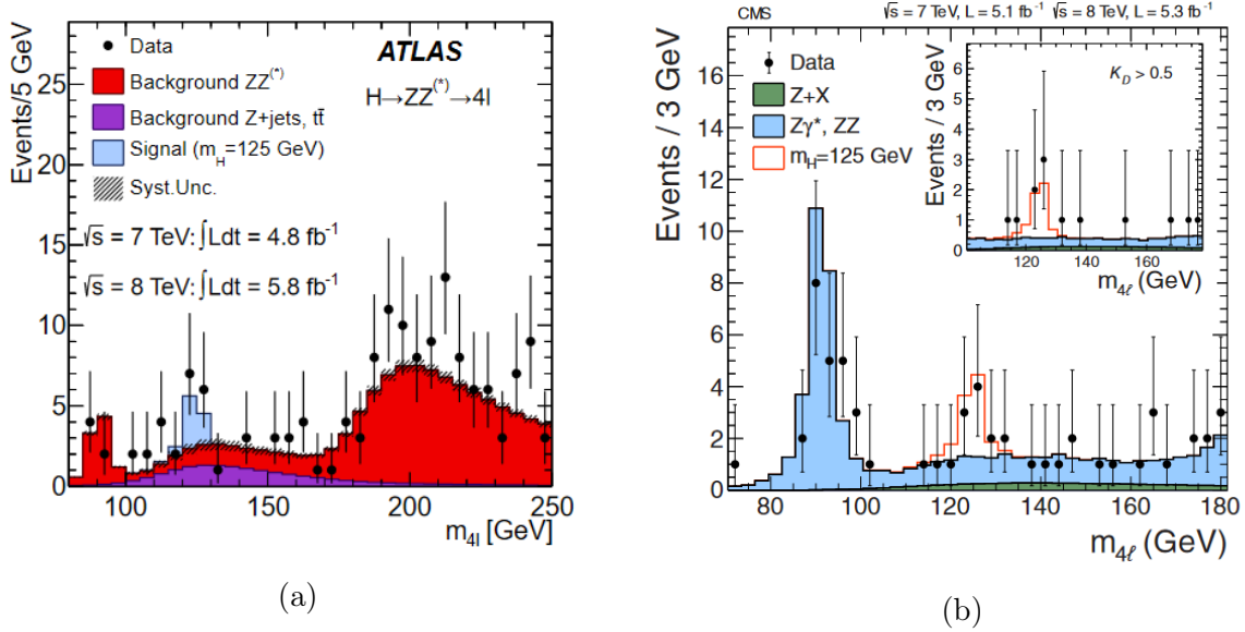
Figure 1.2.5: Distribution of four lepton invariant mass for the h \rightarrow ZZ^* \rightarrow l^+l^-l^+l^- decay channel for (a) ATLAS (Reproduced from [8]) and (b) CMS (Reproduced from [9]) experiments.
