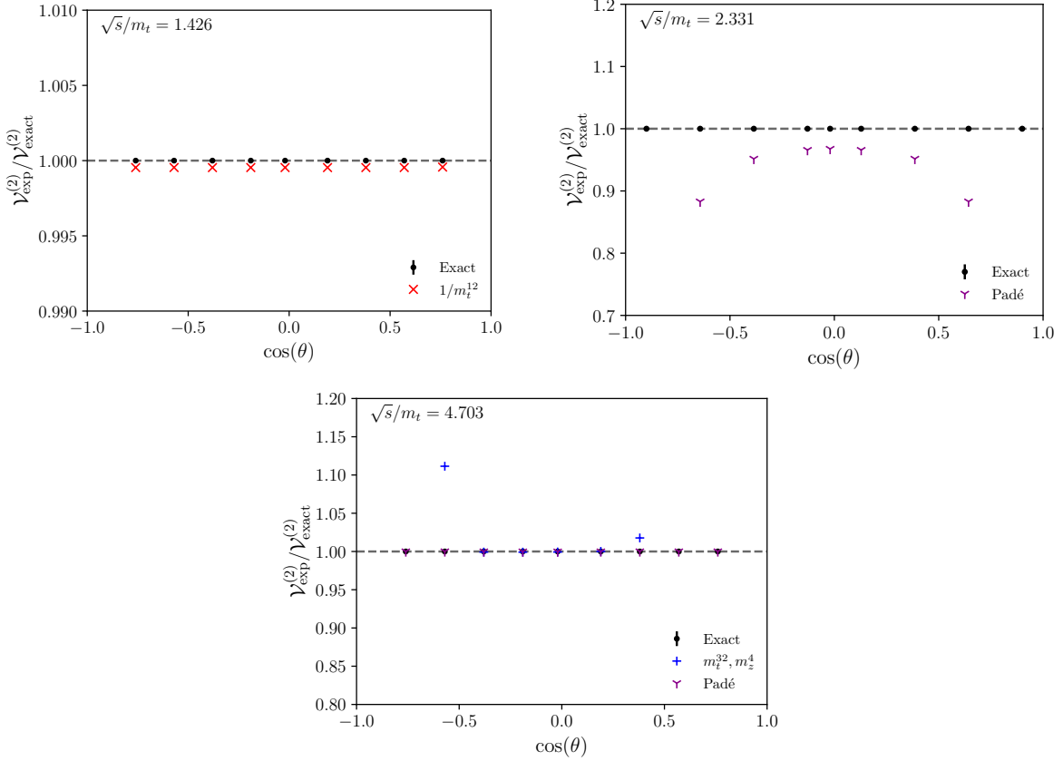
Figure 6.1.2: Comparison of the \cos(\theta) dependence of the unpolarised interference \mathcal{V}^{(2)} with the results expanded in the limit of large top-quark mass for \sqrt{s} = 247 GeV (Top Left Panel) and small top-quark mass for \sqrt{s} = 403 GeV (Top Right Panel) and \sqrt{s} = 814 GeV (Bottom Panel). Reproduced from [6].
