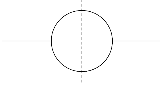
Figure 3.2.1: A two-point function with massless propagators. The dashed line corresponds to the cut propagators.
