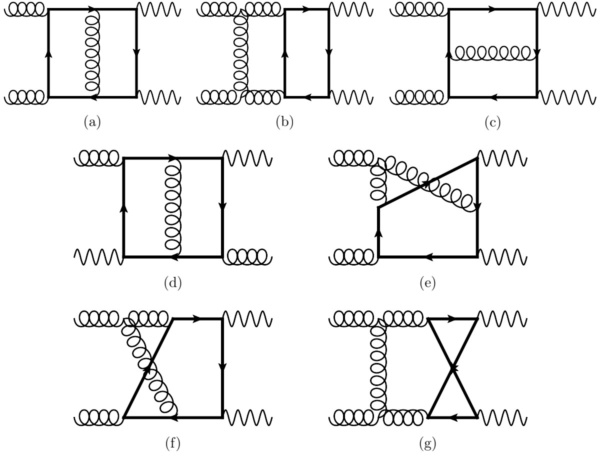
Figure 2.3.2: Representative Feynman diagrams in class A with irreducible topologies. The number of master integrals in each topology are 3, 4, 3, 3, 5, 5, and 4 respectively
