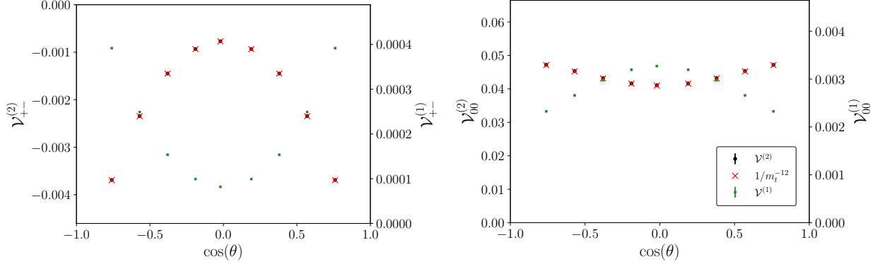
Figure 6.1.8: The \cos(\theta) dependence of 1-loop and 2-loop interferences for polarised ZZ production in gluon fusion at \sqrt{s}/m_t = 1.426 . The large top-quark mass expansion [12] (to order 1/m_t^{12} ) is shown for comparison. Here, the top left and bottom right panels of Fig. 6.1.4 are reproduced using Catani’s original subtraction scheme [13]. Reproduced from [6].
