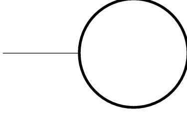
Figure 3.1.1: A tadpole graph with the thick loop corresponding to the massive propagator with mass m .
