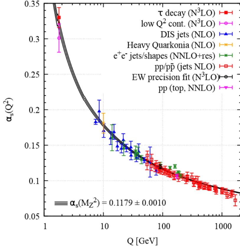
Figure 1.4.7: Plot showing theoretical prediction for the strong coupling \alpha_S against experimental measurements. Reproduced from [1].
