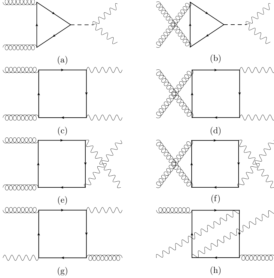
Figure 2.2.1: Feynman diagrams for the process gg \rightarrow ZZ at 1-loop (LO). 2.2.1a and 2.2.1b are the Higgs exchange diagrams.
