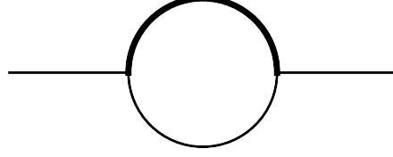
Figure 3.1.2: A two-point function with one massive propagator. The thick line corresponds to the massive propagator.
