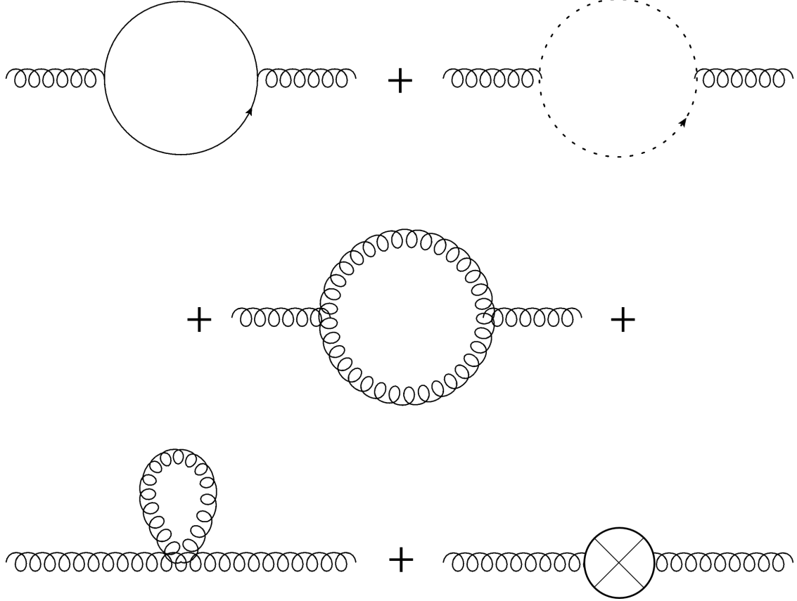
Figure D.1: All the diagrams contributing to 1-loop correction to the gluon propagator, including the counterterm diagram. Requiring that the sum is finite allows the calculation of the counterterm \delta_G .
