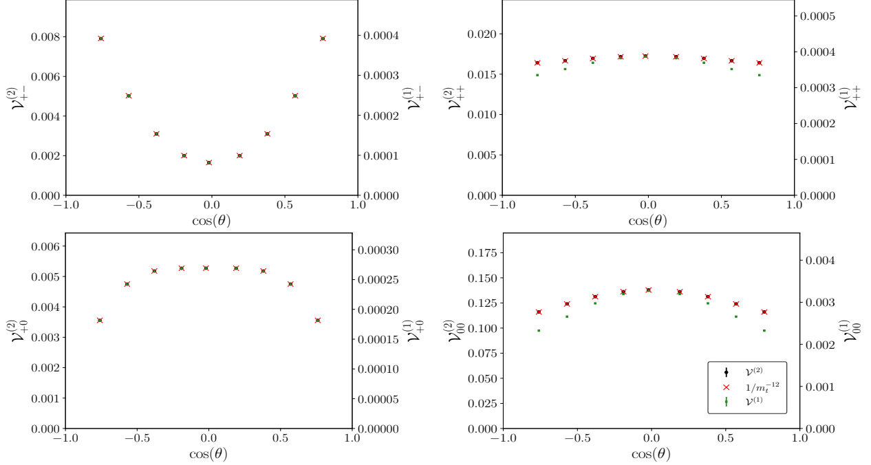
Figure 6.1.4: The \cos(\theta) dependence of 1-loop and 2-loop interferences for polarised ZZ production in gluon fusion at \sqrt{s}/m_t = 1.426 . The large top-quark mass expansion [12] (to order 1/m_t^{12} ) is shown for comparison. Reproduced from [6].
