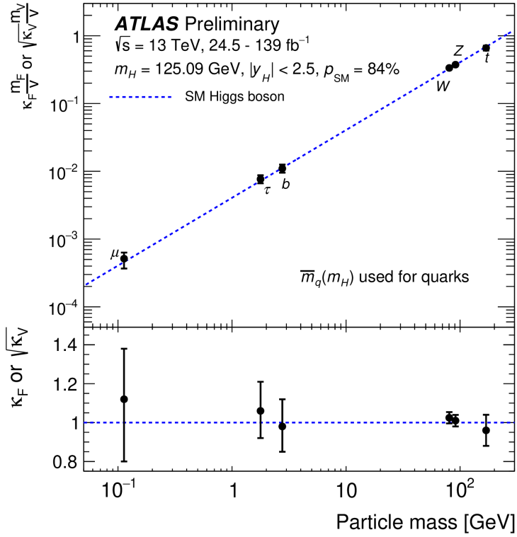
Figure 1.2.7: Plot of the measured Higgs boson couplings to other Standard Model particles against particle mass. Reproduced from [10].
