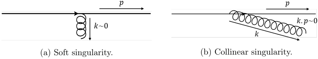
Figure 1.4.5: Infrared divergences corresponding to the emission of a real particle. Fig. 1.4.5a shows emission of a gluon with very small momentum i.e. a soft divergence while Fig. 1.4.5b shows the emission of a gluon collinear with the external particle.
