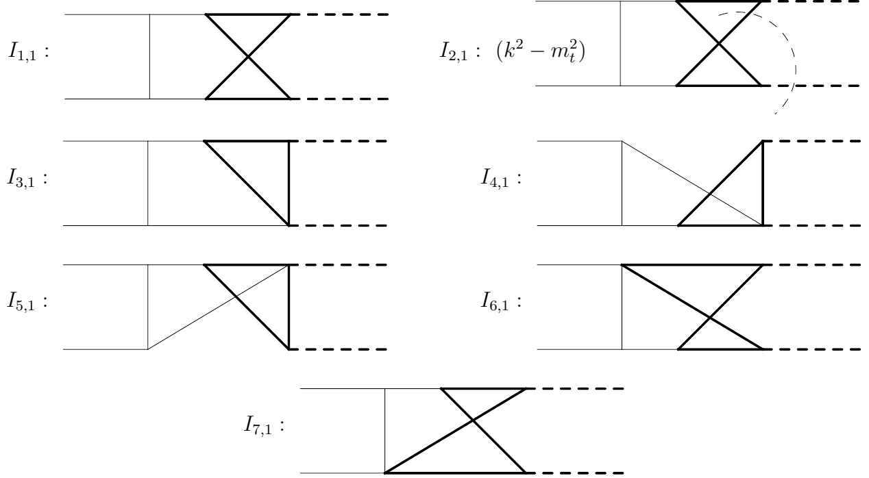
Figure 4.2.3: Integrals appearing in the linear combination in Eq. 4.2.20. I_{1,1} is the corner integral of the topology under consideration. I_{2,1} is a second integral in the topology, but with a numerator (k^2 - m_t^2) , where k is equal to the difference of the momenta of the edges marked by the thin dashed lines. Integrals I_{3,1}, I_{4,1}, I_{5,1}, I_{6,1}, I_{7,1} belong to subtopologies. All integrals are defined in d = 4 - 2\epsilon dimensions. Reproduced from [6].
