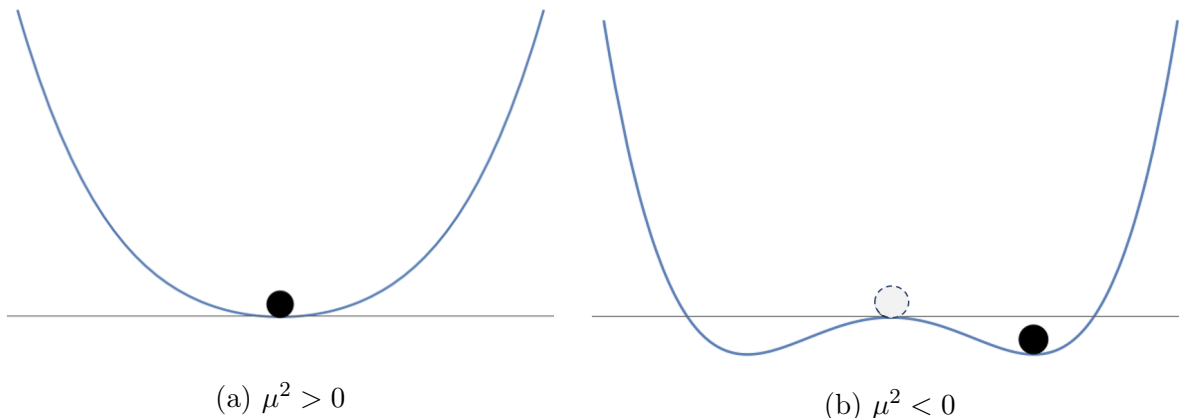
Figure 1.2.2: Scalar field \Phi with two different vacuum configurations. For \mu^2 < 0 the vacuum state is no longer symmetric and the field acquires a non-zero expectation value.
