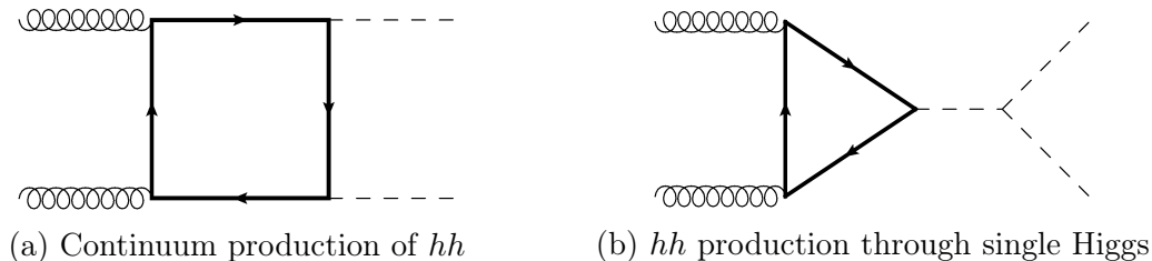
Figure 1.3.1: Higgs pair production through gluon fusion at LO.
