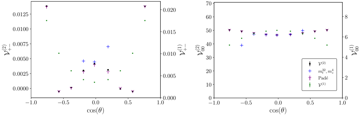
Figure 6.1.10: The \cos(\theta) dependence of 1-loop and 2-loop interferences for polarised ZZ production in gluon fusion at \sqrt{s}/m_t = 4.703 . The small top-quark mass expansion (to order m_t^{32} ) and Padé improved expansion [12] are shown for comparison. Here, the top left and bottom right panels of Fig. 6.1.6 are reproduced using Catani's original subtraction scheme [13]. Reproduced from [6].
