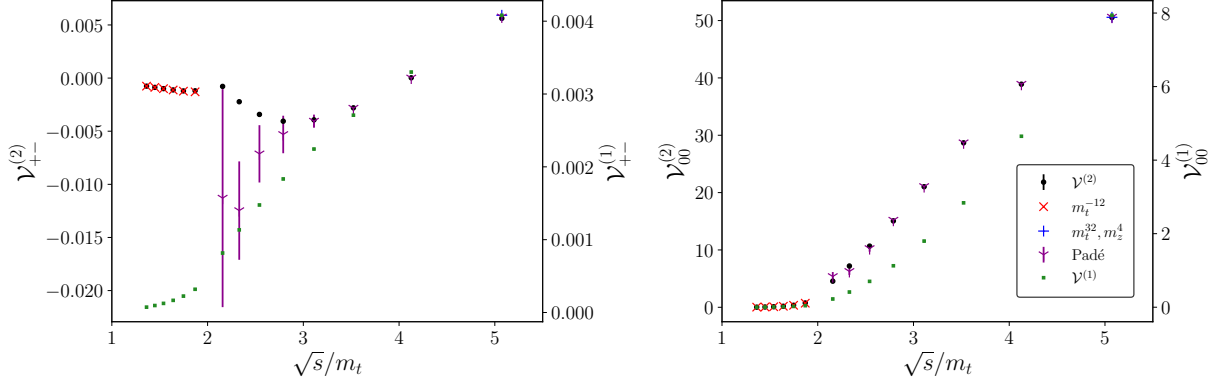
Figure 6.1.7: The \sqrt{s} dependence of 1-loop and 2-loop interferences for polarised ZZ production in gluon fusion at \cos(\theta) = -0.1286 . Here, the top left and bottom right panels of Fig. 6.1.3 are reproduced using Catani’s original subtraction scheme [13]. Reproduced from [6].
