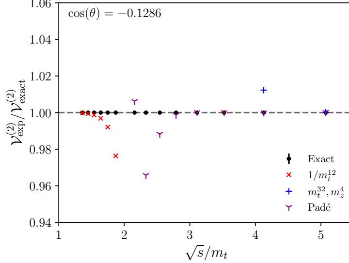
Figure 6.1.1: Comparison of the \sqrt{s} dependence of the unpolarised interference \mathcal{V}^{(2)} with expansion for large and small top-quark mass [12] at fixed \cos(\theta) = -0.1286 . The large top-mass expansion is shown in colour red, the small top-mass expansion in blue, and the Padé improved small top-mass expansion in purple. The exact result is shown in black. Note that the error bars have been plotted for the exact result, they are too small to be visible on the plot, however. Reproduced from [6].
