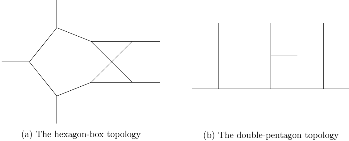
Figure 3.5.1: The non-planar topologies for 5-point 2-loop \gamma\gamma + \text{jet} production.
