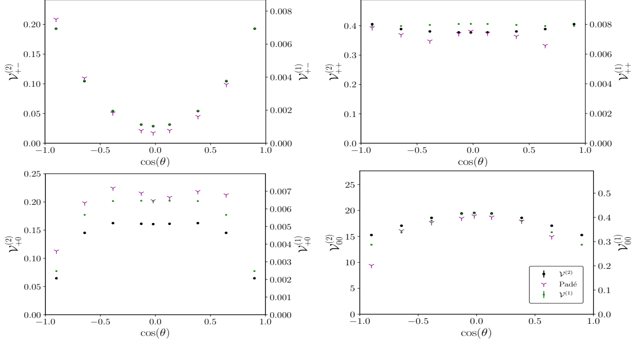
Figure 6.1.5: The \cos(\theta) dependence of 1-loop and 2-loop interferences for polarised ZZ production in gluon fusion at \sqrt{s}/m_t = 2.331 . The Padé improved small top-quark mass expansion [12] is shown for comparison. Reproduced from [6].
