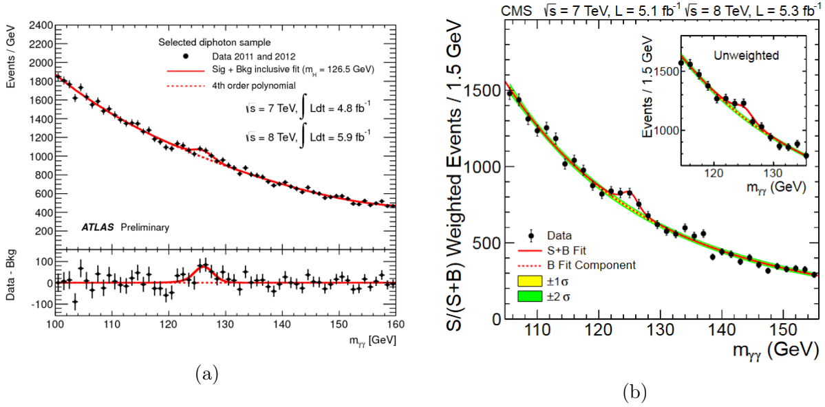
Figure 1.2.6: Distribution of the invariant mass of the photon pair for the h \rightarrow \gamma\gamma decay channel for (a) ATLAS (Reproduced from [8]) and (b) CMS (Reproduced from [9]) experiments.
