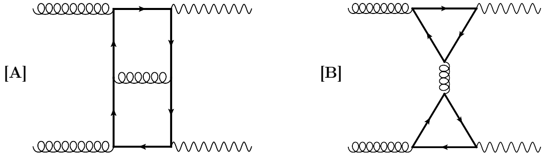
Figure 2.3.1: Example Feynman diagrams representing the two classes of diagrams at 2-loops
