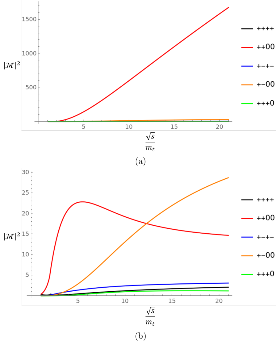
Figure 2.2.4: Comparison of |\mathcal{M}|^2 for different helicities for the top quark contribution including the Higgs diagrams.
