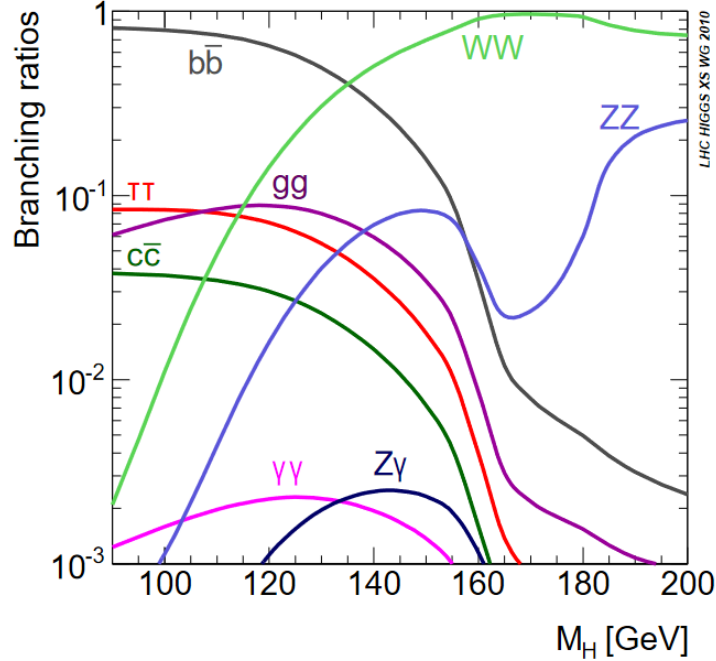
Figure 1.2.4: Plot of the Standard Model Higgs branching ratios against the Higgs mass. Measured value of Higgs mass is m_h = 125.25 \pm 0.17 GeV. Reproduced from [7].
