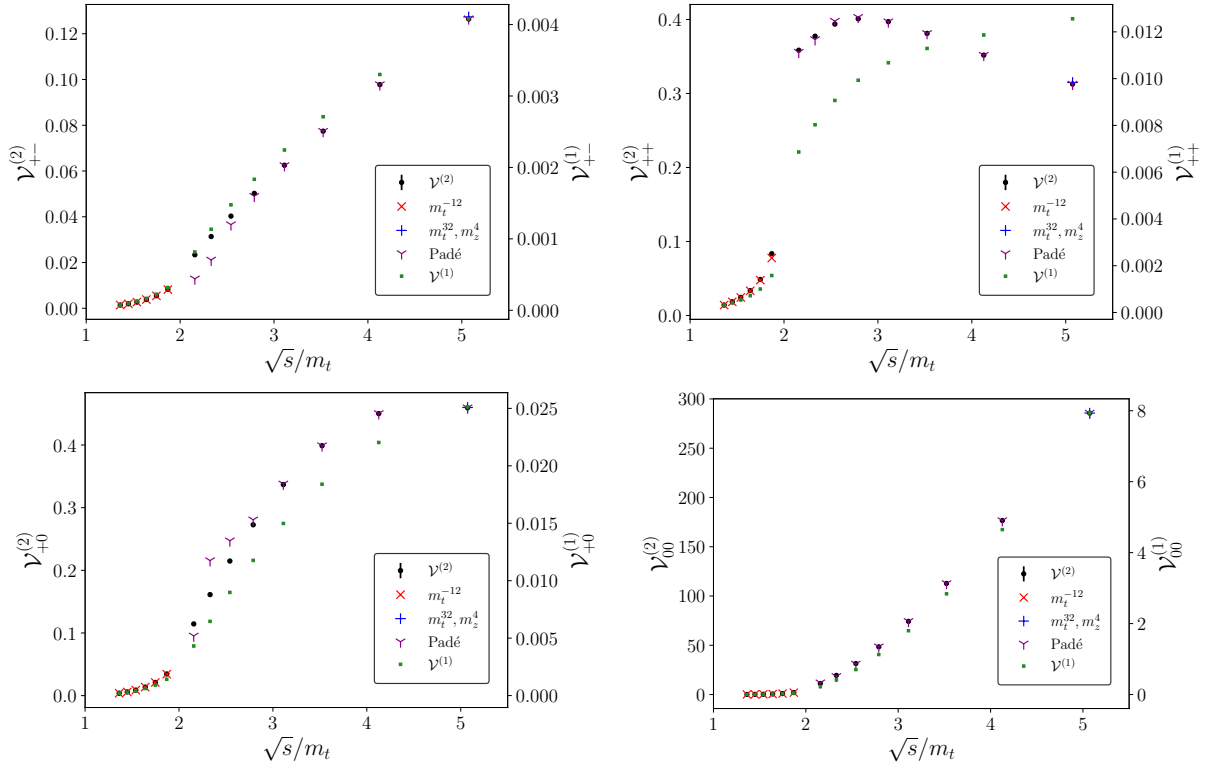
Figure 6.1.3: The \sqrt{s} dependence of 1-loop and 2-loop interferences for polarised ZZ production in gluon fusion at \cos(\theta) = -0.1286 . Reproduced from [6].
