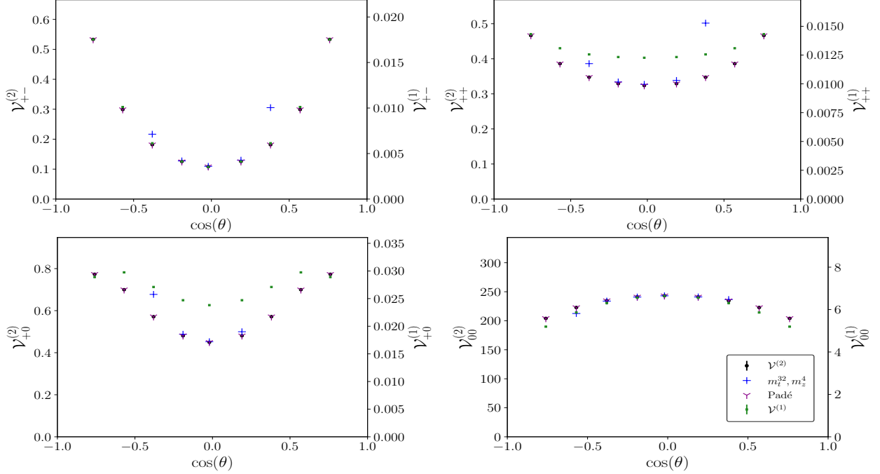
Figure 6.1.6: The \cos(\theta) dependence of 1-loop and 2-loop interferences for polarised ZZ production in gluon fusion at \sqrt{s}/m_t = 4.703 . The small top-quark mass expansion (to order m_t^{32} ) and Padé improved expansion [12] are shown for comparison. Reproduced from [6].
