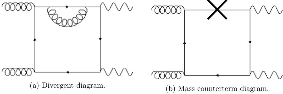
Figure 5.2.1: Mass counterterm diagrams required at 2-loops. The big dark cross in Fig. 5.2.1b corresponds to the counterterm vertex insertion.
