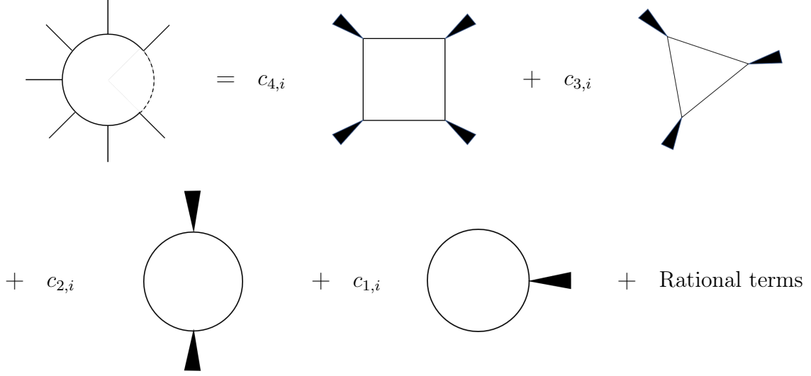
Figure 2.2.2: Decomposition of a general 1-loop Feynman integral
