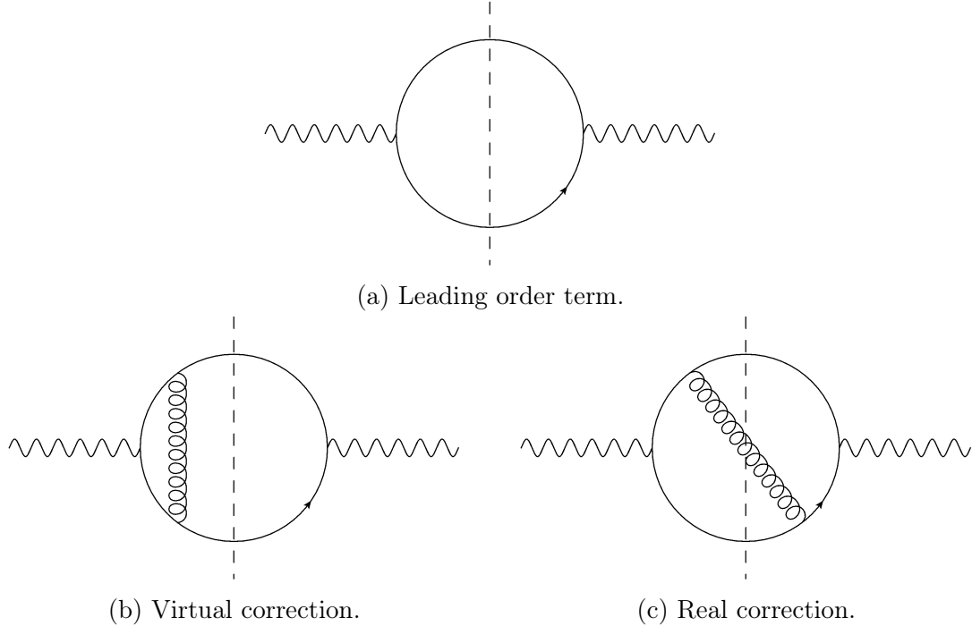
Figure 1.4.6: QCD corrections to q\bar{q} \rightarrow \gamma . Fig. 1.4.6b shows the \alpha_S correction through the exchange of a virtual gluon while Fig. 1.4.6c show the \alpha_S correction through the emission of a real gluon.
