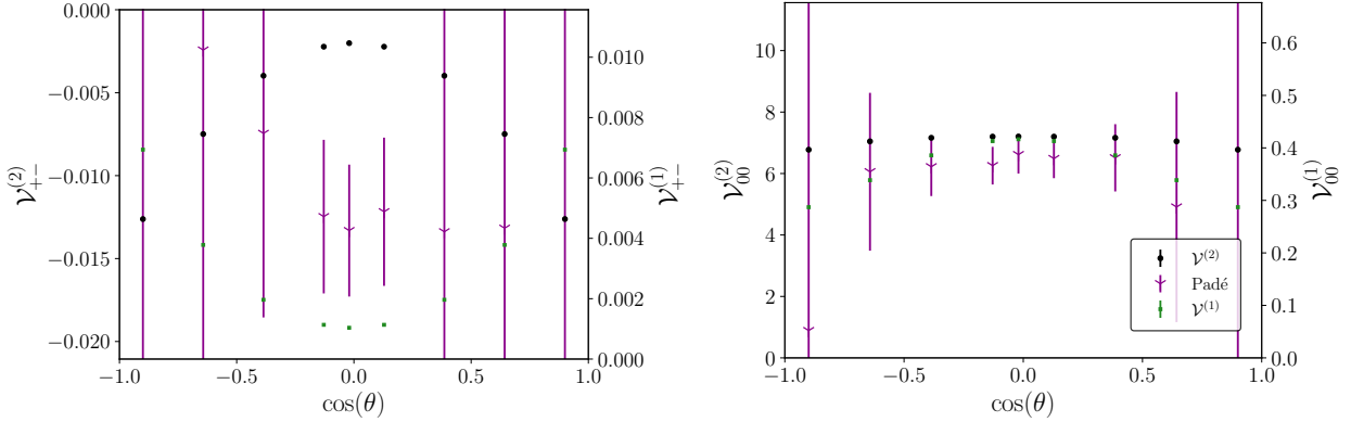
Figure 6.1.9: The \cos(\theta) dependence of 1-loop and 2-loop interferences for polarised ZZ production in gluon fusion at \sqrt{s}/m_t = 2.331 . The Padé improved small top-quark mass expansion [12] is shown for comparison. Here, the top left and bottom right panels of Fig. 6.1.5 are reproduced using Catani’s original subtraction scheme [13]. Reproduced from [6].
